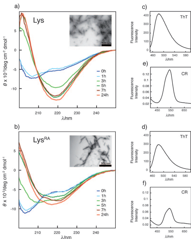
Figure 2. Aggregation kinetics of a) Lys at pH 2.0 and 60 °C and b) Lys RA at pH 2 and 20 °C monitored by far UV-CD. Samples of fibrils formed after 24 h and isolated by ultracentrifugation have a fibrillar morphology (insets in (a) and (b)) and bind ThT (c, d) and CR (e, f). In the presence of the fibrils the ThT fluorescence maximum is ca. 485 nm, and the CR absorbance maximum is ca. 540 nm, which is typical of the amyloid structure (see the Supporting Information).
