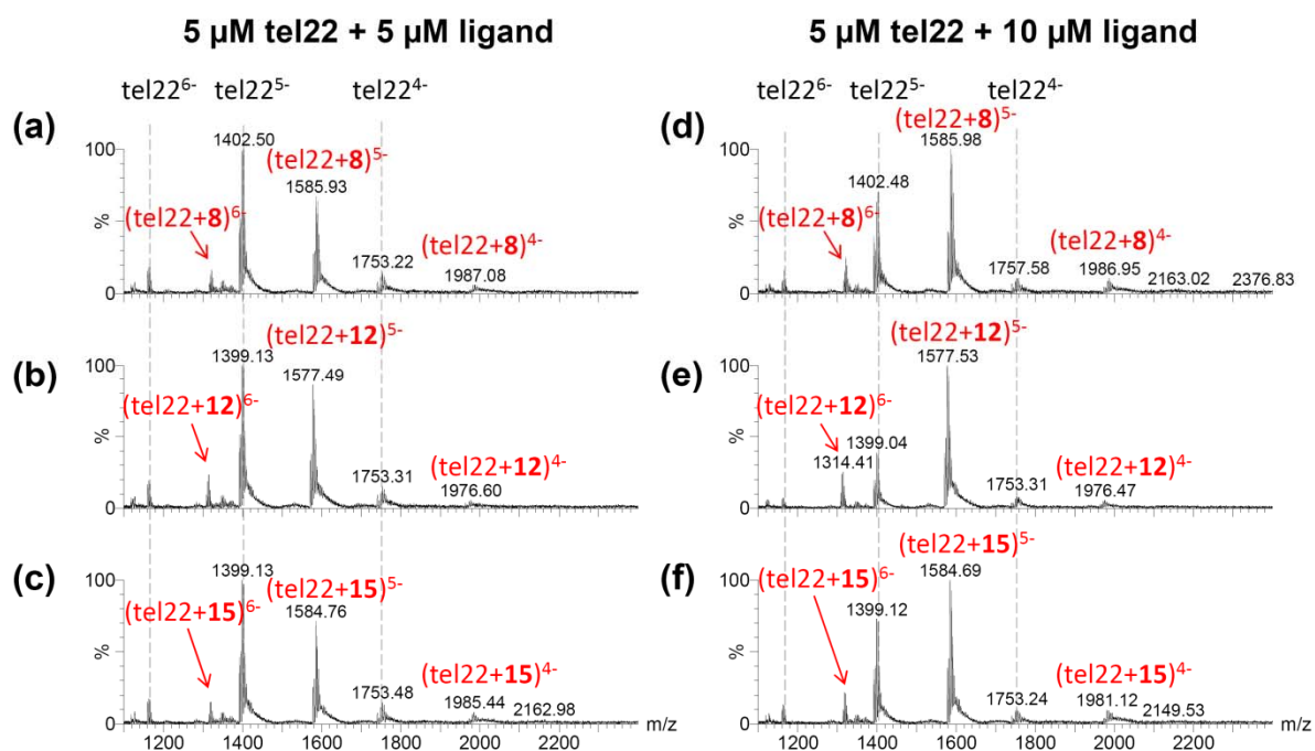
Figure S1: Representative ESI-MS spectra of mixtures between 5 \mu\text{M} telomeric G-quadruplex dAGGG(TTAGGG) 3 (tel22) and 5 \mu\text{M} ligand 8 (a), 12 (b), 15 (c), or 10 \mu\text{M} of the same ligand (d-f). The free tel22 and the complexes were detected at charge states 6- to 4-. The most intense charge state (5-) was used for determining the K_d 's.
