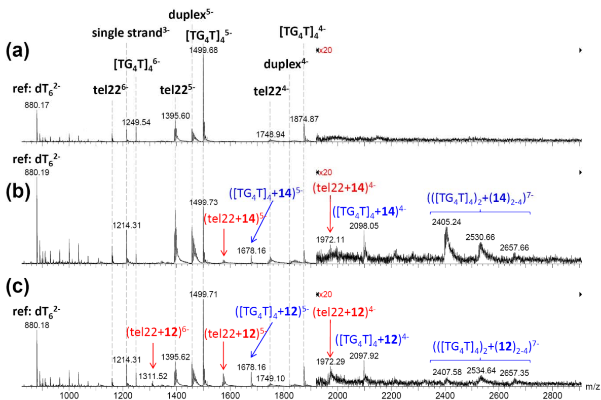
Figure S2: Competition experiment between the telomeric G-quadruplex dAGGG(TTAGGG) 3 (tel22), the duplex (dCGCGAATTCGCG) 2 , and the tetrameric G-quadruplex [dTG_4T]_4 , 5 \mu M each. The single strand dT_6 is added (2 \mu M) as an intensity reference. Ammonium acetate concentration was 100 mM. (a) No ligand added, (b) addition of 10 \mu M ligand 14 , (c) addition of 10 \mu M ligand 12 . Note the 20 \times intensity zoom in m/z range [1920-2950].
