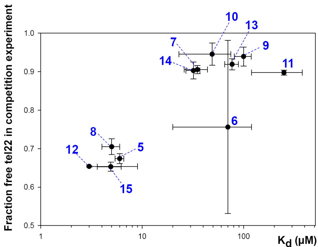
figure S3: The excellent correlation between the K_d for ligand binding to tel22 and determination and the fraction free tel22 found in the competition experiment shows that the competition experiment is a reliable way to assess relative ligand binding affinities for several DNA structures at the same time.
