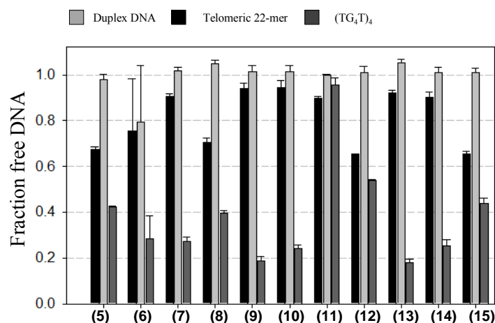
Figure S5: Results of ESI-MS competition experiments for the series of ligands reported here, showing in each instance the fraction of free DNA for three oligonucleotides. Ligands are defined in Table 1.
