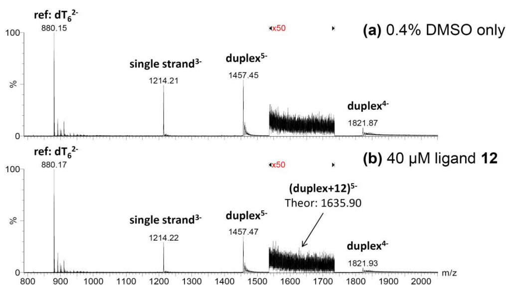
Figure S4: ESI-MS spectra of (a) 5 \mu\text{M} duplex (dCGCGAATTCGCG) 2 alone with 2 \mu\text{M} reference strand dT 6 , and of (b) 5 \mu\text{M} duplex (dCGCGAATTCGCG) 2 with 2 \mu\text{M} reference strand dT 6 and 40 \mu\text{M} of ligand 12 . The 1:1 complex between the duplex and the ligand
