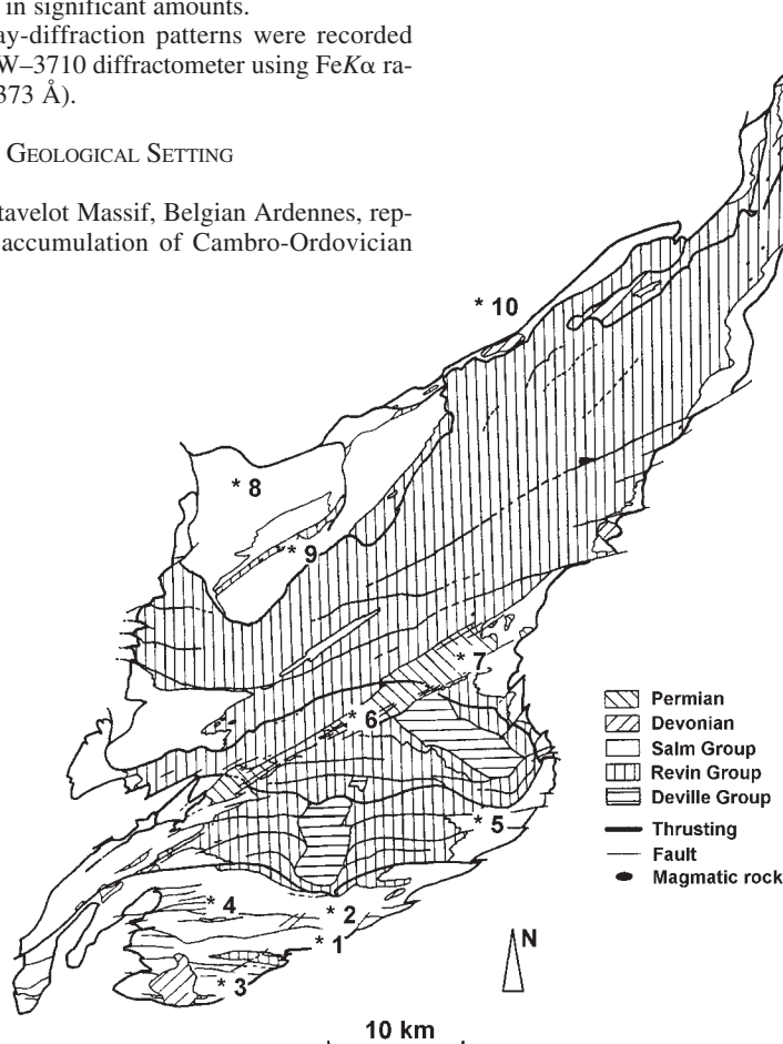
FIG. 1. Geological map of the Stavelot Massif, Belgium (after Geukens 1999). 1: Salmchâteau, 2: Vielsalm, 3: Bihain, 4: Lierneux, 5: Recht, 6: Stavelot, 7: Malmédy, 8: Theux, 9: Spa, 10: Eupen.
