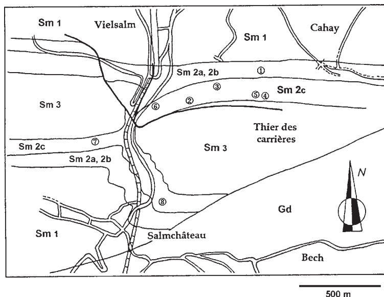
FIG. 2. Location of the copper sulfide mineralization in the Vielsalm–Salmchâteau area. Sm 1: Jalhay Formation, Sm 2a: Meuville Member, Sm 2b: Les Plattes Member, Sm 2c: Colanhan Member, Sm 3: Bihain Formation. The numbers correspond to those given in Table 1. Geological map after Fourmarier (1944), stratigraphy after Geukens (1999) and Verniers et al. (2001).
