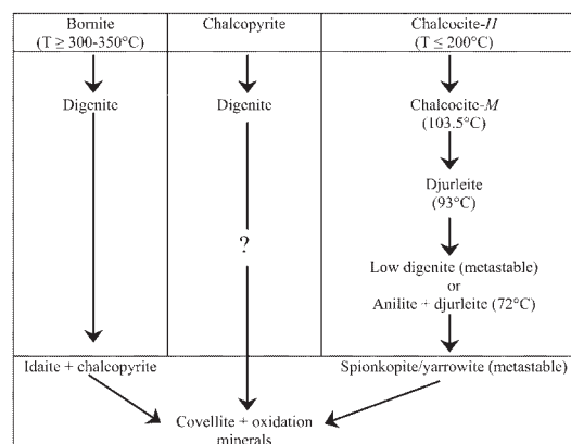
Fig. 5. Sequences of transformation in the copper sulfides from the Vielsalm-Salmchâteau area.
