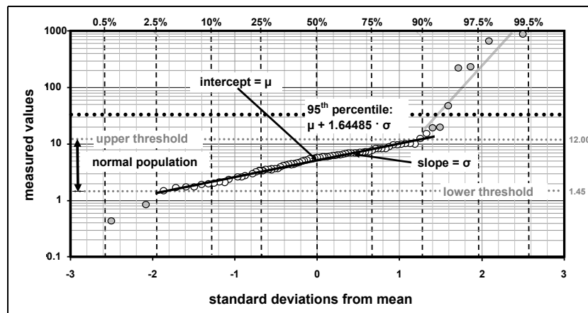
Fig 1: Filtering of anomalies, fitting of line of best fit to the remaining data and derivation of their relevant distribution parameters ( \mu = mean, \sigma = standard deviation).
