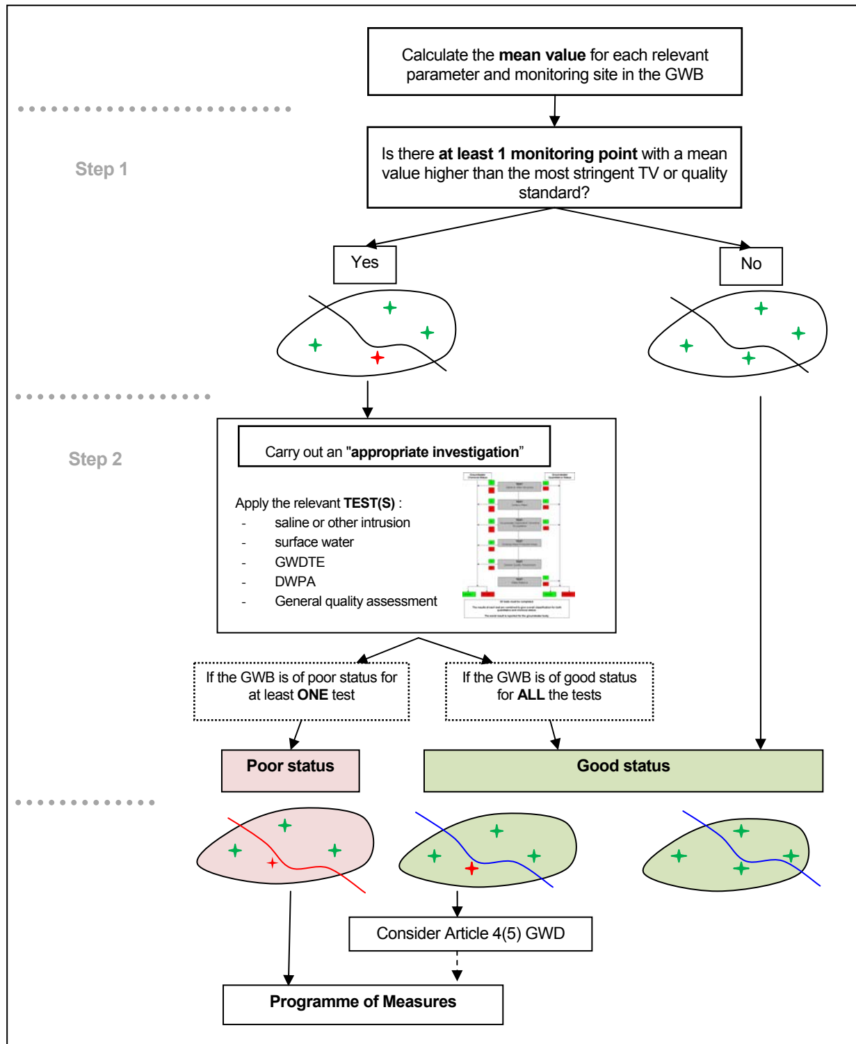
Figure 1: General procedure to assess a GWB chemical status.
