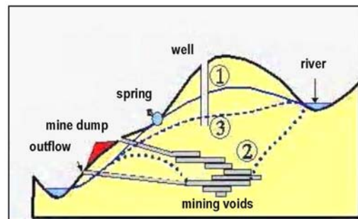
Figure 2: Perturbation of groundwater circulations due to mining works and abandonment (INERIS) (Legend: ① initial state, ② state during mining works, ③ final state after mining abandonment).
