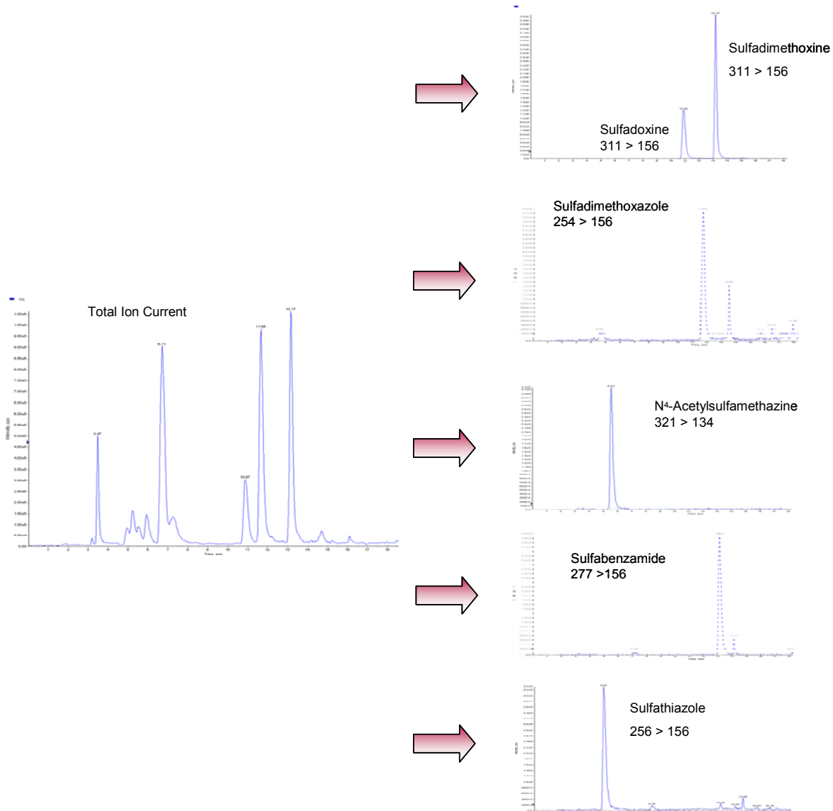
Figure 2. Total ion current (TIC) and single ion chromatograms showing the most abundant transitions of five of the sulfonamides studied in a matrix-matched standard solution of 1 ng/L.
