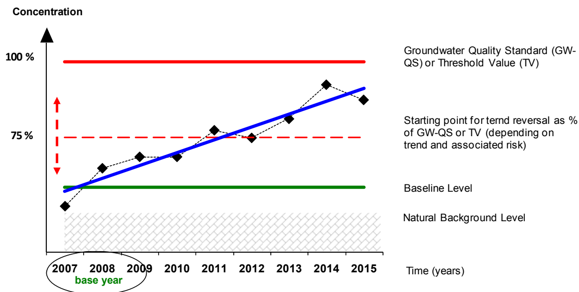
Figure 2: Elements of trend and trend reversal assessment.
