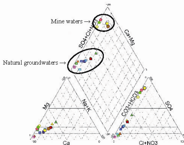
Figure 1: Piper diagram of natural and mine groundwaters (southern France, INERIS).
