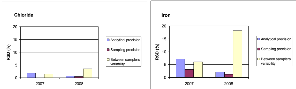
Figure 2: Selected statistical results from Danish groundwater sampling proficiency test in 2008.
