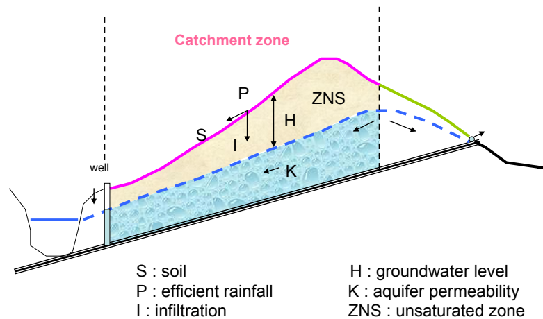
Figure 2 - Parameters used for vulnerability mapping in a case of continuous aquifer
