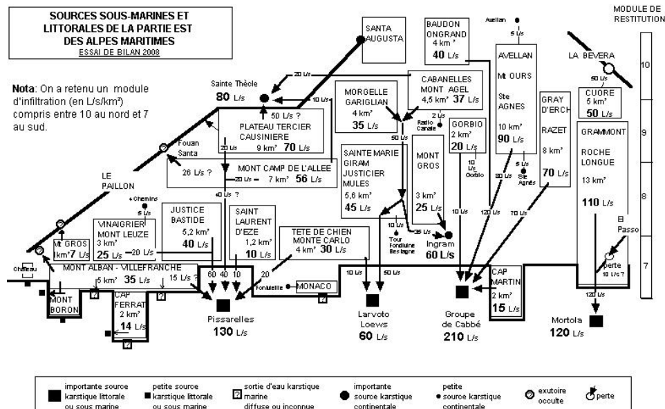
Figure 1: Groundwater balance of the karstic units between Nice and menton (France).
