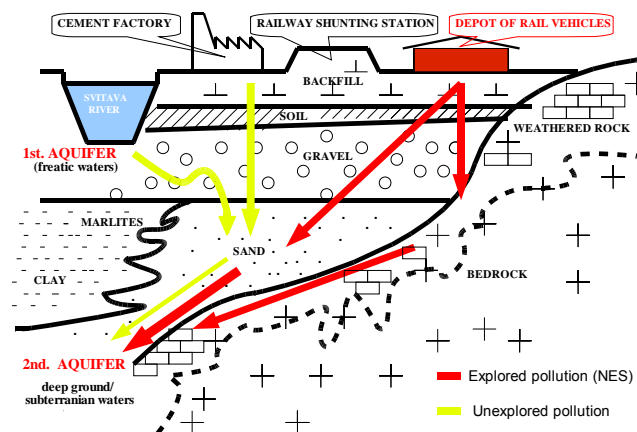
Figure 1: Geological section and the ways of contamination.
