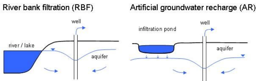
Figure 1: Most common MAR techniques in Europe: Bank filtration (BF), artificial groundwater recharge (AR).
