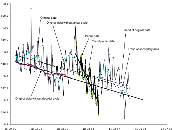
Figure 1: Time evolution head.
