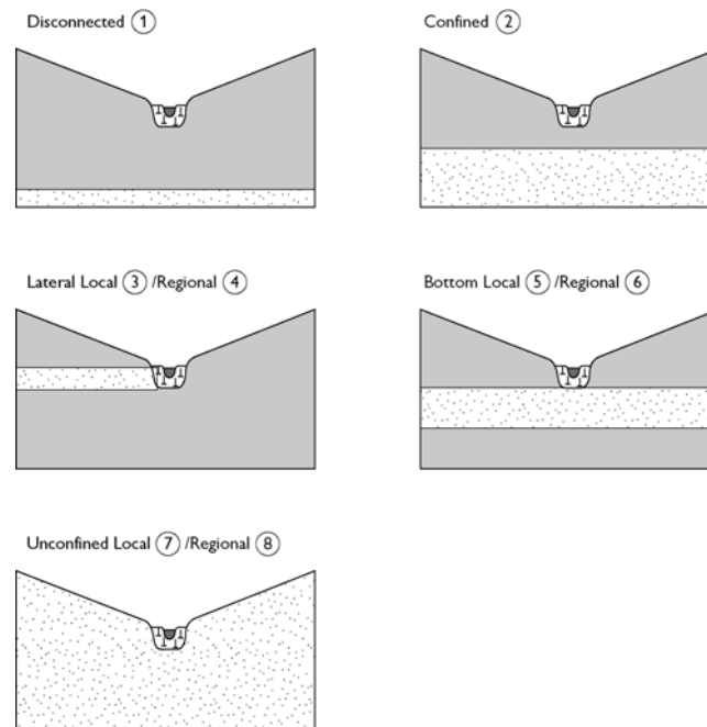
Figure 3: Riparian Hydrogeological Types. The hydrogeological legend corresponds to Figure 2.
