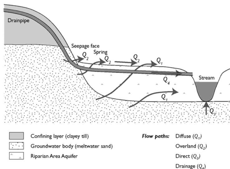
Figure 4: Flow paths through a riparian area to a stream.
