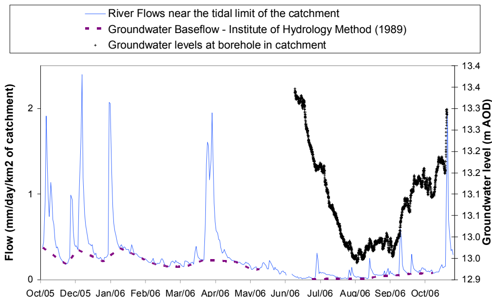
Figure 2. Comparison of measured river flow and groundwater baseflow at the tidal limit of the largest catchment.
