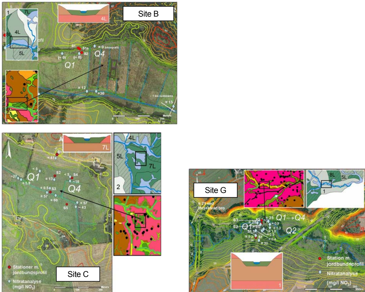
Figure 7: Information in restoration sites B, C and G applied to guide protection strategies against nitrate load to Åkær stream. Nitrate concentrations in mg/l in December 2007.
