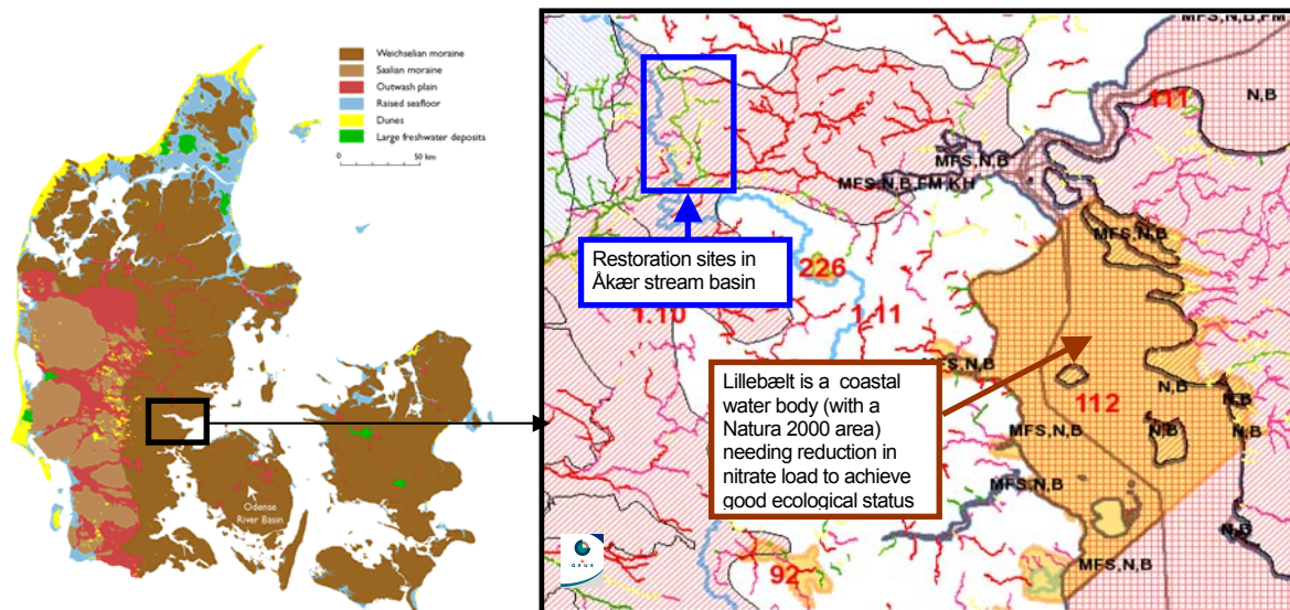
Figure 5: Case study area in a moraine landscape in Denmark. Åkær Stream (blue square) is recharged by a nitrate polluted Local Groundwater Body (red cross hatched) of poor status. The receiving Lillebælt coastal water body also has a poor status (red square hatched). A Natura 2000 area (yellow) is situated in Lillebælt.
