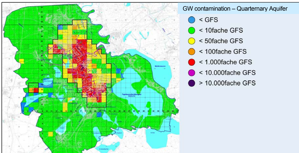
Figure 2: Exceedance of threshold values (GFS) in groundwaterbody “Pilotarea Bitterfeld-Wolfen” (VM 2-4).
