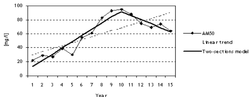
Figure 4: Two-sections model for assessing trend reversal.
