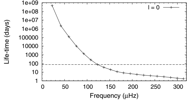
Fig. 4. Theoretical lifetimes of radial modes of model A. The horizontal line corresponds to our choice of the resolution limit (75 days).
