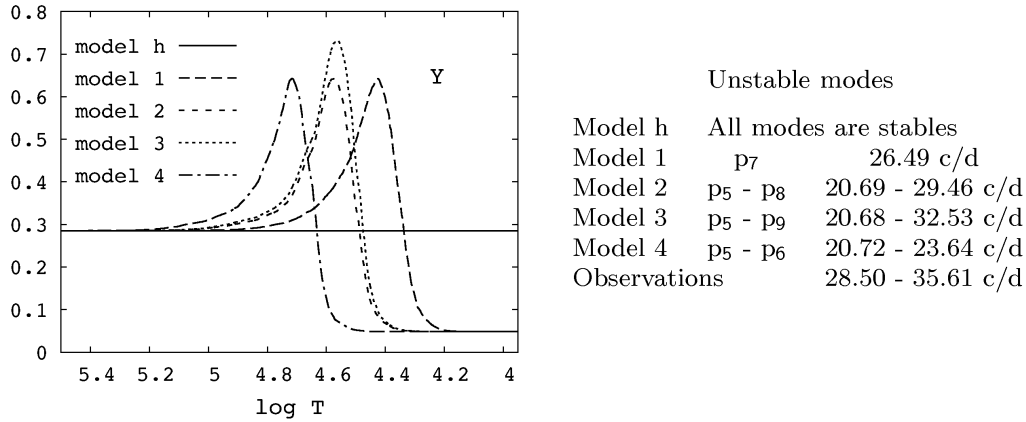
Figure 1: Left: Different He profiles. Right: Ranges of predicted unstable modes as compared with the observed frequency range.
