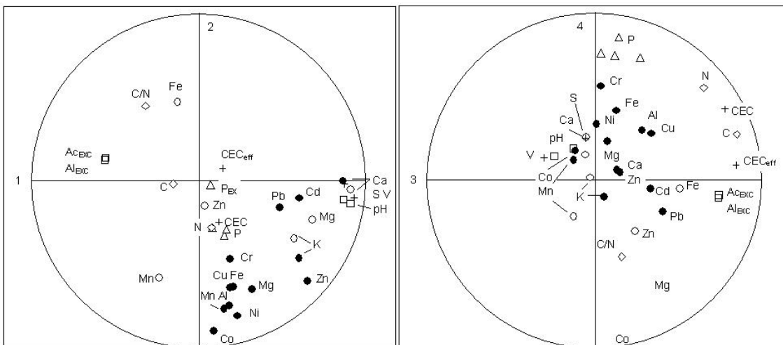
Figure 3 Scatter plots of correlations between forest soil properties and the first two principal components (left) or third and fourth (right).
