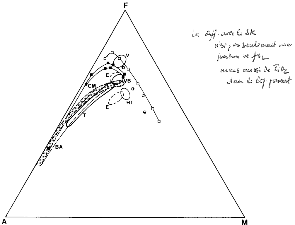
Fig. 1 A ( \text{Na}_2\text{O} + \text{K}_2\text{O} ) - F ( \text{FeO} + 0.9 \text{Fe}_2\text{O}_3 ) - M ( \text{MgO} ) diagram for representative monzonorites and related rocks. The clusters enclose the data from the various occurrences. List of abbreviations: Rogaland occurrences: T, Tellnes dike; VB, Varberg dike; V, Vettaland dike; HT, Hydra massif and Tjörn chilled margins. Other occurrences: E (two clusters), Labrador (Harp Lake, Nain) and Grenville Province (Belleau-Desaulniers, Grenville Township, Morin, Lac Croche, Marcy, Snowy Mountain), from EMSLIE (1978); BA, Loch Ba ring dike, Scotland, from SPARKS (1988); CM (dotted cluster), Crater of the Moon, Snake River Plain, Idaho, from LEEMAN et al. (1976); (star), Skaergaard chilled marginal gabbro KT39, from HOOVER (1989); \square (open square), Skaergaard liquid evolution calculated by Wager (WAGER and BROWN, 1968); \blacksquare (full square), Skaergaard liquid evolutions calculated by HUNTER and SPARKS (1987); partial melts from high-alumina basalt obtained by BAKER and EGGLEER (1987): \bullet , high-alumina basalt AT-112; \circ , run number 1098, 6% glass at 8 kb; \odot , run number 953, 44% glass at 8 kb.
