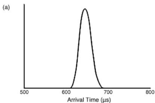
Fig. 3. (a) A single peak ATD was acquired for the -5 and -6 charge states of [(dTG_4T)_4 + 3NH_4] and [(T1)_4 + 2NH_4] . The ATD shown is for [(dTG_4T)_4 + 3NH_4]^{5-} with a cross section of 775 \text{ \AA}^2 . Parallel quadruplex structures for (b) [(dTG_4T)_4 + 3NH_4]^{5-} and (c) [(T1)_4 + 3NH_4]^{5-} that match the experimental cross sections.
