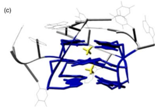
(T1)_4 Parallel \sigma_{\text{Theory}} = 799 \text{ \AA}^2
