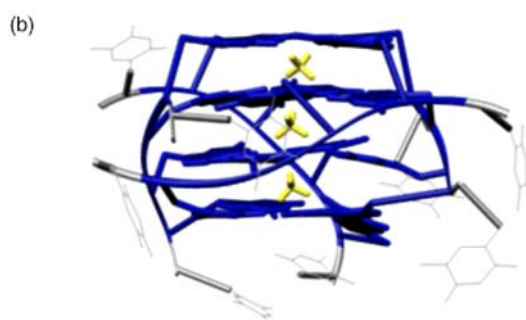
(dTG_4T)_4 Parallel \sigma_{\text{Theory}} = 780 \text{ \AA}^2
