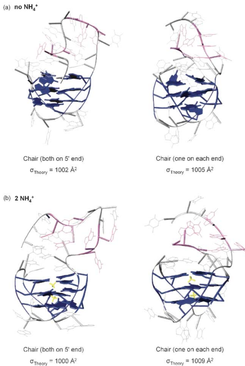
Fig. 9. The theoretical antiparallel chair structures for T6^{5-} in which the two extra T_2AG_3 are either on the 5' end, or one on the 5' end and the other on the 3' end. Structures are shown (a) without NH_4^+ and (b) with 2NH_4^+ .
