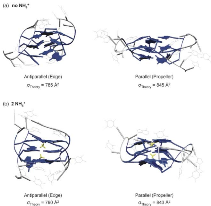
Fig. 5. The theoretical structures for the antiparallel (edge) and parallel (propeller) structures of (T2)_2 that match the experimental cross sections (a) without NH_4^+ stabilization and (b) with NH_4^+ stabilization.
