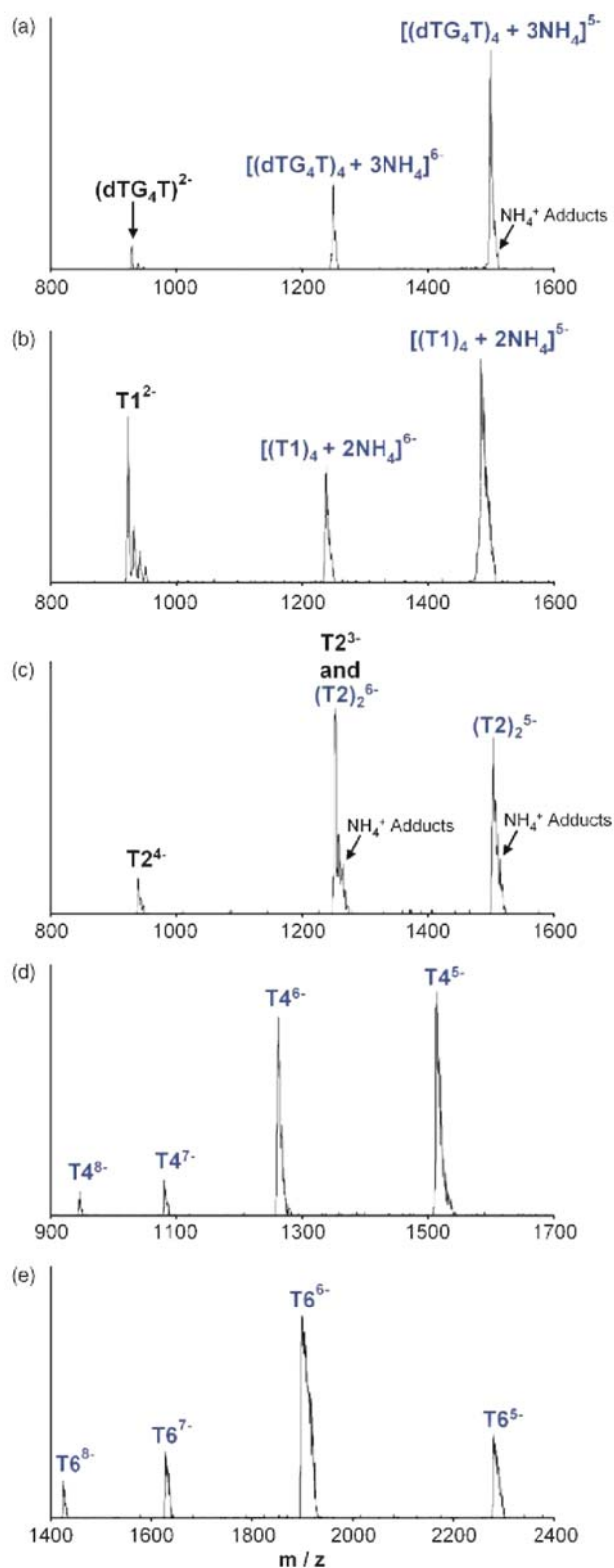
Fig. 2. Nano-ESI mass spectra for (a) dTG_4T , (b) T1 , (c) T2 , (d) T4 and (e) T6 . The dominant peaks for the 4-strand complexes of T1 and dTG_4T have 2 and 3 NH_4^+ adducts, while the dominant peaks for (T2)_2 , T4 and T6 do not have NH_4^+ adducts. All possible quadruplex stoichiometries are shown in blue. The background was subtracted on the spectra to clearly illustrate the peaks.
