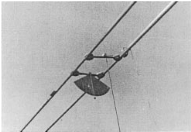
Fig. 10. Scale to visually measure rotation angle and angular potentiometer.
