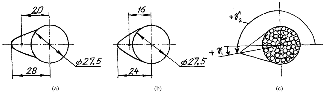
Fig. 5. Geometry of the airfoils of (a) ESSP and of (b) KazNIIE mounted on the conductor. Center of gravity location estimate for the airfoils is given. (c) Angle of attack definition.
