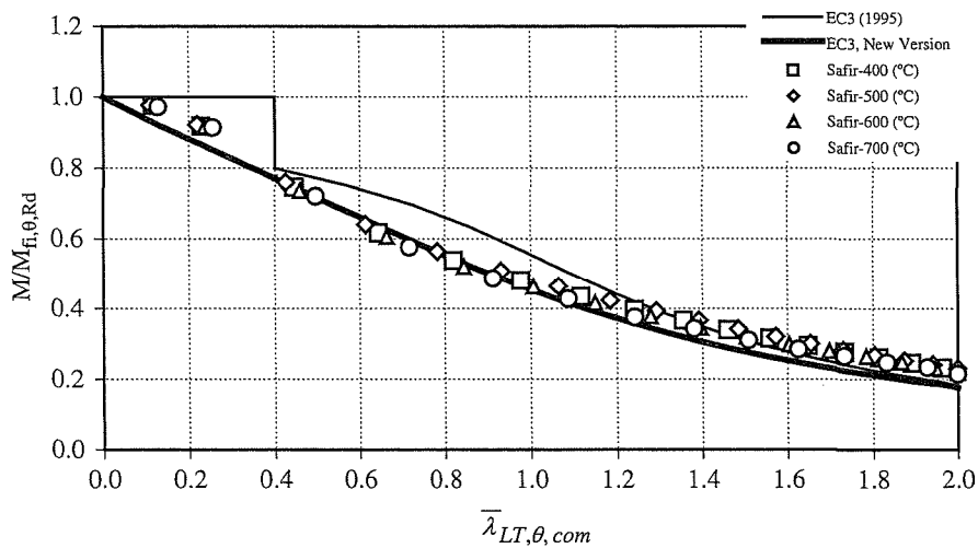
Fig. 4. Design curves for lateral torsional buckling of beams.
