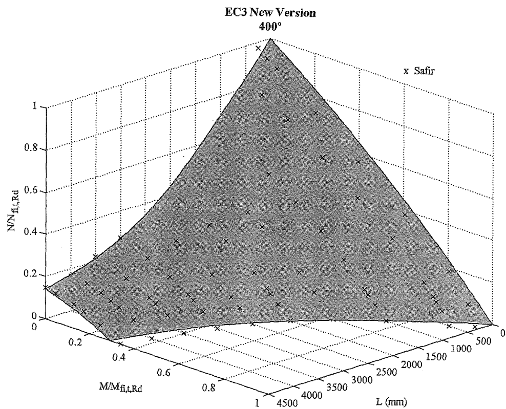
Fig. 8. Interaction surfaces for combined moment and axial load at 400°C—new version.
