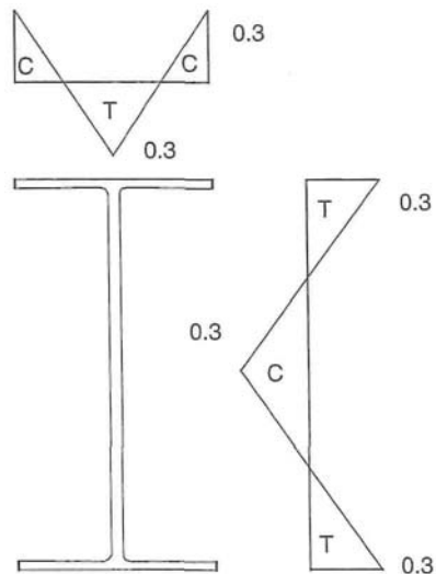
Fig. 2. Residual stresses: C—compression; T—tension.
