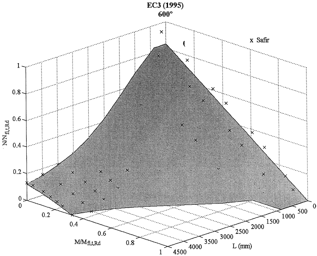
Fig. 9. Interaction surfaces for combined moment and axial load at 600°C—version from 1995.
