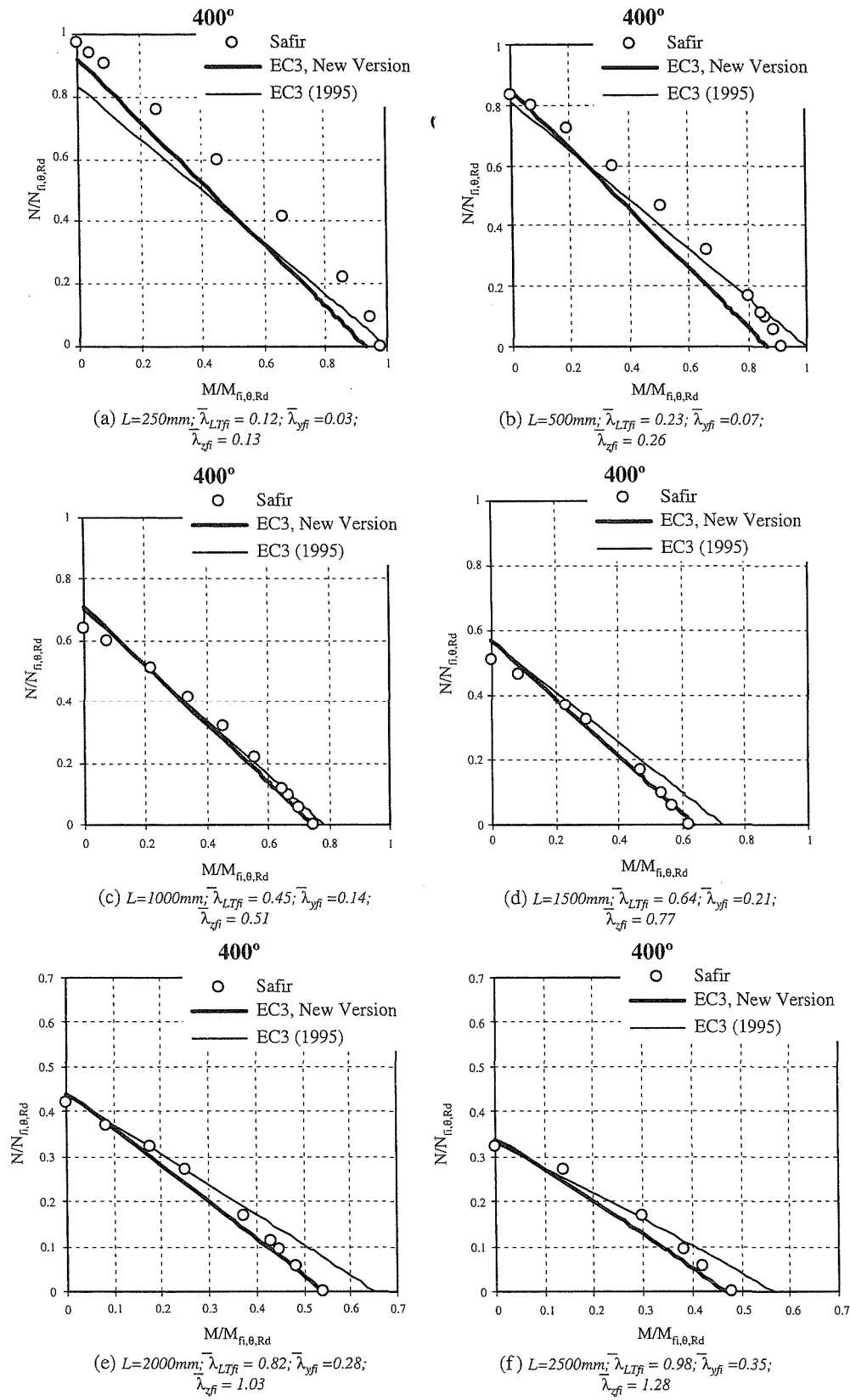
Fig. 5. Interaction diagrams for combined moment and axial load at 400°C.
