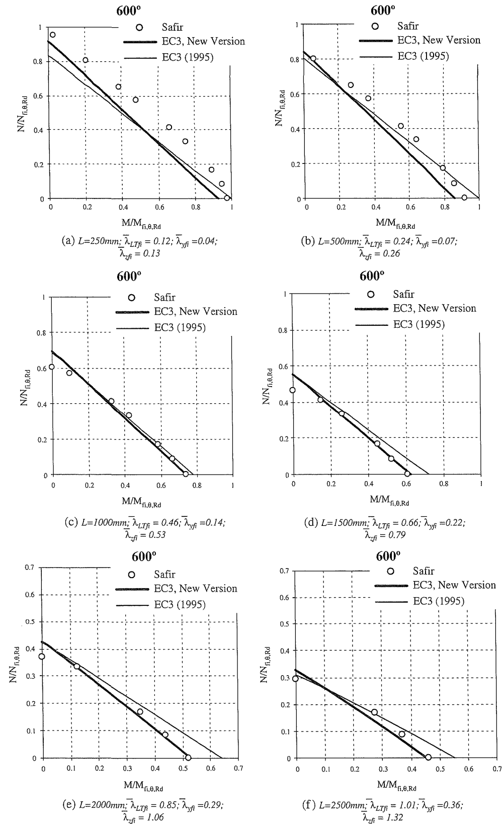
Fig. 6. Interaction diagrams for combined moment and axial load at 600°C.
