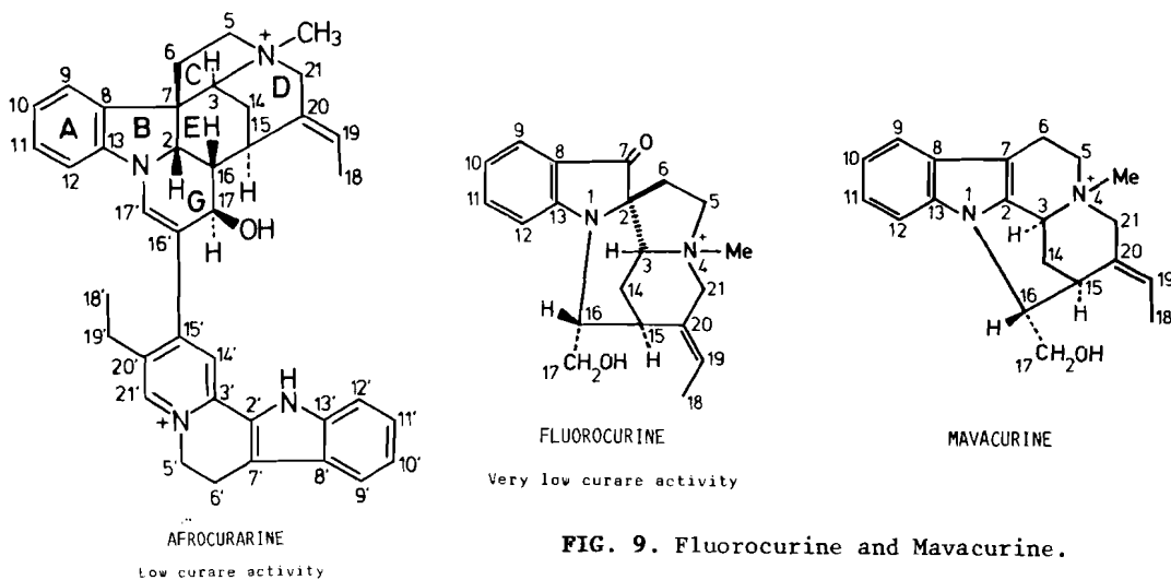
FIG. 8. Afrocurarine.
