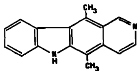
ELLIPTICINE
