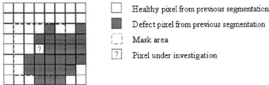
Fig. 4. Mask used by the algorithm.
