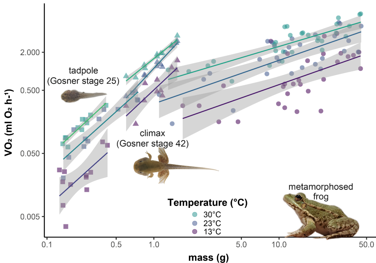
Fig. 1: Allometric effect of body size on oxygen consumption for three developmental stages and three temperatures in invasive marsh frogs ( Pelophylax ridinbundus ). Logarithm scales were used for each axis. Each square stand for an individual tadpole, triangles for metamorphosing individuals (climax stage), and circles for metamorphosed stages. The lines represent the linear regressions of oxygen consumption on body mass and the grey shade the confidence interval. The violet color stands for a 13 °C test temperature, blue for 23 °C, and green for 30 °C.
