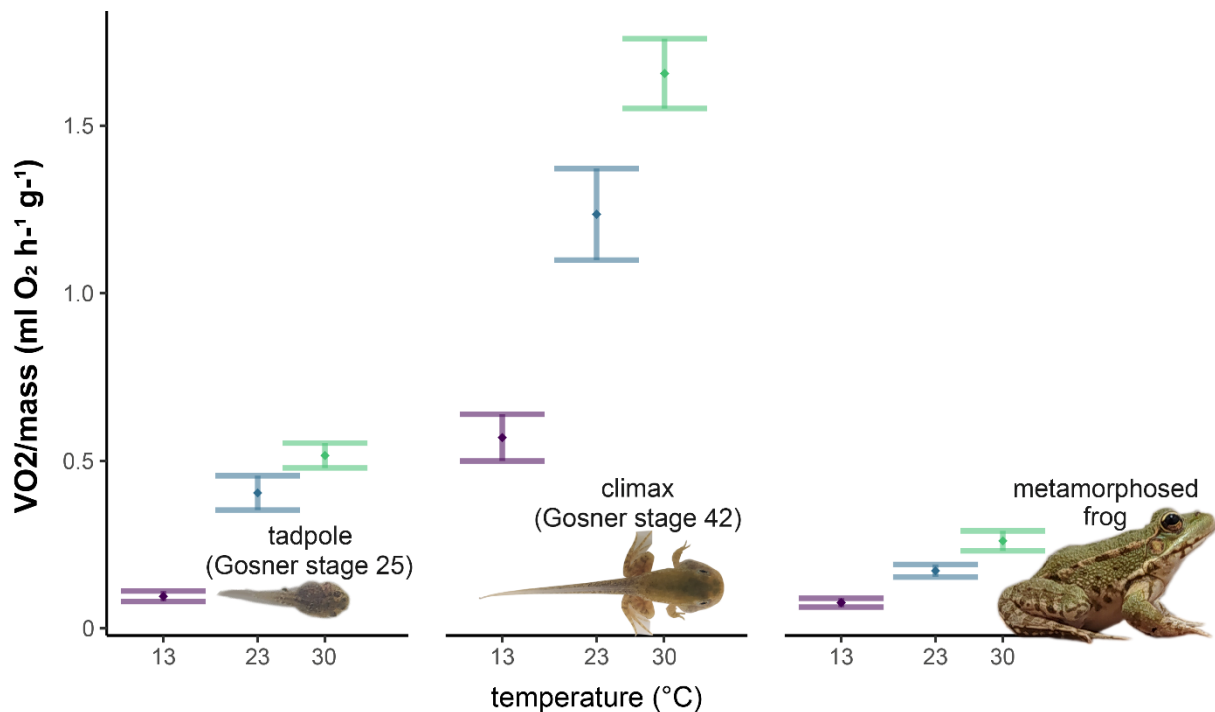
Fig. 2: Thermal dependency of the mass specific metabolic rate among developmental stages of invasive marsh frogs ( Pelophylax ridibundus ). Standard errors are represented by error bars and the dots represent the mean. The violet color stands for a 13 °C test temperature, blue for 23 °C, and green for 30 °C.
