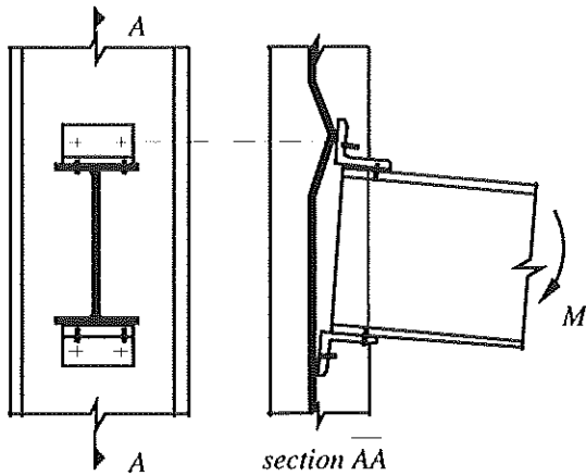
Fig. 3. Local mechanism
