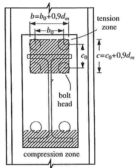
Fig. 8. Bolted connection
