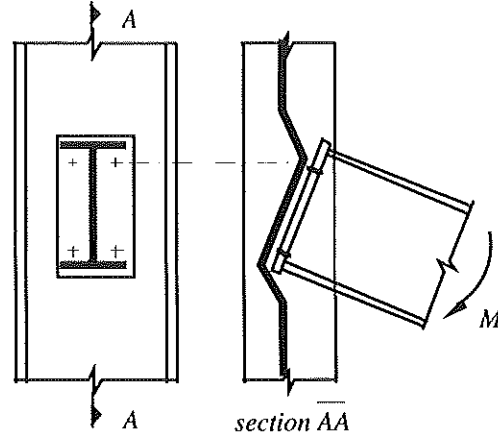
Fig. 4. Global mechanism
