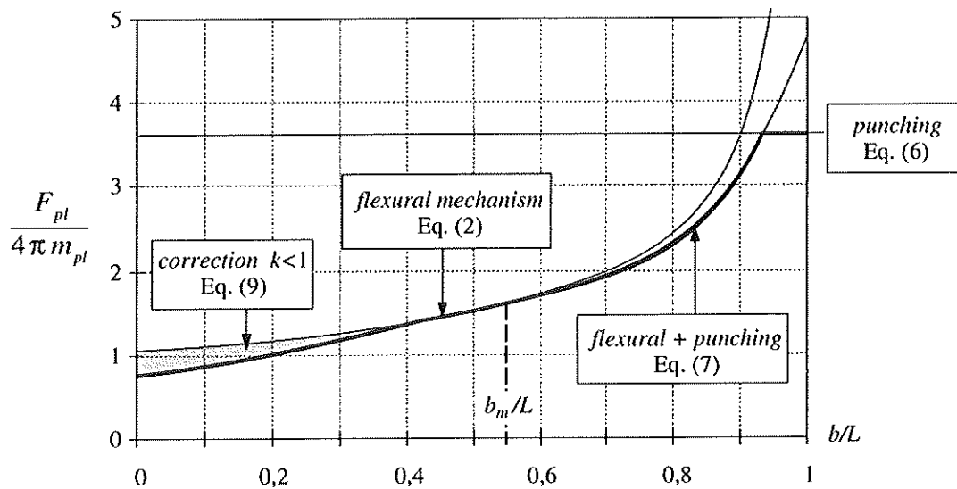
Fig. 12. Comparison between the three modes of local failure
