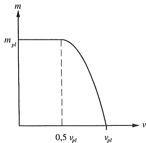
Fig. 10. Interaction between m (moment) and v (shear force)
