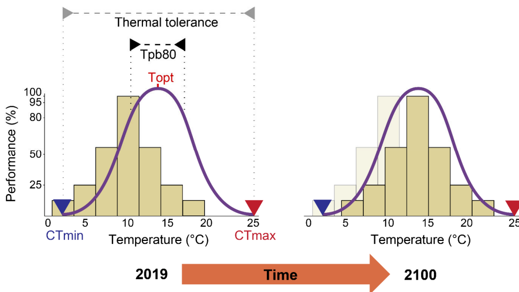
Fig. 1 Theoretical representation of a shift of annual temperature distribution (histogram) that better fits a performance curve of an invasive ectotherm. The shift has been increased for readability. The curve, in purple, is bounded by the critical thermal minimum (CT min , blue triangle), and the critical thermal maximum (CT max , red triangle). The range of temperature between these bounds defines the thermal tolerance where the organism can maintain activity (horizontal grey dashed lines). The temperature associated with the maximum value of performance defines the thermal optimum (T opt , red). Finally, the range of temperatures where performance is greater or equal to a desired level (commonly 80% or 95%) defines a performance breadth (T pb , horizontal black dashed line; Angilletta et al., 2002).
