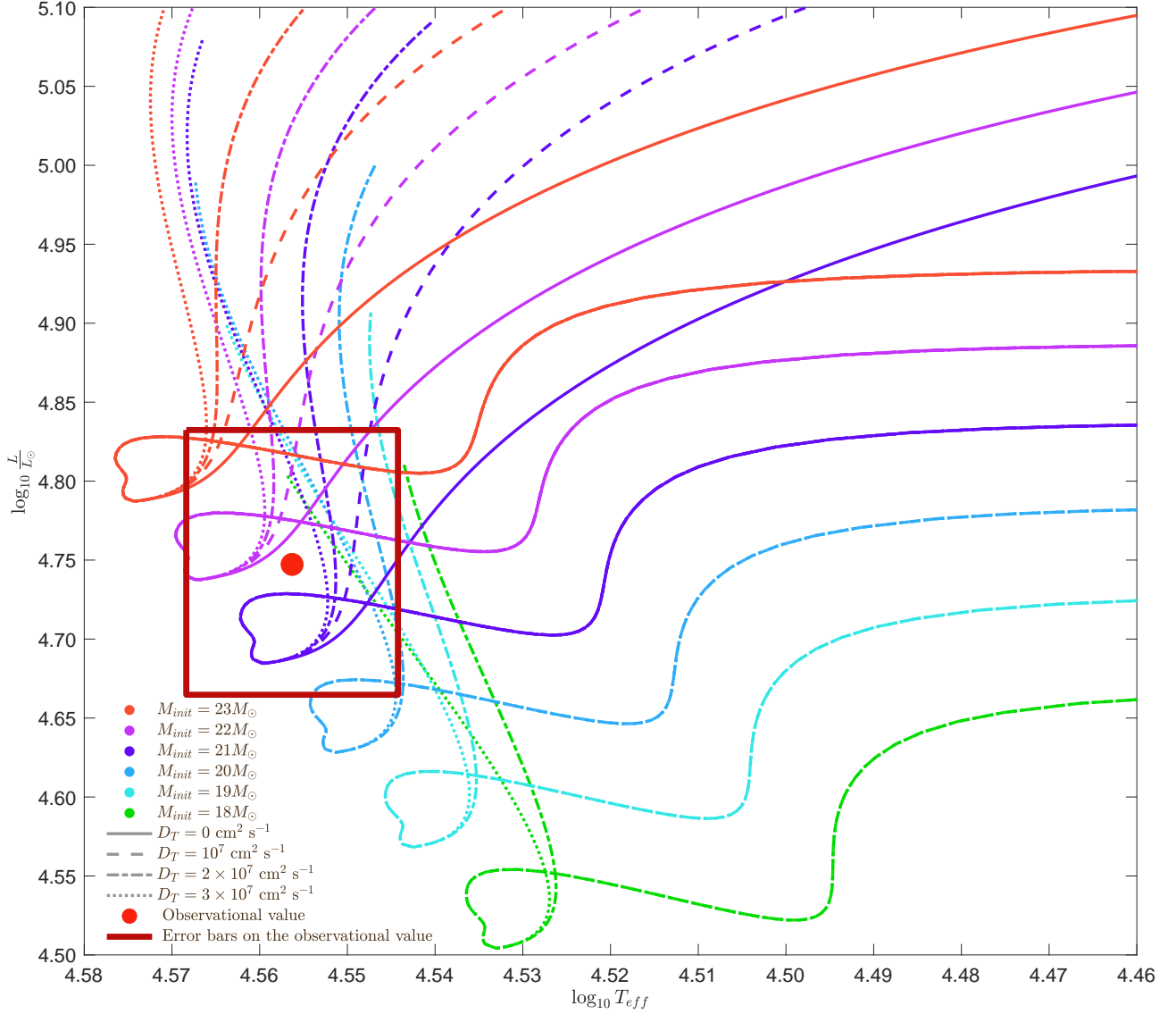
Figure 7. Hertzsprung-Russell diagram: evolutionary tracks of Clés models for the secondary star of M_{init} = 18 M_{\odot} (green), 19 M_{\odot} (turquoise), 20 M_{\odot} (light blue), 21 M_{\odot} (purple), 22 M_{\odot} (plum), and 23 M_{\odot} (coral), and D_T = 0 \text{ cm}^2 \text{ s}^{-1} (solid line), 10^7 \text{ cm}^2 \text{ s}^{-1} (dashed line), 2 \times 10^7 \text{ cm}^2 \text{ s}^{-1} (dotted-dashed line), and 3 \times 10^7 \text{ cm}^2 \text{ s}^{-1} (dotted line). All models have \xi = 1 and \alpha_{ov} = 0.30 . The observational value is represented by the red point, and its error bars are represented by the dark red rectangle.
