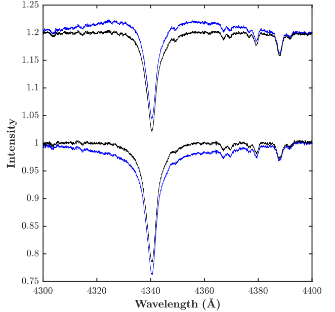
Figure 1. Reconstructed spectra of the stellar components of HD 165052 in the wavelength domain around the H \gamma line, using the shift and add method (blue) and the QER20 Package (black). The spectra of the stellar components are vertically shifted for clarity.
