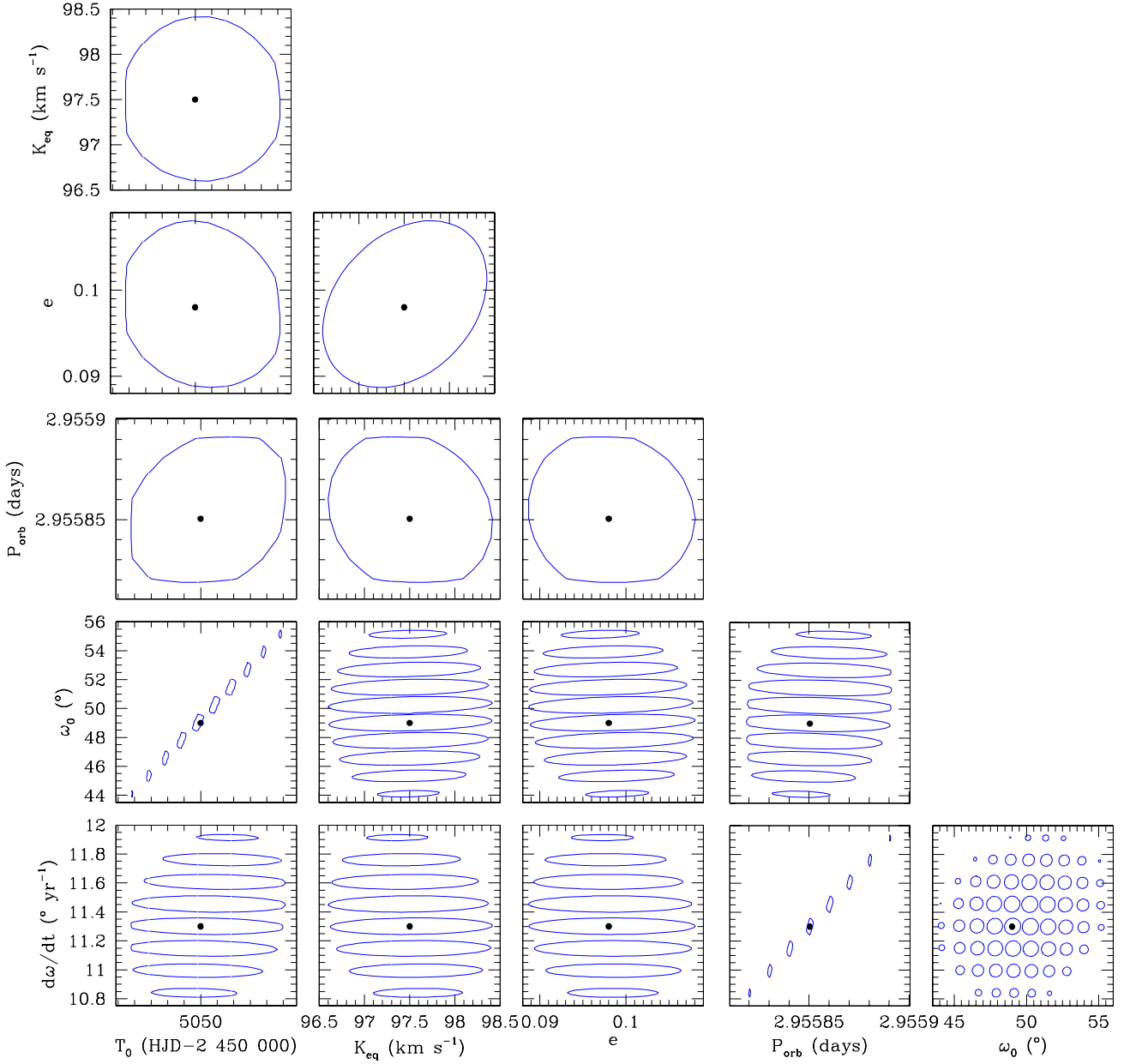
Figure 4. Confidence contours for the best-fit parameters obtained from the adjustment of the equivalent RV data of HD 165052. The best-fit solution is shown in each panel by the black filled dot. The corresponding 1\sigma confidence level is shown by the blue contour. We note the “zebra-like” strips for \omega_0 and \dot{\omega} are computational artefacts.
