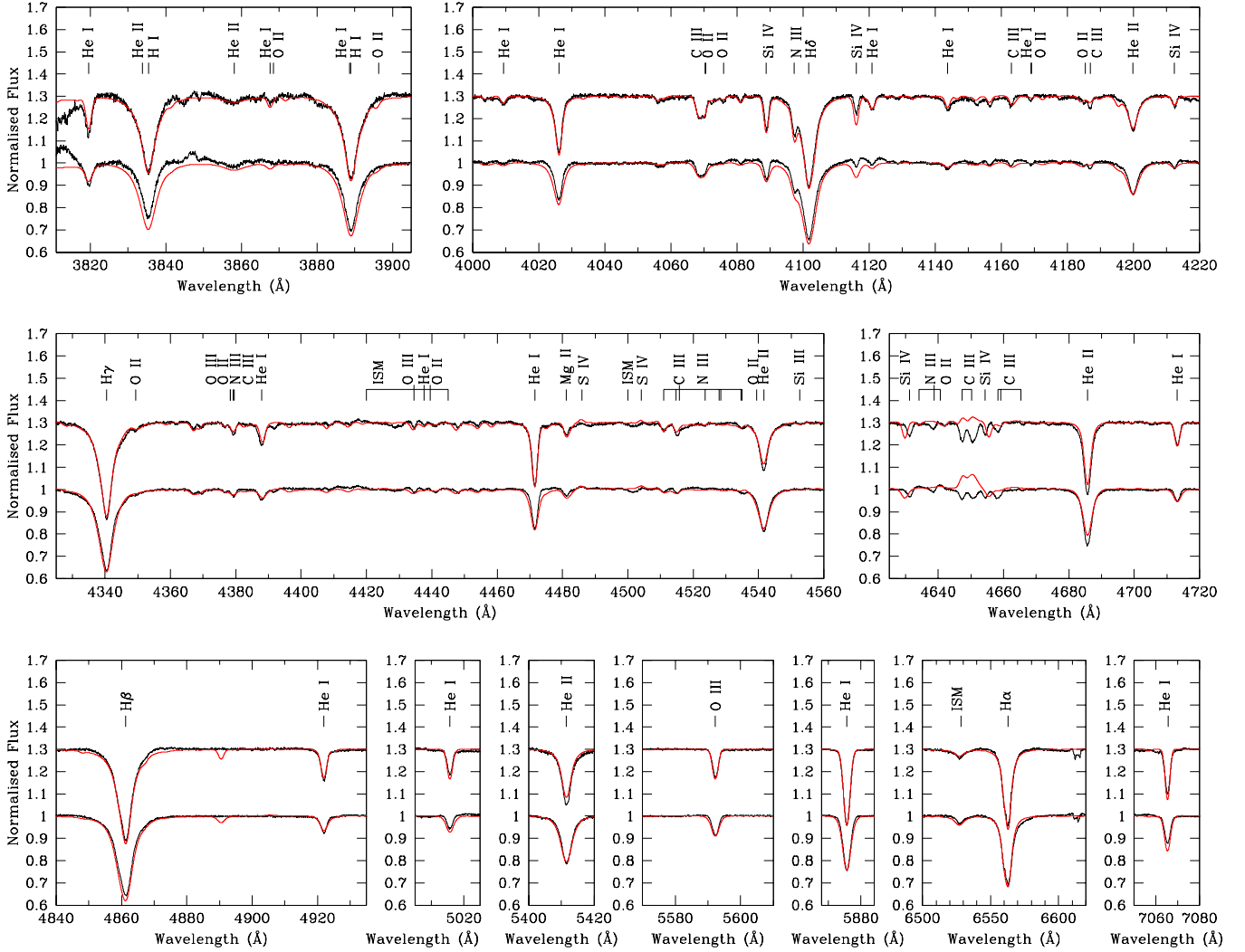
Figure 3. Normalised disentangled spectra (in black) of the primary and secondary stars of HD 165052 (the spectrum of the secondary star is shifted by +0.3 in the y-axis for clarity) together with the respective best-fit CMFGEN model atmosphere (in red).
