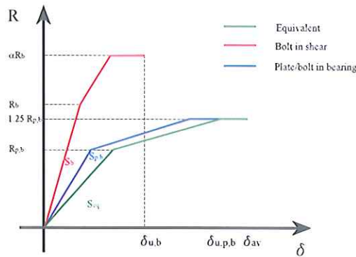
Figure 4 – Assemblage of the individual components behaviour.
