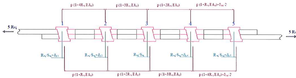
Figure 5 – Connection with 5 bolt rows.
