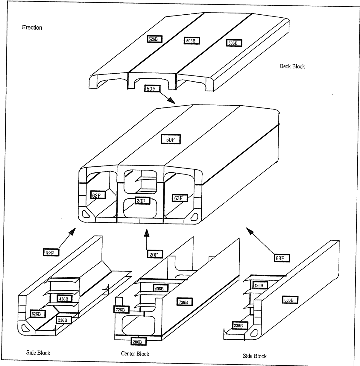
Figure 12a - Fabrication Sequence Diagram (Part 1)
