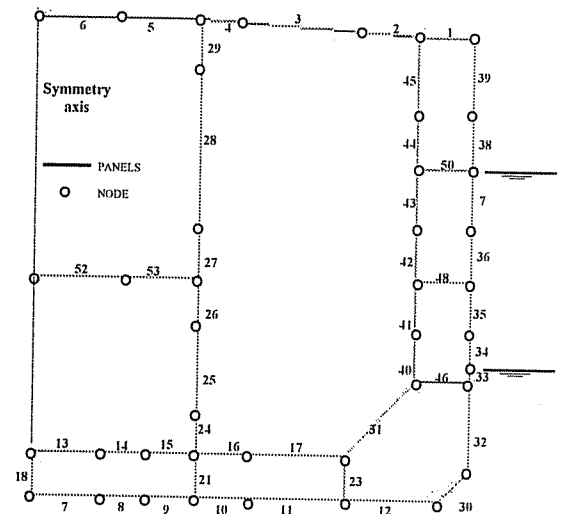
Figure 14 - LBR5 Product Mesh Model
