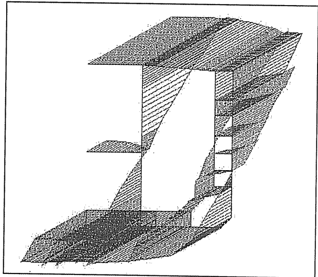
Figure 16 - Longitudinal Stress, \sigma(x) = 210 \text{ N/mm}^2 , 3D analysis (Sagging + load case 2).
