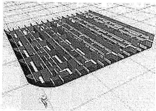
Figure 18 Location of double bottom section (left) and interior structure with top plate removed (right)
