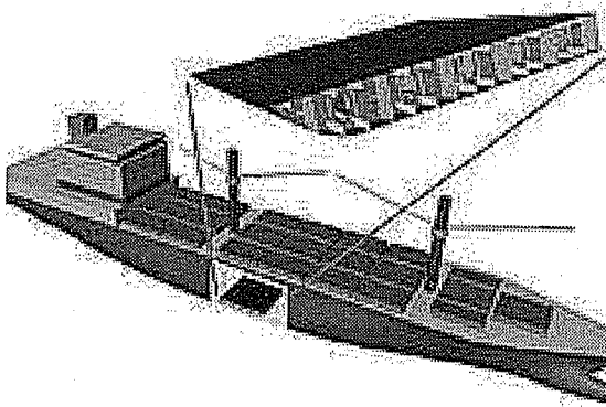
Figure 18 Location of double bottom section (left) and interior structure with top plate removed (right)
