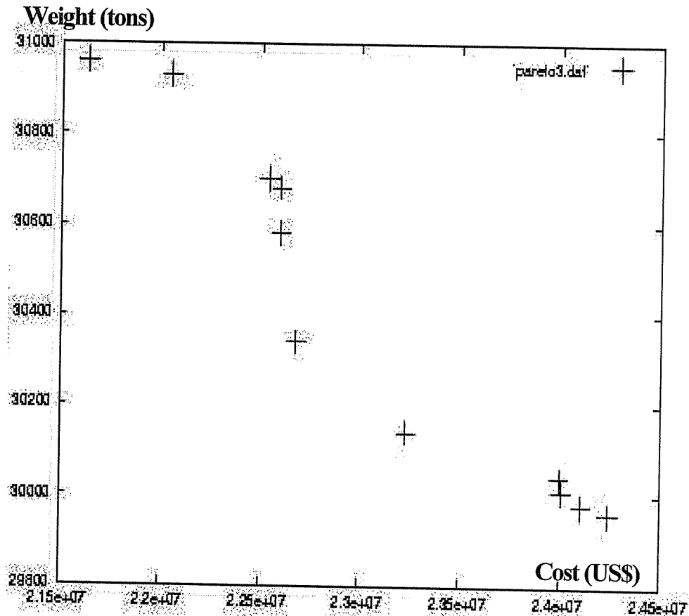
Figure 13 - Pareto Optimal Set - Optimum Weight versus Optimum Cost
