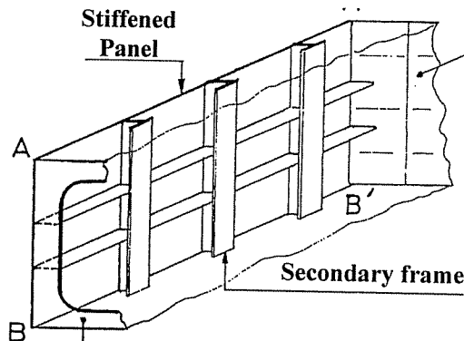
Figure 6 - A Stiffened Plate with Frames and Longitudinals (between 2 bulkheads)
