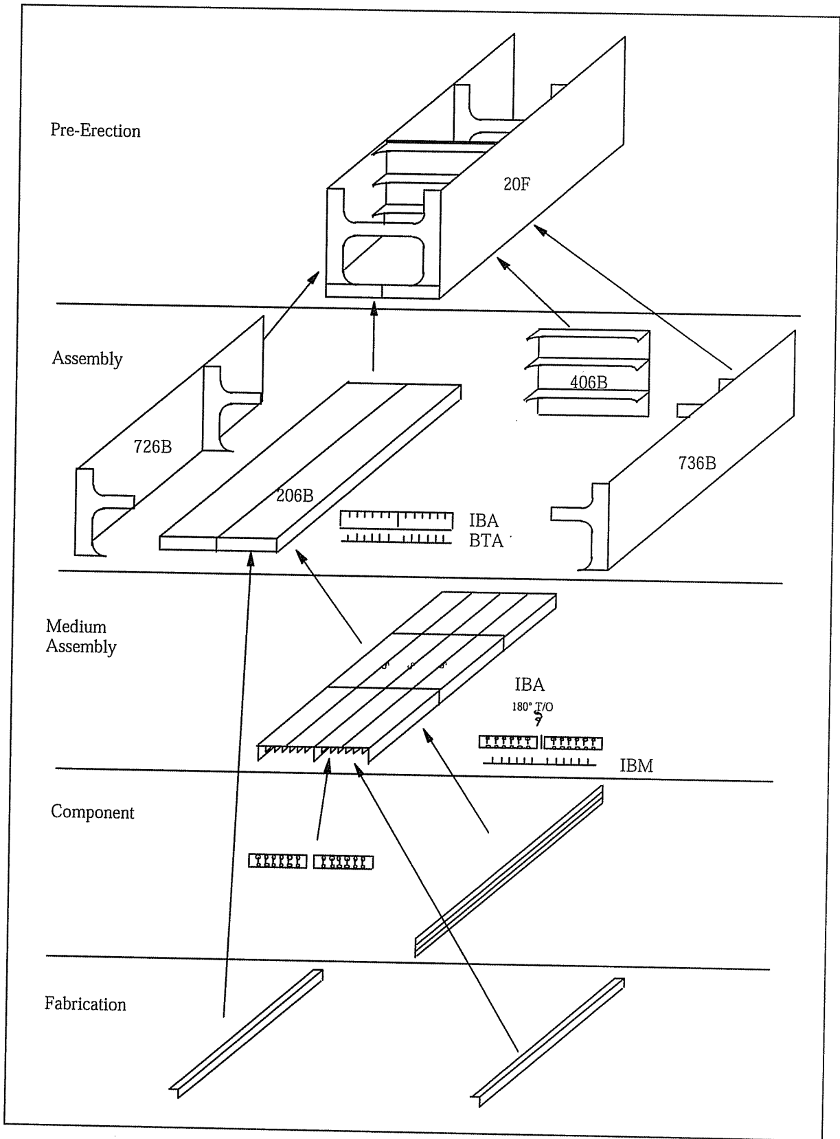
Figure 12b - Fabrication Sequence Diagram (Part 2)
