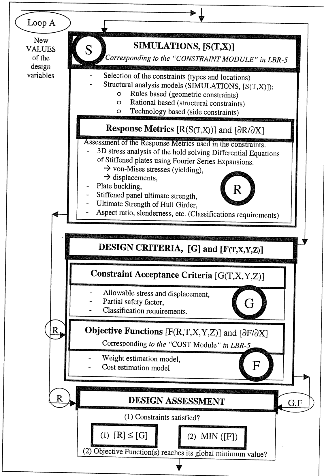
Figure 4-b The LBR-5 Framework (Part 2)
