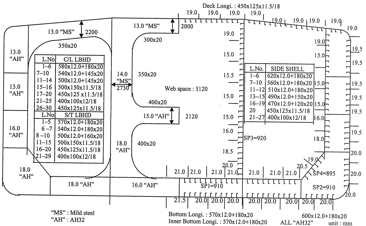
Figure 9 - Existing VLCC Ship Design
