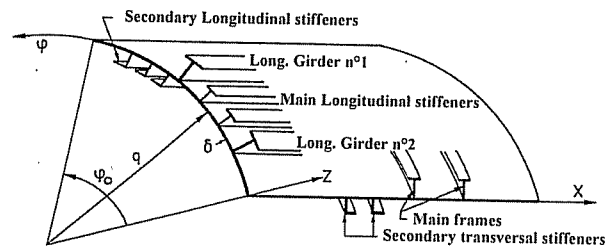
Figure 5 - A stiffened panel (Basic Product Element) of a LBR5 mesh model (including longitudinal and transversal members).
