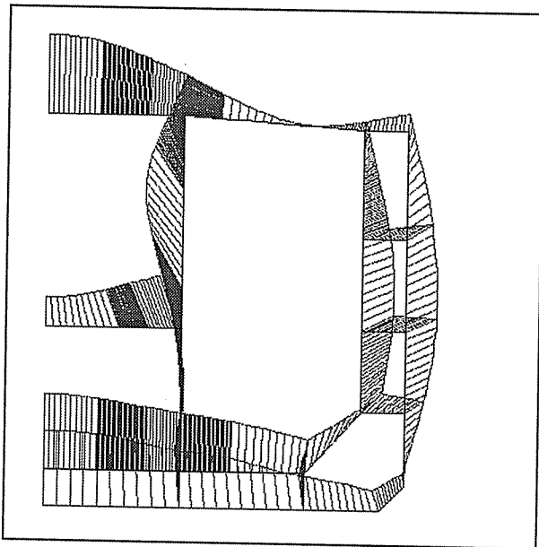
Figure 15 - Transversal Displacement ( \delta ), At mi-span of a block, \delta \text{ max } = 30 \text{ mm} , 2D analysis using a refined mesh model, (Load case 1)
