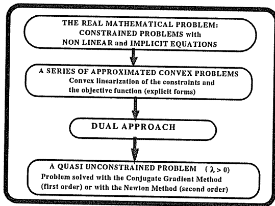
Figure 7 - An Optimization Module using Convex Linearization and Dual Method
