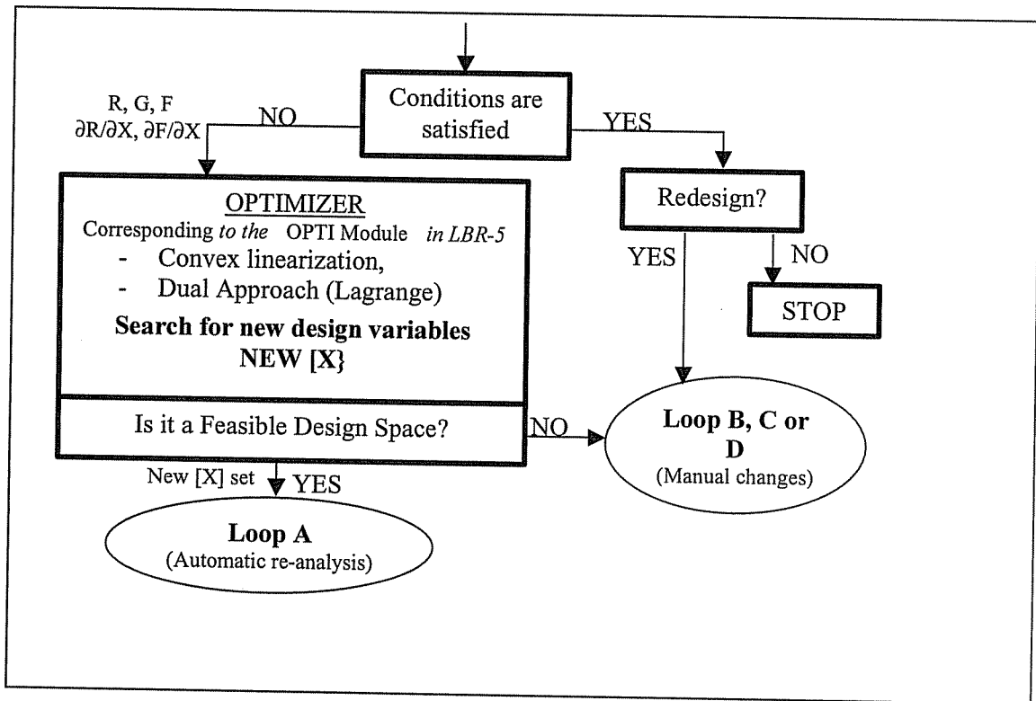
Figure 4c - The LBR-5 Framework (Part 3)
