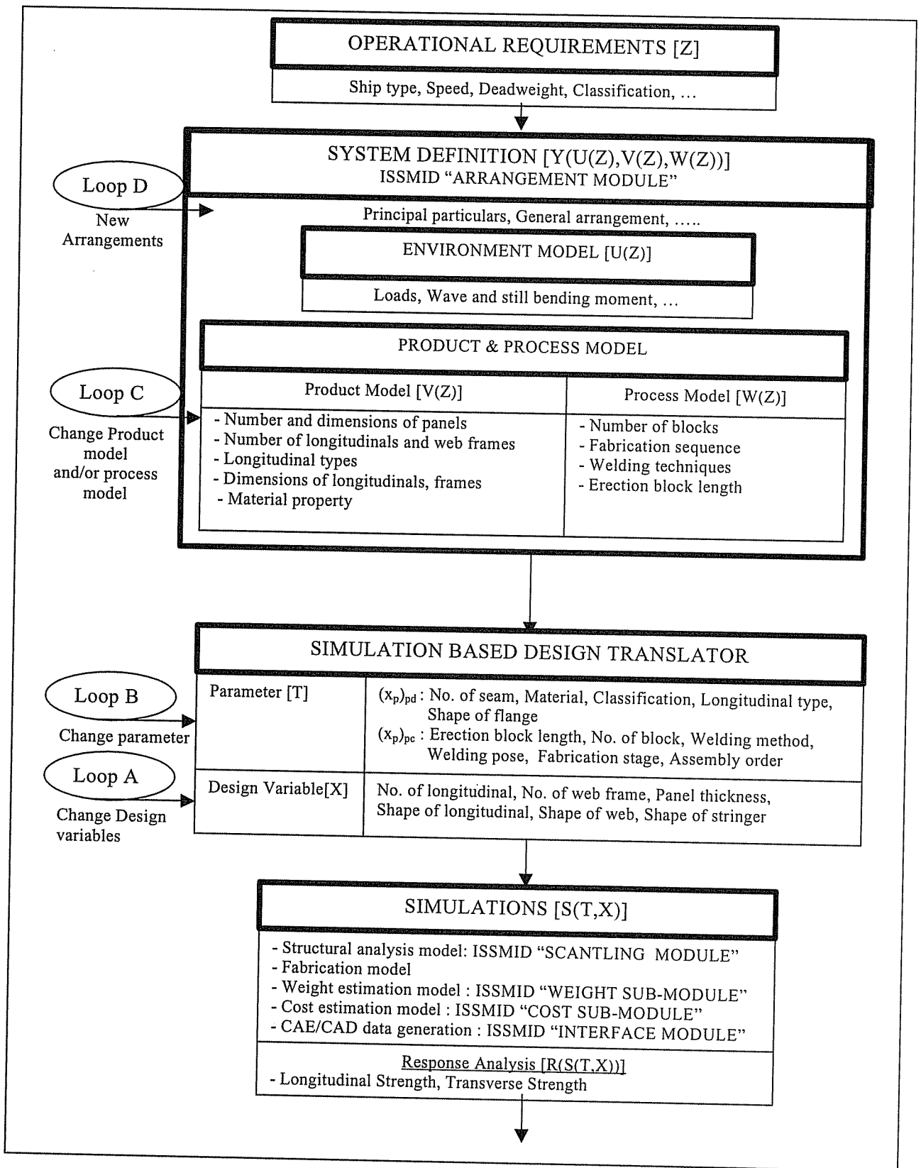
Figure 2a - ISSMID-T Framework (Part 1)
