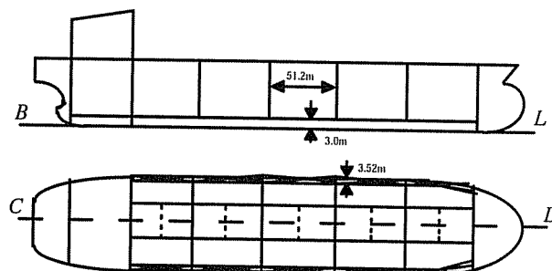
Figure 10 - General Arrangement (L=320 m; B=58 m; D=31 m; T=22 m and C B =0.83)
