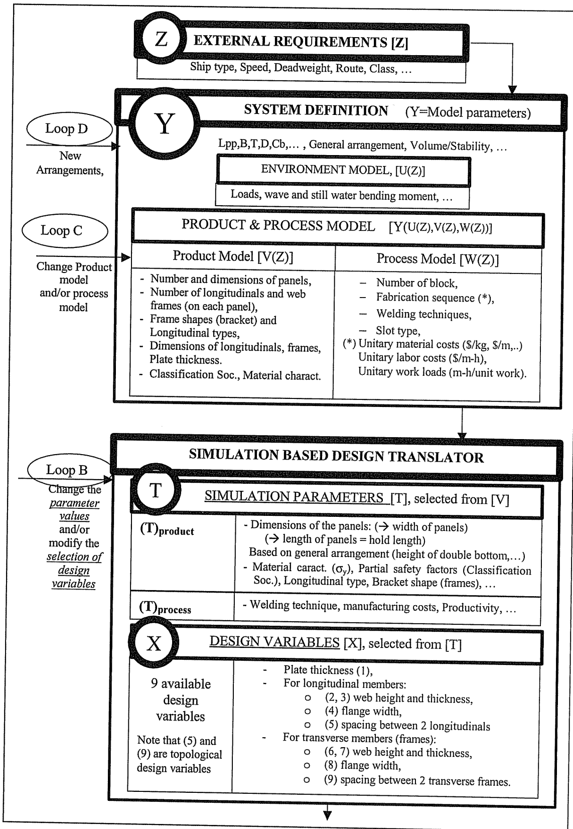
Figure 4a - The LBR-5 Framework (Part 1)
