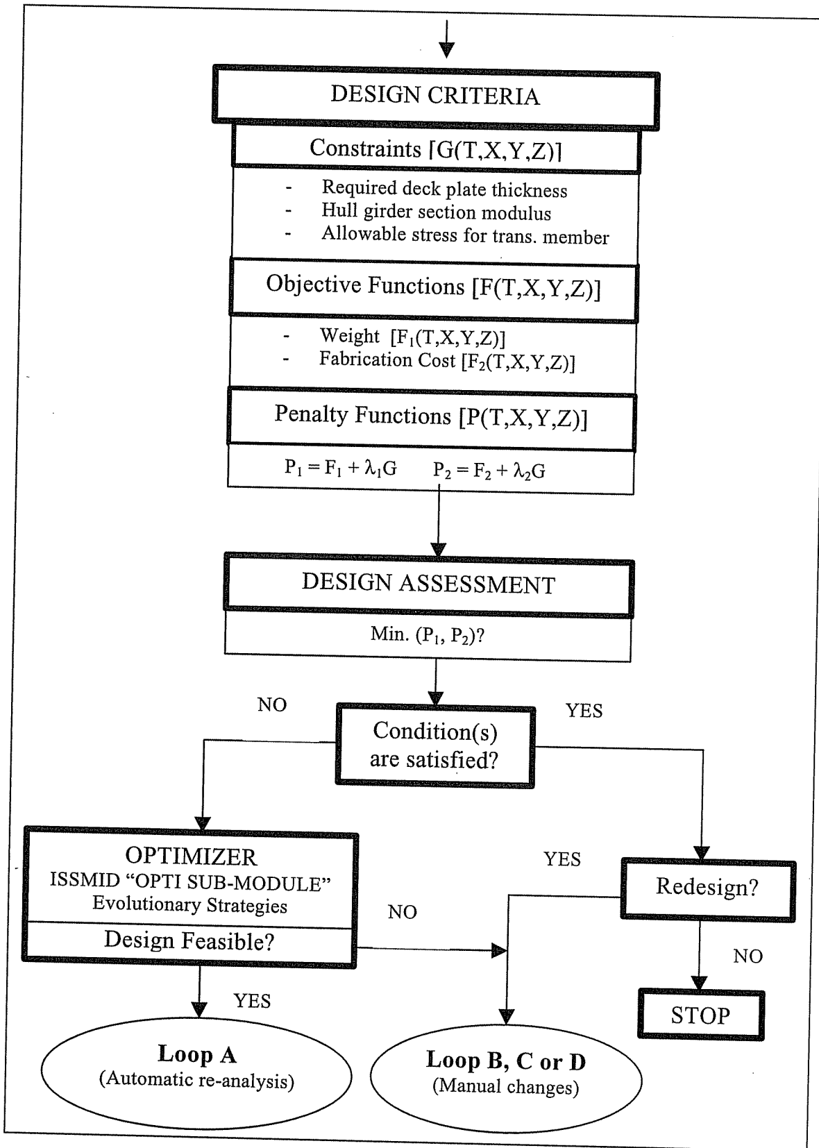
Figure 2b - ISSMID-T Framework (Part 2)
