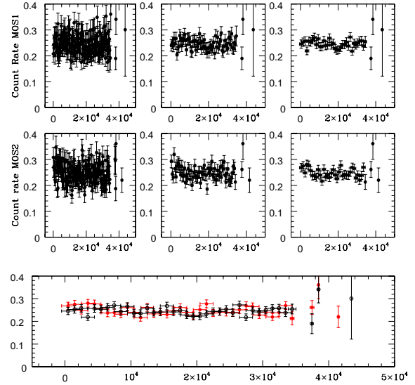
Fig. 1. X-ray lightcurves of \theta Car in the 0.2–5 keV band. Top: MOS1 lightcurves with time bins of 200, 500 and 1000s (from left to right). Middle: Same for MOS2. Bottom: Superposition of the MOS1 (open black symbols) and MOS2 (filled red symbols) lightcurves with 1ks-bins.
