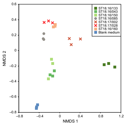
FIGURE 3 Non-metric multidimensional scaling (NMDS) ordination based on Bray–Curtis dissimilarities of the mVOC composition of seven bacterial strains investigated in this study ( n = 3 ; stress value = 0.158). The microbial volatile organic compound (mVOC) composition differed significantly between the bacterial strains and the blank medium (perMANOVA: F = 38.6 , p < .001 ). Symbol colours indicate the effect of the mVOC blends on the olfactory response of the primary parasitoid Aphidius colemani , that is, green = attractive, grey = neutral and red = repellent. Blue refers to the blank medium. Symbol shapes indicate the effect of the mVOC blends on the olfactory response of the hyperparasitoid Dendrocerus aphidum , that is, circle = attractive, square = neutral and cross = repellent
