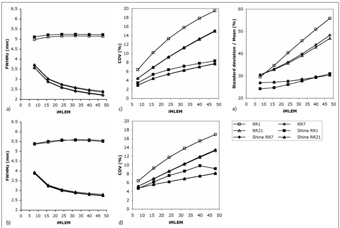
Fig. 3 Function of the number of equivalent MLEM iterations; reconstruction with 8 subsets, eventually SHINE pre-processing of the projections, and standard OSEM (RR1) or multi-ray OSEM with 7 (RR7) or 21 rays (RR21); a, c) no tilt; b, d) camera head tilted by 20° a, b) full width at half-maximum in the axial direction measured on line 3 of the 13-lines phantom c, d) coefficient of variation measured on the cylinder phantom e) standard deviation-to-mean ratio measured on a patient hot thyroid nodule
