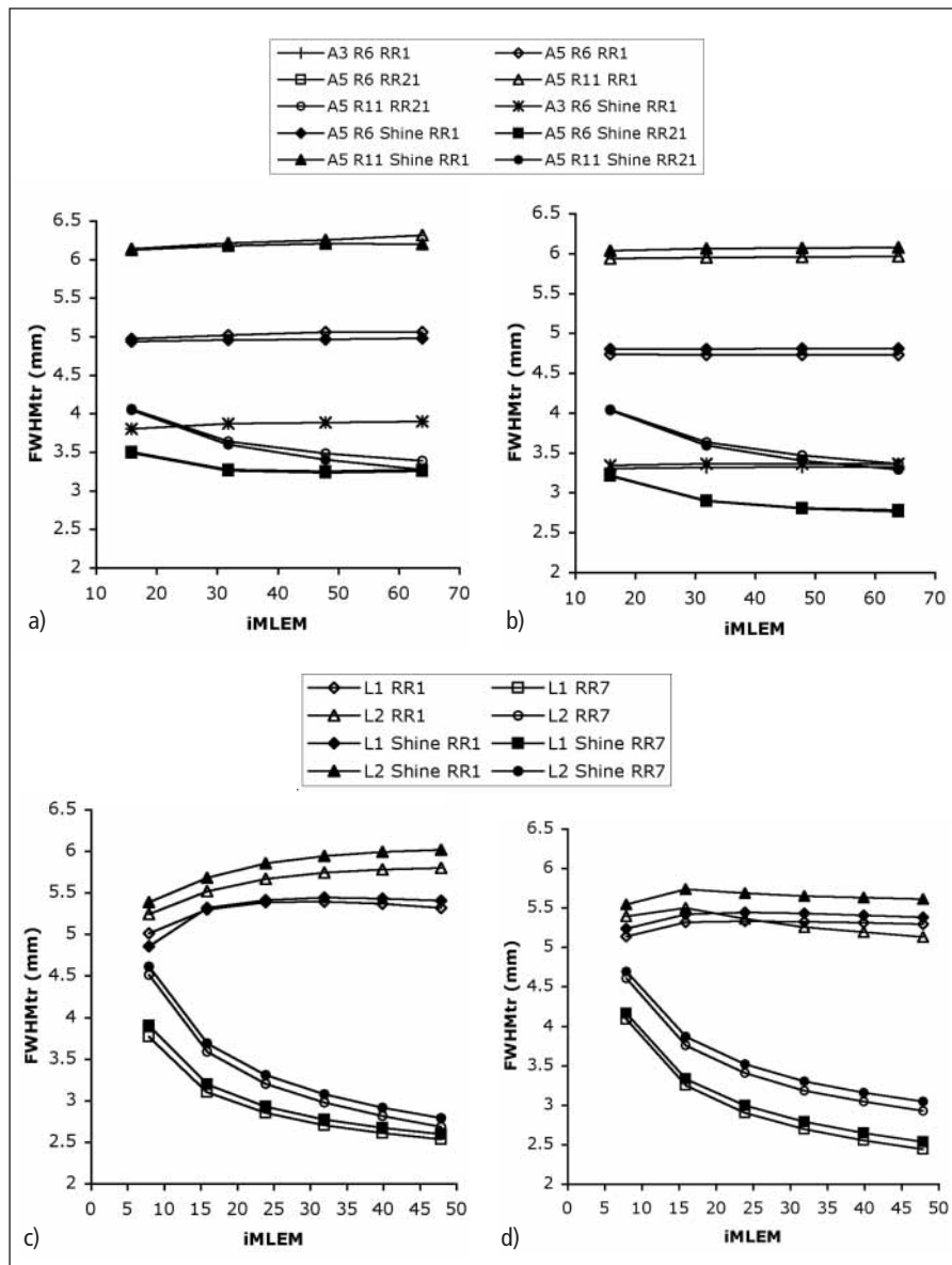
Fig. 2 Mean full width at half-maximum in the transverse plane; eventually SHINE pre-processing of the projections, and standard OSEM (RR1) or multi-ray OSEM with 7 (RR7) or 21 rays (RR21) a, b) as a function of the number of equivalent MLEM iterations; acquisition parameters: 360° orbit, 64 projections (A: pinhole aperture in mm; R: pinhole radius in cm); reconstruction with 16 subsets, a) line on camera rotation axis; b) line off axis. c, d) on line 1 (L1) or 2 (L2) of the 13-lines phantom as a function of the number of equivalent MLEM iterations; reconstruction with 8 subsets; c) no tilt, d) camera head tilted by 20°
