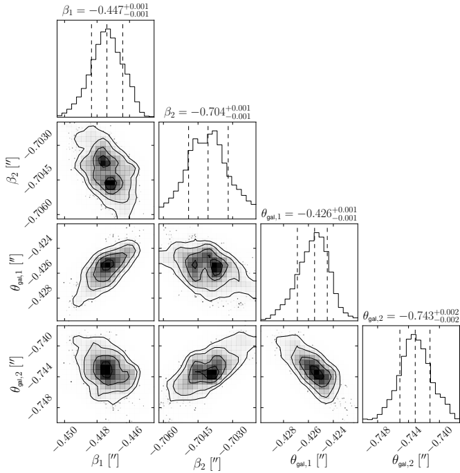
Fig. 4. Results of the MCMC sampling for the source position and lens galaxy centroid. The diagonal panels illustrate the posterior pdfs while the off-axis ones illustrate the correlation between the parameters. The vertical dashed lines locate the 16– and 84–th percentiles.
