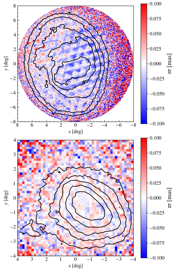
Fig. A.9. Measured parallaxes of stars in the LMC ( upper panel ) and SMC ( lower panel ). The banding associated with the Gaia scanning law is clearly visible.
