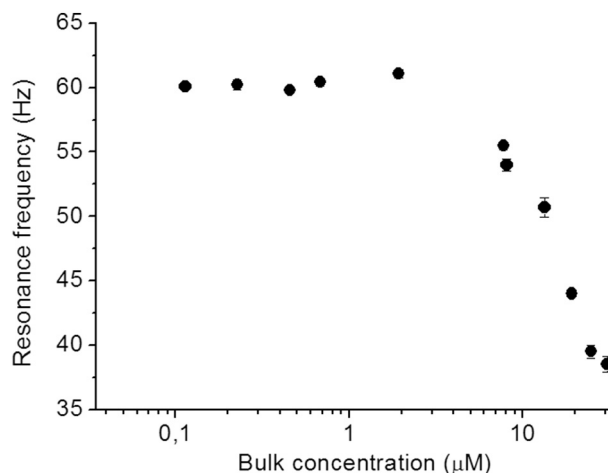
Fig. 4. Resonance frequency versus MR bulk concentration of a SQ drop of radius 0.7\ \text{mm} . The two regimes corresponding to the gas-state and the liquid-expanded state for the surface monolayer of MR at the SQ/water interface can be identified. Standard errors from the fitting procedure are reported.
