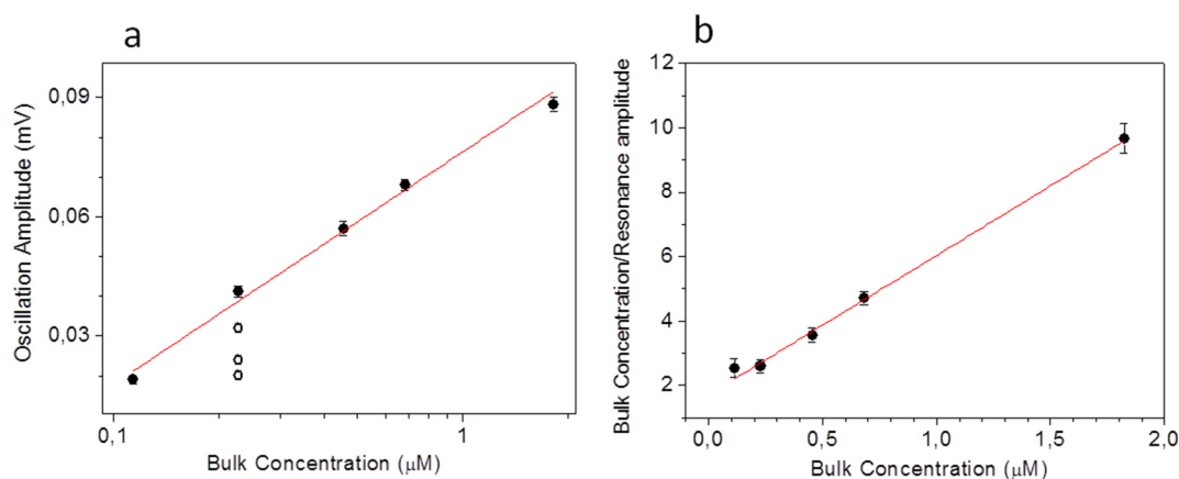
Fig. 5. a) Resonance amplitude versus MR bulk concentration, in the regime corresponding to the gas state for the interfacial monolayer. The highlighted slice shows successive transient values of the resonance amplitude (empty dots) after administration of the second surfactant dose (0.11 → 0.22 \mu\text{M} bulk concentration), soon after, 3 and 6 min after administration. The line corresponds to the fit to Temkin isotherm model of the steady state experimental values (full dots). b) The same experimental data are reported for testing the Langmuir isotherm model. Errors on the parameter of the fitting procedure are reported.
