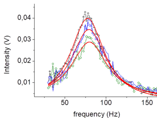
Fig. 3. Resonance amplitude increasing during MR adsorption at the interface of a SQ drop ( R = 0.6\ \text{mm} ) after addition of MR to the bulk, in the concentration range corresponding to the gas-state for the interfacial monolayer, surface pressure being unaffected. The three presented spectra are taken 5, 7 and 11 min after administration. Red lines are the Lorentzian fits.
