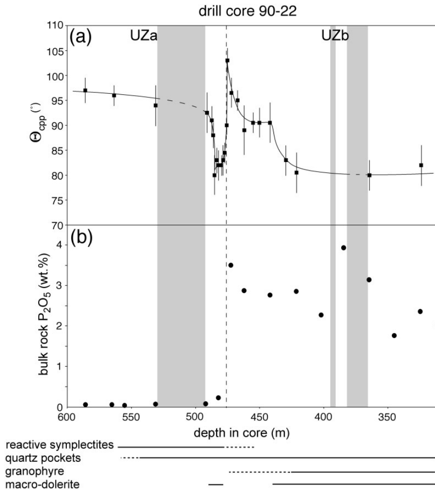
Fig. 5. (a) Variation of \Theta_{\text{cpx}} in drill core 90-22, from Holness (2015) . (b) The bulk-rock \text{P}_2\text{O}_5 concentration [data from Tegner et al. (2009) ]. The arrival of cumulus apatite is shown as the dotted line at 475 m depth in core. The vertical grey bands show the stratigraphic position and extent of late-stage dykes [no distinction is made between mafic and (the rarer and thinner) granophyric dykes]. The continuous lines beneath the graph denote regions of the stratigraphy characterized by different late-stage microstructural features (shown in Fig. 7 ); the dotted ends to these lines denote stratigraphic regions where each late-stage feature is present but rare.
