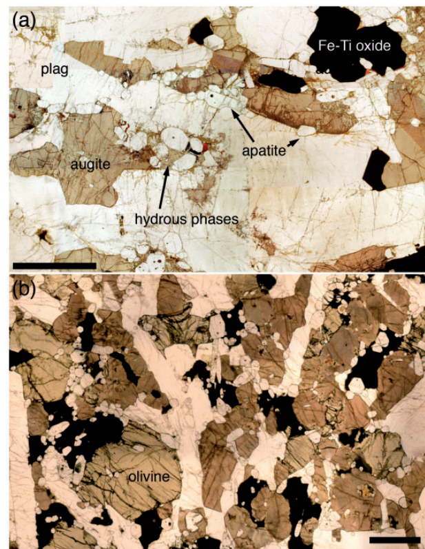
Fig. 10. (a) Photomicrograph of gabbro at 475.9 m depth in drill core 90-22: this is the lowest sample from 90-22 that contains abundant euhedral apatite grains. It should be noted how the apatite grains cluster in triangular spaces between plagioclase primocrysts, and are associated with late-stage, primary magmatic, hydrous minerals. Scale bar represents 2 mm. (b) Gabbro at 471.9 m depth in drill core 90-22. Here the apatite grains are more homogeneously distributed and are no longer clustered within spaces between primocrysts. Scale bar represents 2 mm.
