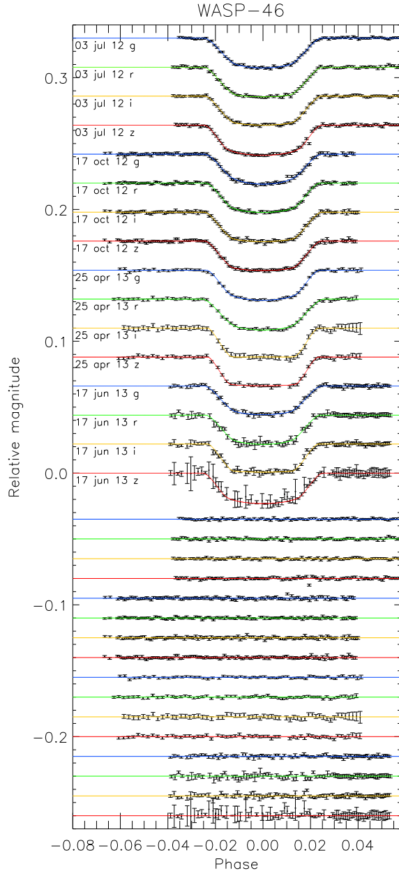
Figure 3. Phased light curves of four transits of WASP-46 observed with GROND. Each transit was observed simultaneously in four optical bands. As in Figs. 1 and 2 the light curves are compared with the best-fitting curves given by JKTEBOP, and the residuals from the fits are displayed at the bottom in the same order as the light curves. The curves are shifted along the y axis for clarity.
