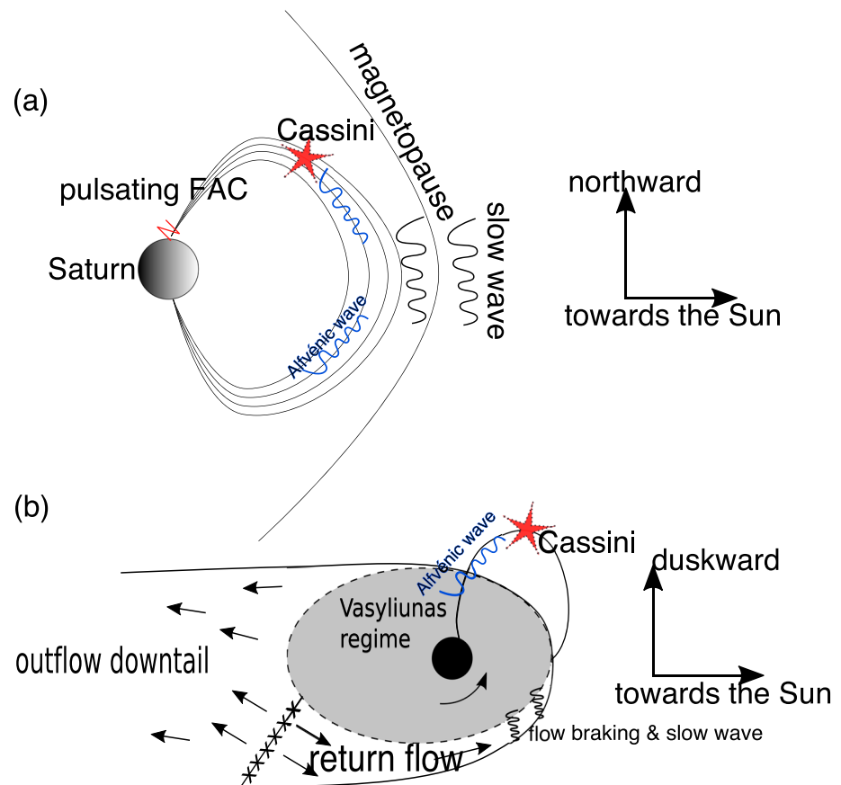
Figure 4. Illustration of two physical pictures for the generation of the plasma wave observed in this study. (a) Slow mode wave generated in magnetosheath propagates into magnetosphere and converts to Alfvénic wave that carries FAC to ionosphere and generate a transient aurora. (b) The return flow from the nightside Dungey cycle reconnection experiences a blockage in the equatorial plane, which generates slow mode compressional wave within the magnetosphere. The slow mode wave converts to Alfvénic wave and generate aurora intensification. The picture of flow cycle is adapted from Radioti et al. (2017) (originally from Southwood & Chané, 2016).
