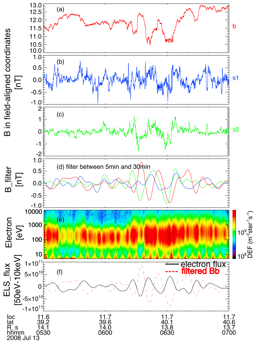
Figure 3. The results of wave analysis of in situ measurements. (a–c) Three components of the magnetic field in mean field-aligned (MFA) coordinate system. (d) The results of a band-pass filter (5 min to 30 min) of the three magnetic components (Figures 3a–3c). (e) Electron differential energy flux. (f) The total flux of the electron differential energy flux at energies between 50 eV and 10 keV. The red dashed line if the filtered the compressional component magnetic field as shown in Figure 3d.
