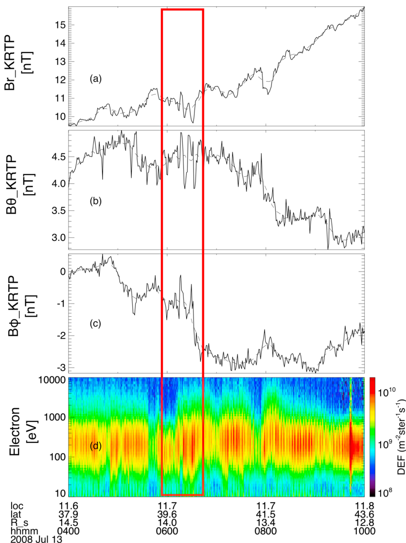
Figure 2. Overview of the in situ measurements from Cassini. (a–c) The components of magnetic field in Kronocentric Radial-Theta-Phi coordinates. (d) Electron differential energy flux from Cassini CAPS-ELS instrument. The red rectangle indicates the perturbations of magnetic fields and plasma corresponding to the auroral intensification.
