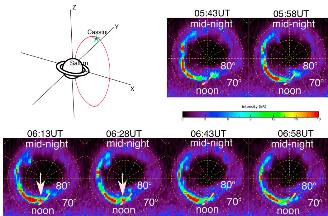
Figure 1. Aurora images on 13 July 2008 (DOY 195) from Cassini/UVIS instrument. Each image was obtained in a time window of \sim 10 min. The time displayed on the top of each image represents the start time of each window. The location of Cassini is presented on the top left of this figure. The location of the Cassini spacecraft was magnetically mapped to Saturn's polar region. The filled pink circle represents the foot point of Cassini at 0730 UT. The yellow dots show foot points of Cassini's trajectories between 12 July and 14 July 2008. The white arrows indicate the auroral intensification region.
