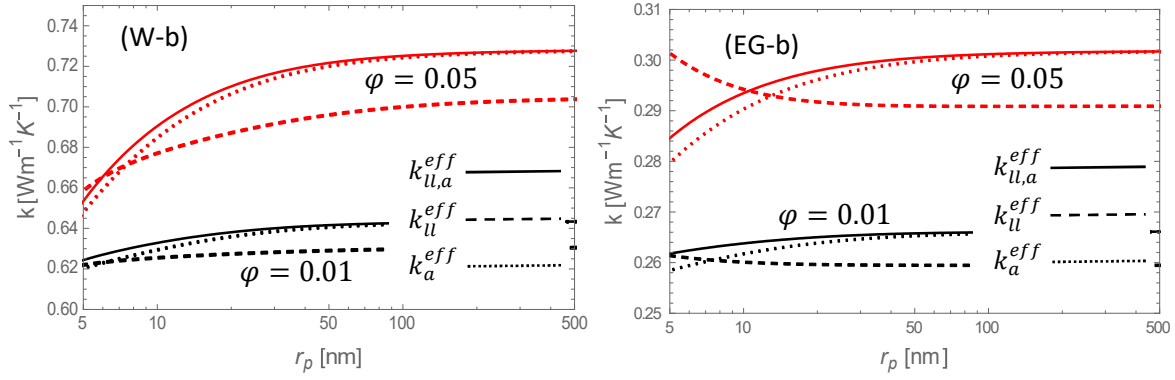
Fig. 5 Effective thermal conductivity k_{l,a}^{eff} (solid lines) compared to k_l^{eff} (dashed lines) and k_a^{eff} (dotted lines) versus the nanoparticle radius at volume fractions of 1% (lower curves) and 5% (upper curves), for (a) \delta = 1 nm and (b) \delta = 3 nm. The nanofluids consist of alumina nanoparticles in water (W) and ethylene glycol (EG).
