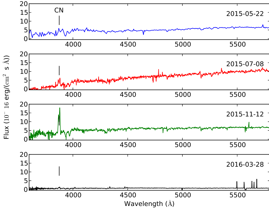
Figure 1. Examples of FORS2 sky-subtracted extracted spectra for four different dates: 2015 May 22, 2015 July 08, 2015 November 12, and 2016 March 28. Those spectra have been extracted out to 5". The vertical line indicates the wavelength of the CN emission.
