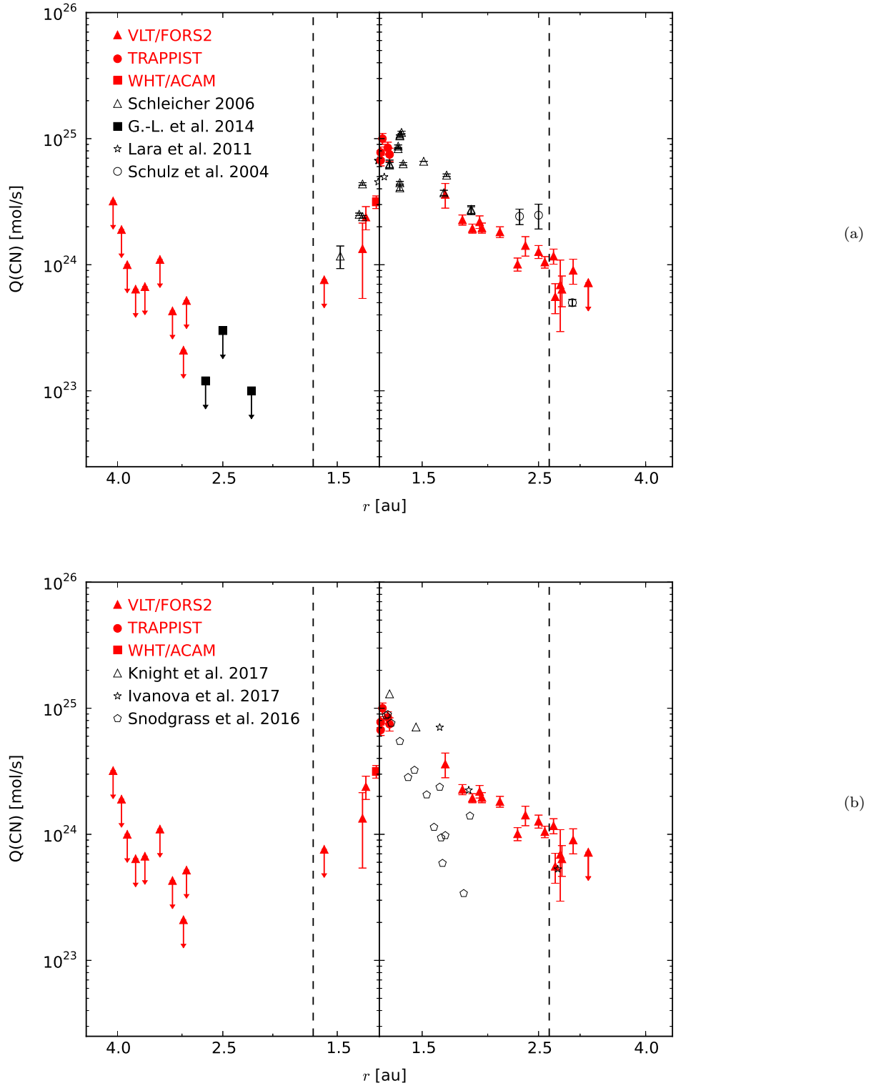
Figure 2. Pre- and post-perihelion evolution of comet 67P CN production rate. We include data obtained with VLT/FORS2 (red triangles), with TRAPPIST (red full circles), and with WHT/ACAM (red square). (a) We compare our results to measurements performed at previous perihelion passages (Schleicher 2006; Schulz et al. 2004; Guilbert-Lepoutre et al. 2014; Lara et al. 2011). (b) We compare our results to measurements performed with other instruments during this perihelion passage (Snodgrass et al. 2016a; Knight et al. 2017; Ivanova et al. 2017). The two vertical dashed lines indicate the equinox.
