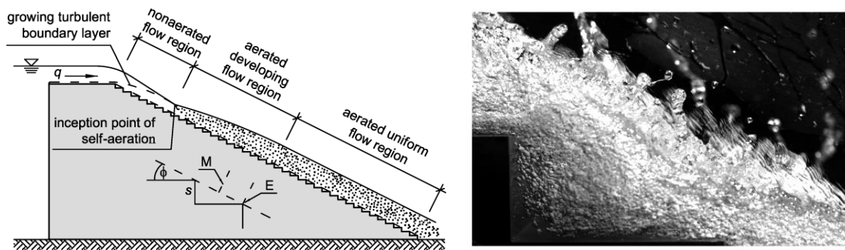
Figure 1. Sketch of flow regions over a spillway (left) and aerated flow at step 21 for q = 0.07 m 2 /s (right).
