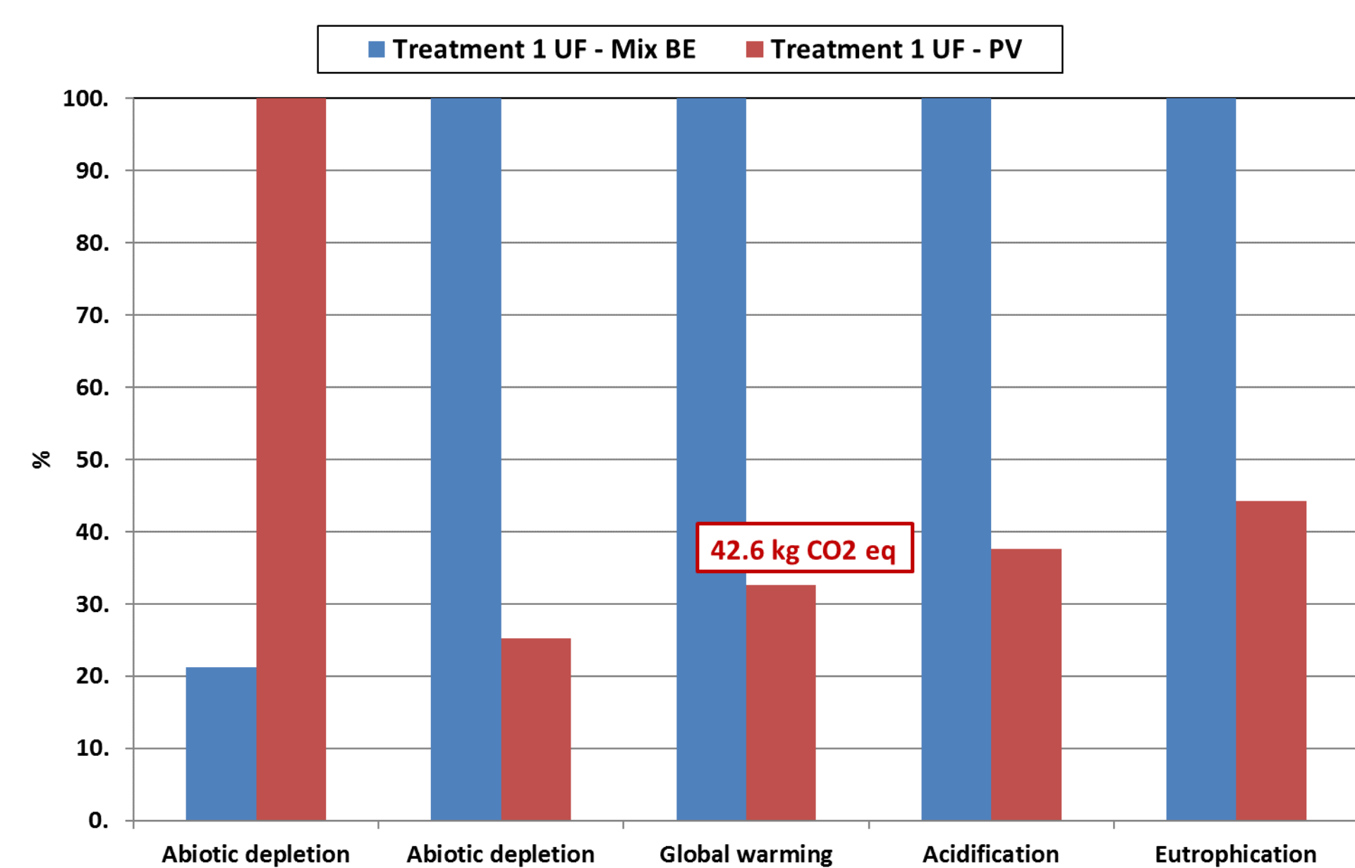
Figure 4. Comparison of the impacts of the treatment of 1 tonne of food waste in an EC100 supplied with Belgian electricity mix (in blue) or by PV (in red) – characterisation CML-IA
