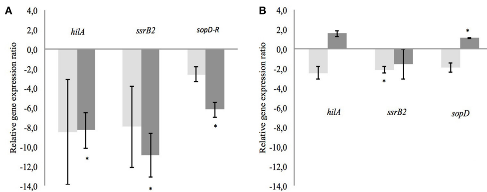
FIGURE 4 | Effect of CFSM from MRS2 G medium (A) and MRS2-3' SL medium (B) fermented by B. bifidum (light gray) and B. crudilactis (dark gray) on virulence gene expression of S. Typhimurium after 4 h of incubation. Gene expression ratios of S. Typhimurium were normalized to the expression of the housekeeping gene gmk and compared with those of the unfermented media. Negative values represent down-regulation of genes and positive values represent up-regulation of genes. * P \leq 0.05 .
