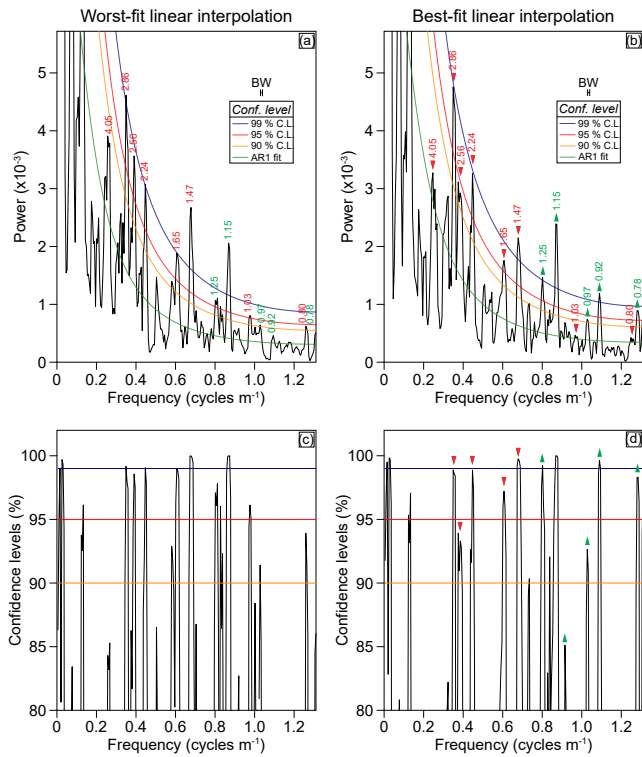
Figure A2. Comparison of spectra of the resampled time series for the worst-fit case (a and c) and for the best-fit case (b and d). Spectra (a) and (b) are calculated using the 2\pi multi-taper method with confidence levels calculated using the method of Mann and Lees (1996) with a Tukey’s end-point rule (Meyers, 2014). Panels (c) and (d) show the confidence levels compared to a red noise. Red arrows indicate the frequency at which powers and confidence levels decrease from the worst-fit case to the best-fit case. Green arrows display the opposite case.
