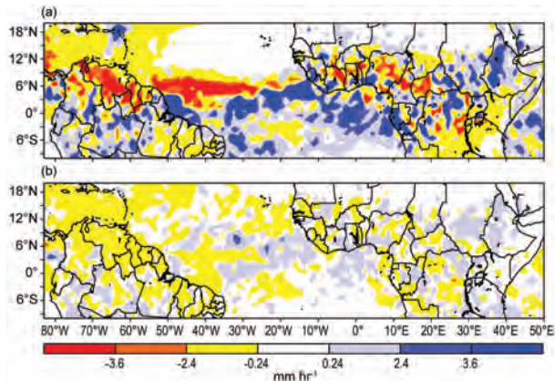
FIG. 4.17. TRMM tropical South America precipitation anomalies ( \text{mm h}^{-1} ) with respect to 1998–2013 for (a) May 2014 and (b) Jan–Dec 2014.
