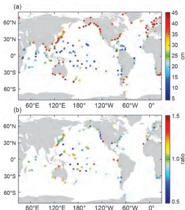
FIG. 3.28. (a) Annual maximum sea level during 2014 computed from the mean of the 2% highest daily values relative to the 2014 annual mean. (b) 2014 annual maximum from (a) divided by the time-averaged annual maximum at each station with at least 20 years of data.
