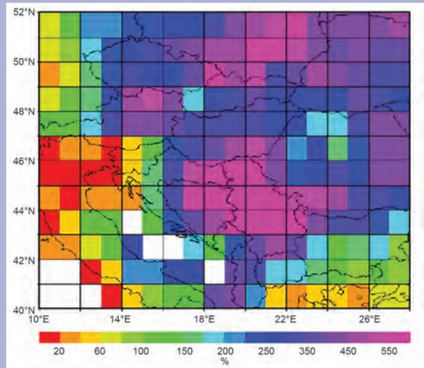
Fig. SB7.4. Relative anomaly of precipitation (%) for southeast Europe on 13–18 May 2014 based on a long-term mean for a 6-day period in May. (Source: GPCP.)
