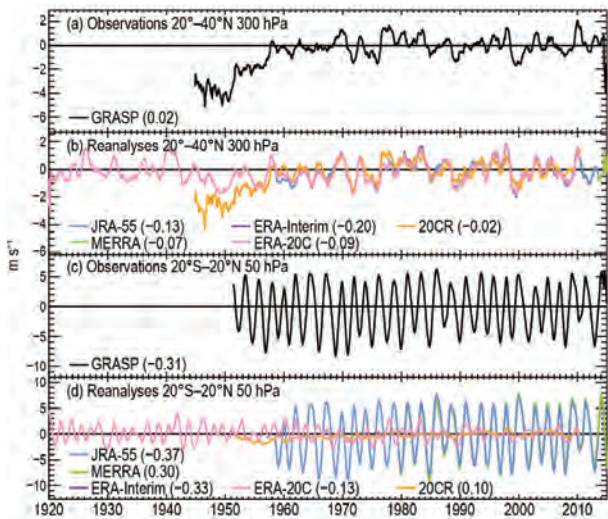
FIG. 2.32. Time series of zonal mean U-wind component ( \text{m s}^{-1} ): (a),(b) in belt 20^{\circ}\text{--}40^{\circ}\text{N} at 300 hPa and (c),(d) in the tropical belt 20^{\circ}\text{S--}20^{\circ}\text{N} at 50 hPa, calculated from ERA-Interim, MERRA, and JRA-55 reanalyses, 20CR, ERA-20C (Poli et al. 2013) surface data only reanalyses (20CR subsampled to where balloon data exist) and pilot balloon/radiosonde winds (GRASP). Values in legend are linear trends in interval 1981–2010 in units \text{m s}^{-1} \text{decade}^{-1} . Note that positive (negative) changes in the zonal wind speed imply an increase in westerlies (easterlies). Data have been smoothed using a 12-point boxcar filter.
