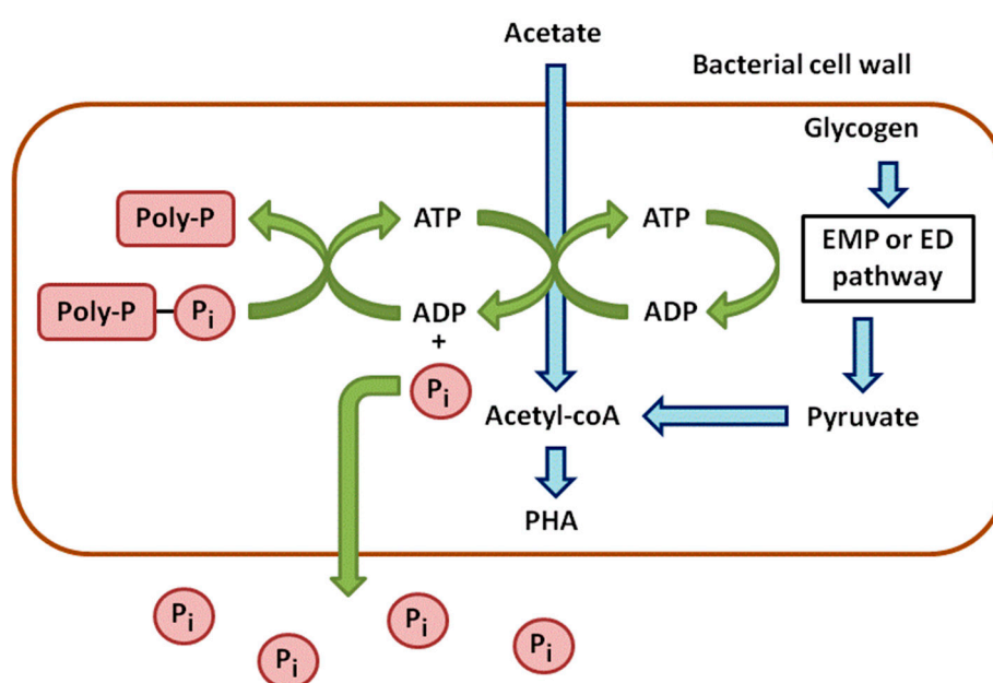
Figure 1. Anaerobic metabolism of phosphorus in phosphate accumulating bacteria.
