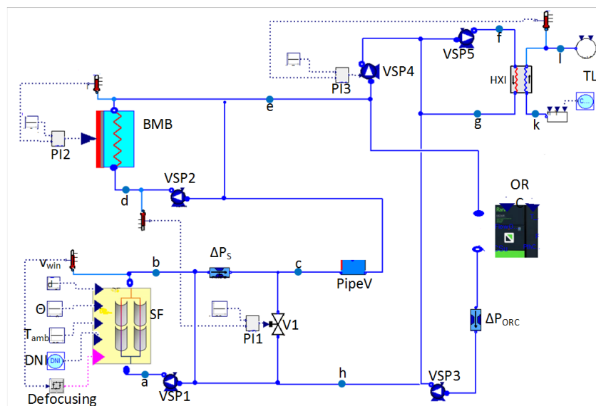
Fig. 2 Modelica model of the system from the Modelica/Dymola GUI.
