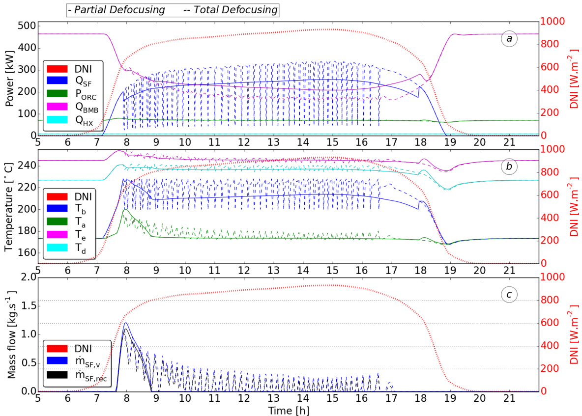
Fig. 4 Dynamic simulation results of the whole plant model during a reference summer day in Cacares, Spain. The dashed line represents the results for a solar field control strategy based on a total defocusing, the solid line for a partial defocusing. (a) Thermal power delivered by the solar field, the biomass, the ORC evaporator and the HX oil/water evaporator (b) Temperature values in key points of the system (c) Mass flows of the solar field bypass and recirculation system.
