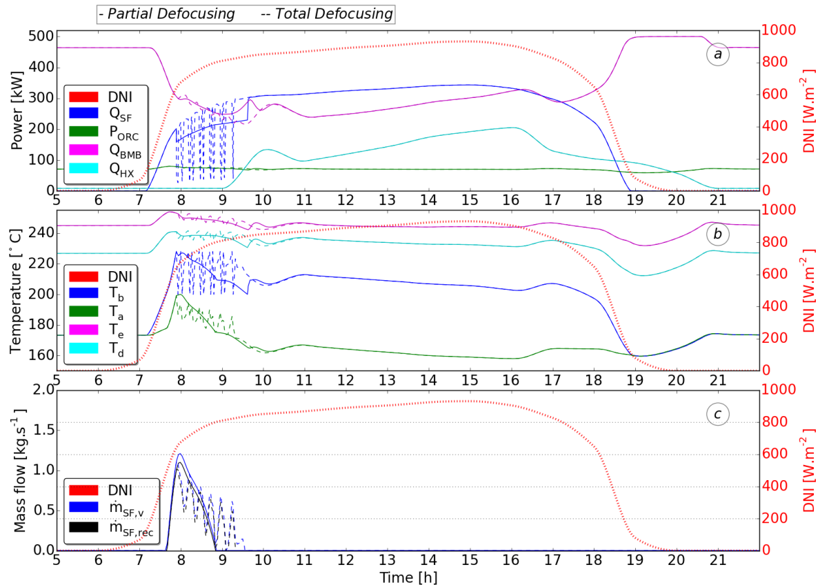
Fig. 5 Dynamic simulation results of the whole plant model during a reference summer day in Caçares, Spain with variable required thermal power. The dashed line represents the results for a solar field control strategy based on a total defocusing (TD), the solid line for a partial defocusing (PD). (a) Thermal power delivered by the solar field, the biomass, the ORC evaporator and the HX oil/water evaporator (b) Temperature values in key points of the system (c) Mass flows of the solar field bypass and recirculation system.
