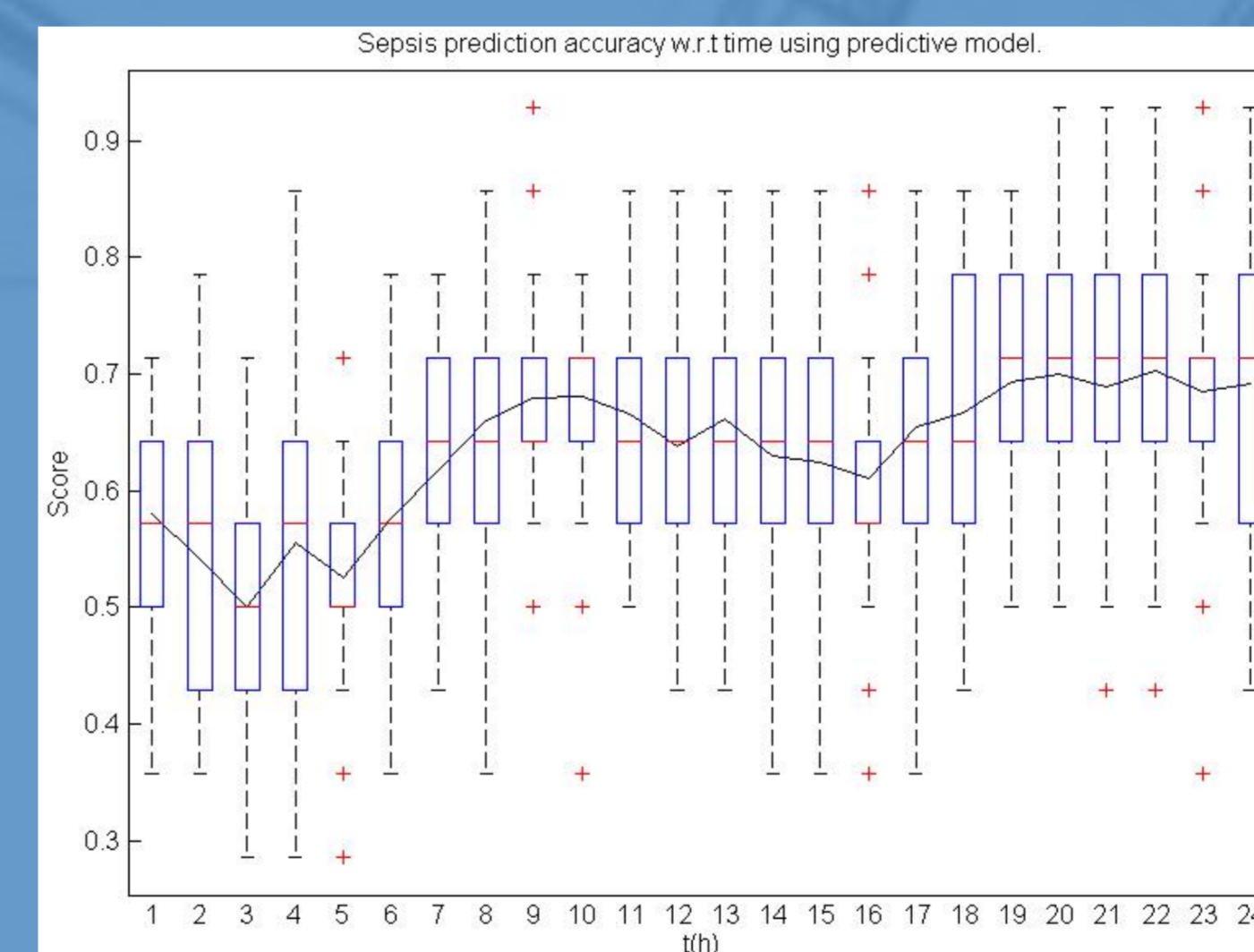
FIGURE V. SEPSIS PREDICTION ACCURACY OF THE PREDICTIVE MODEL W.R.T. TIME.
