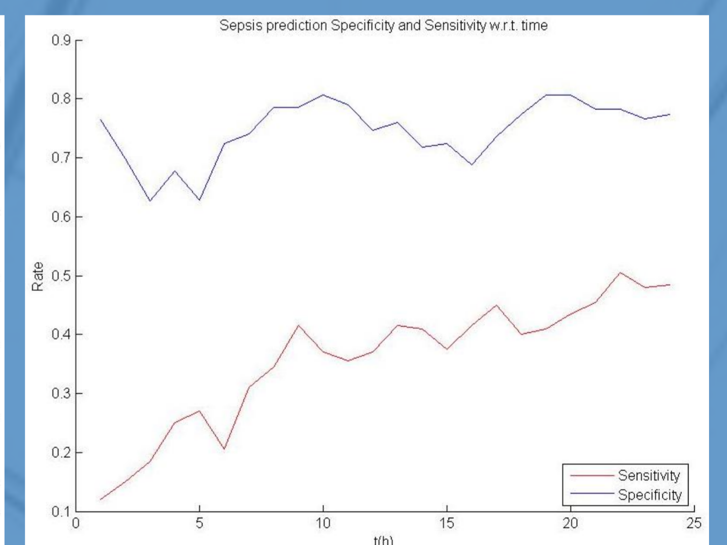
FIGURE VI. SEPSIS PREDICTION SENSITIVITY AND SPECIFICITY OF THE MODEL W.R.T. TIME.
