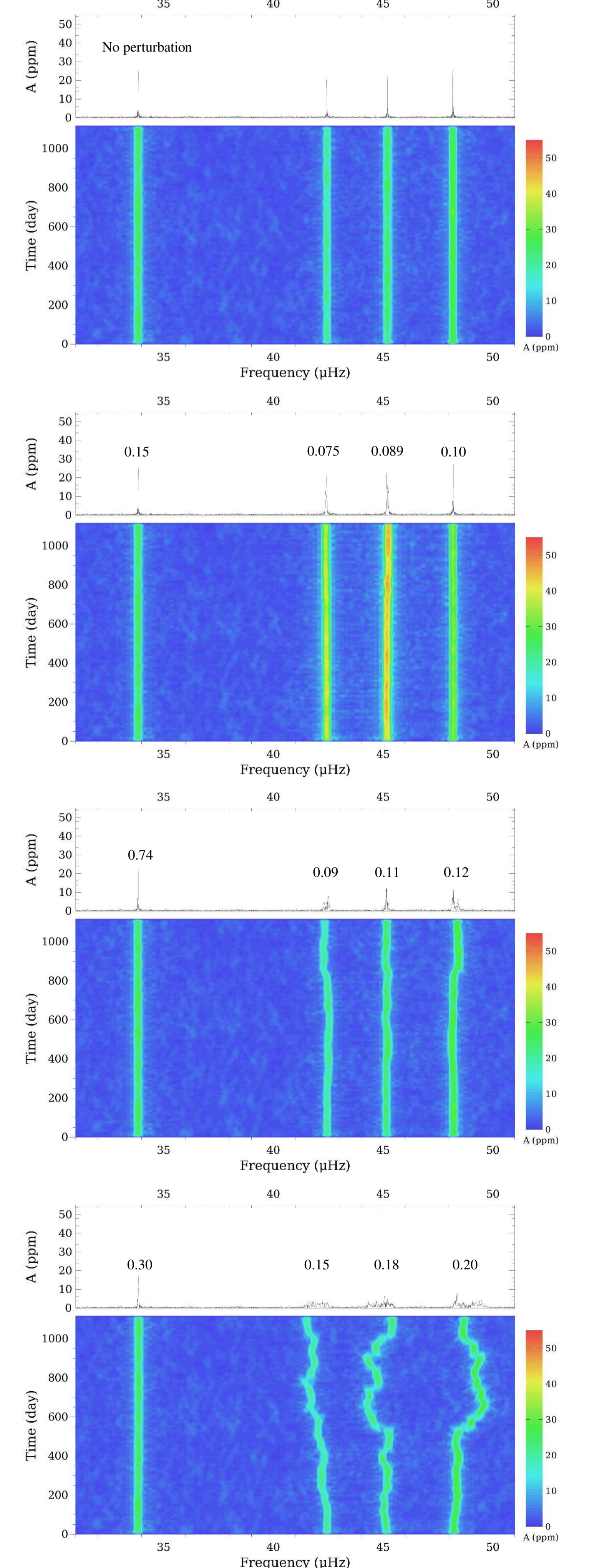
Figure 3 – Analysis of simulated low noise lightcurves computed with the N-body integrator REBOUND (Rein & Liu, 2012) for a configuration of 4 planets with different masses (the values, in earth mass, given above each peak). The simulations cover 1115 day with a sampling time of 60 s (hence similar to the available Kepler data). The top panel represents the case with no gravitational perturbation (purely periodic orbits) and mass is globally increased from top to bottom, up to a case where the system becomes dynamically unstable.
