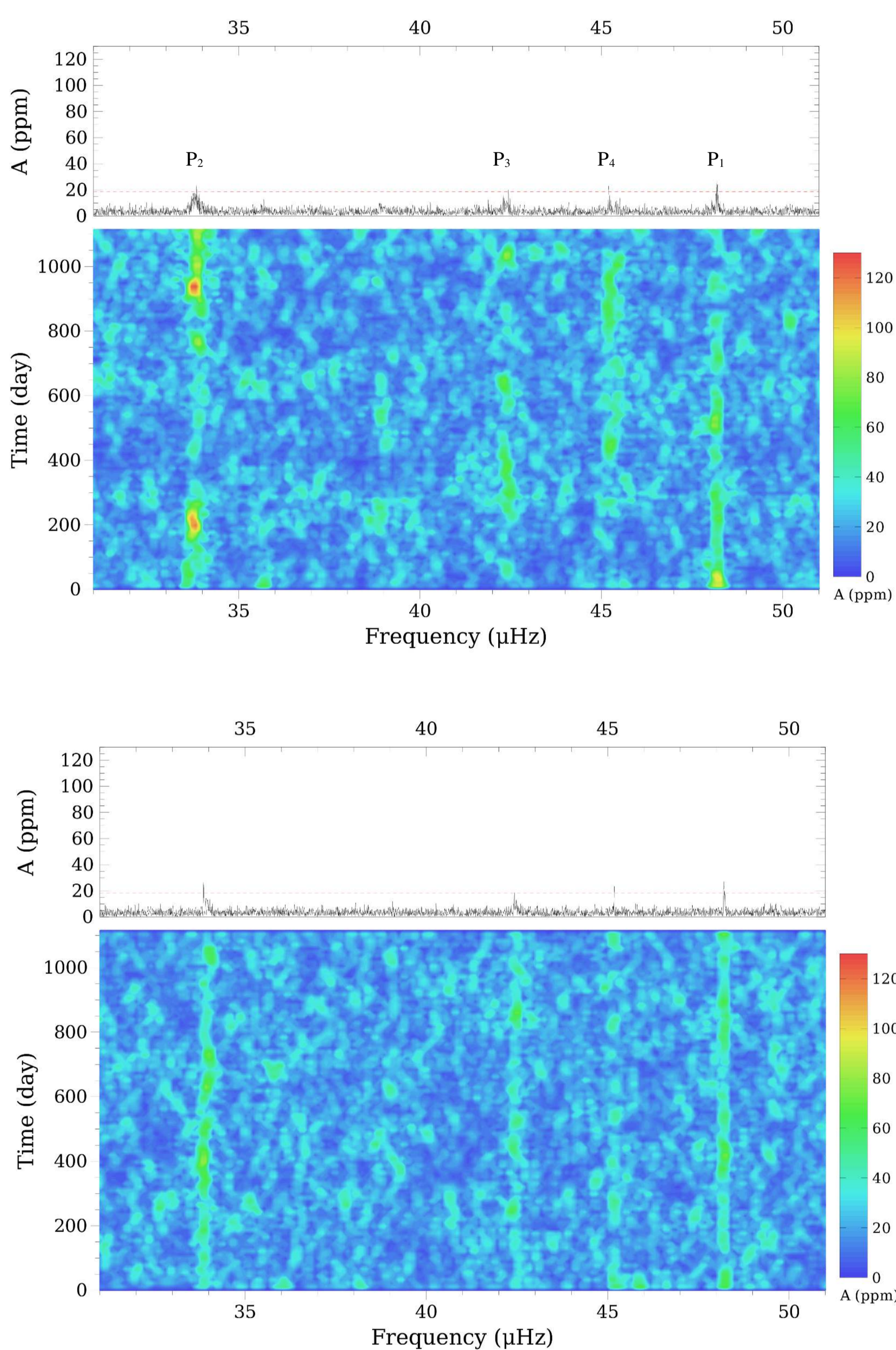
Figure 1 – Analysis of 1115 days (Q5 to Q16) of short cadence Kepler photometry obtained on KIC 05807616, with a close-up view of the 32 – 49 \mu\text{Hz} frequency range where planetary signatures are found. Top panel : High resolution Lomb-Scargle periodogram of the full lightcurve. The red dotted line indicates the secure detection threshold (5.6 \sigma ; see Figure 2 ). Bottom panel : Time-Frequency diagram built from sliding Lomb-Scargle periodograms using a 56 day wide window moved by steps of 11 days along the lightcurve.
