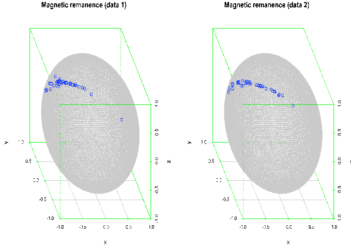
Figure 1: Measurements of remanent magnetization in red slits and claystones made at 2 different locations in Australia
