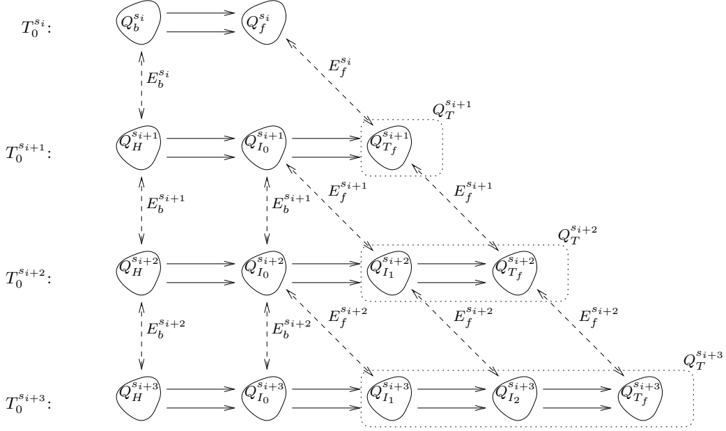
Fig. 1. Incrementally-growing sequence of transducers.
