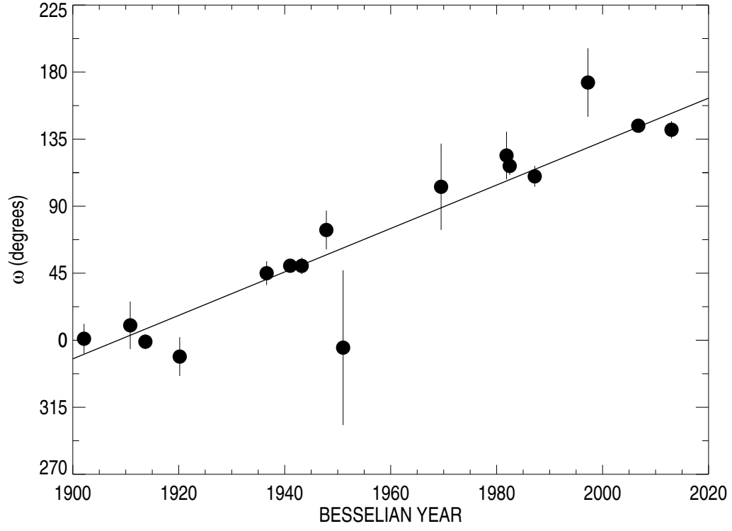
Fig. 6.— Apsidal motion of \delta Ori. A weighted linear fit to the published values (Harvey et al. 1987, H02, M10) yields a measurement of \dot{\omega} = (1.45 \pm 0.04)^\circ\text{yr}^{-1} .
