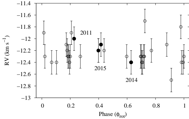
Figure 6. Radial velocity measurements show no trend with rotational phase. The filled circles indicate the values obtained in 2011, 2014 and 2015 and show that they are not significantly different from those from 2013 (open circles).
