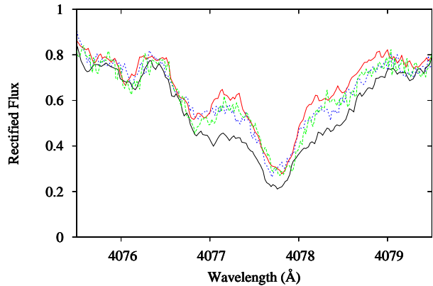
Figure 8. Variations in the profile shape of the Sr II 4077.7Å line with rotational modulation phase. The solid black line was taken at \phi_{\text{rot}} = 0.978 , the solid red line at \phi_{\text{rot}} = 0.597 . The dashed green and dotted blue lines were taken at \phi = 0.771 and \phi_{\text{rot}} = 0.227 , respectively.
