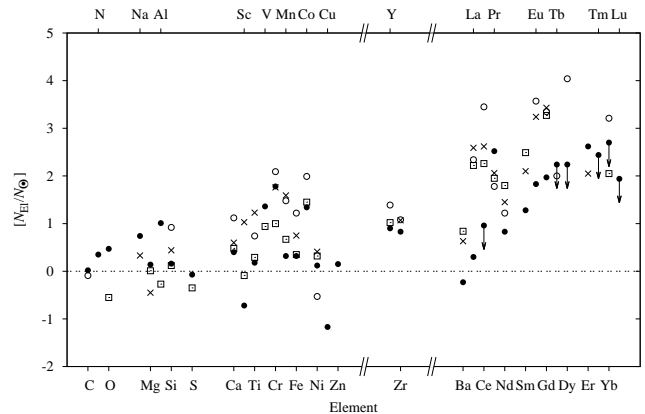
Figure 12. Abundance patterns for KIC 4768731 (filled circles), HD 177765 (open circles), HD 116114 (open squares) and \beta CrB (crosses). Upper limits are indicated by downward pointing arrows. Abundances are given relative to the Solar values from Asplund et al. (2009).
