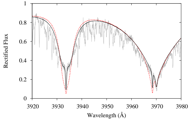
Figure 7. The Ca H and K lines in the FIES spectrum (grey line) taken on 2013 August 6 shows the distinctive pointed core due to element stratification. The solid line shows a synthetic line profile created using a step-shaped stratified abundance profile, while the red dashed-line shows a normal non-stratified synthesis.
