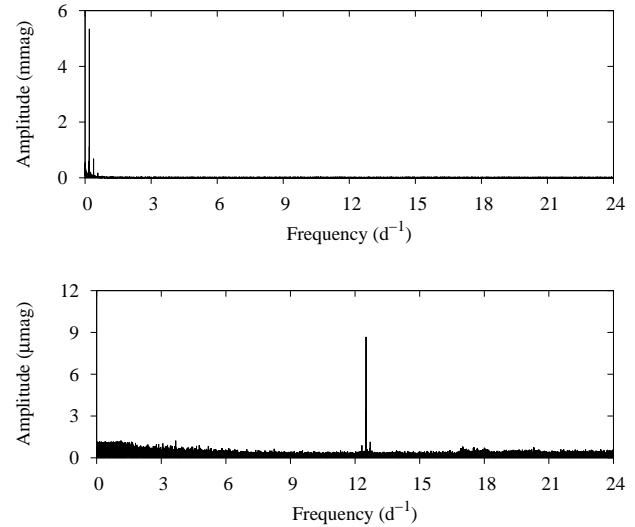
Figure 3. Top panel: An amplitude spectrum for the Q1 to Q17 Kepler long cadence data out to nearly the Nyquist frequency where only the low-frequency rotational variations can be seen, as a consequence of the scale. Bottom panel: An amplitude spectrum after a high-pass filter has removed the low-frequency variation showing the Nyquist alias of the 61.45\text{-d}^{-1} pulsation frequency triplet. Note the three orders of magnitude change in the ordinate scale from mmag in the top panel to \mu\text{mag} in the bottom panel.
