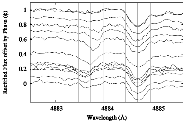
Figure 9. Changes in line profile strength and shape with rotational phase for the Y II line at 4883.7 Å. The rectified spectra have been offset so that their continuum levels correspond to their rotational phases. The nearby Cr II line at 4884.6 Å shows little shape variation with phase. The vertical black and grey lines indicate the line centres and the \pm 15 \text{ km s}^{-1} v \sin i widths, respectively.
