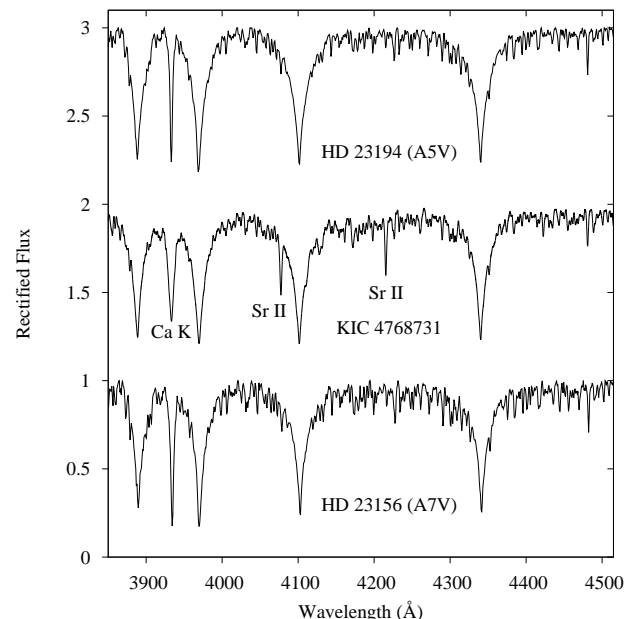
Figure 1. Spectrum of KIC 4768731 compared to the A5 V and A7 V MK standards. Note the prominent Sr II lines at 4077\text{\AA} and 4216\text{\AA} and the abnormal Ca II K line. The spectra have been offset for clarity.
