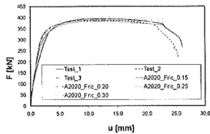
Figure 7 – Comparison of results using different friction coefficient.
