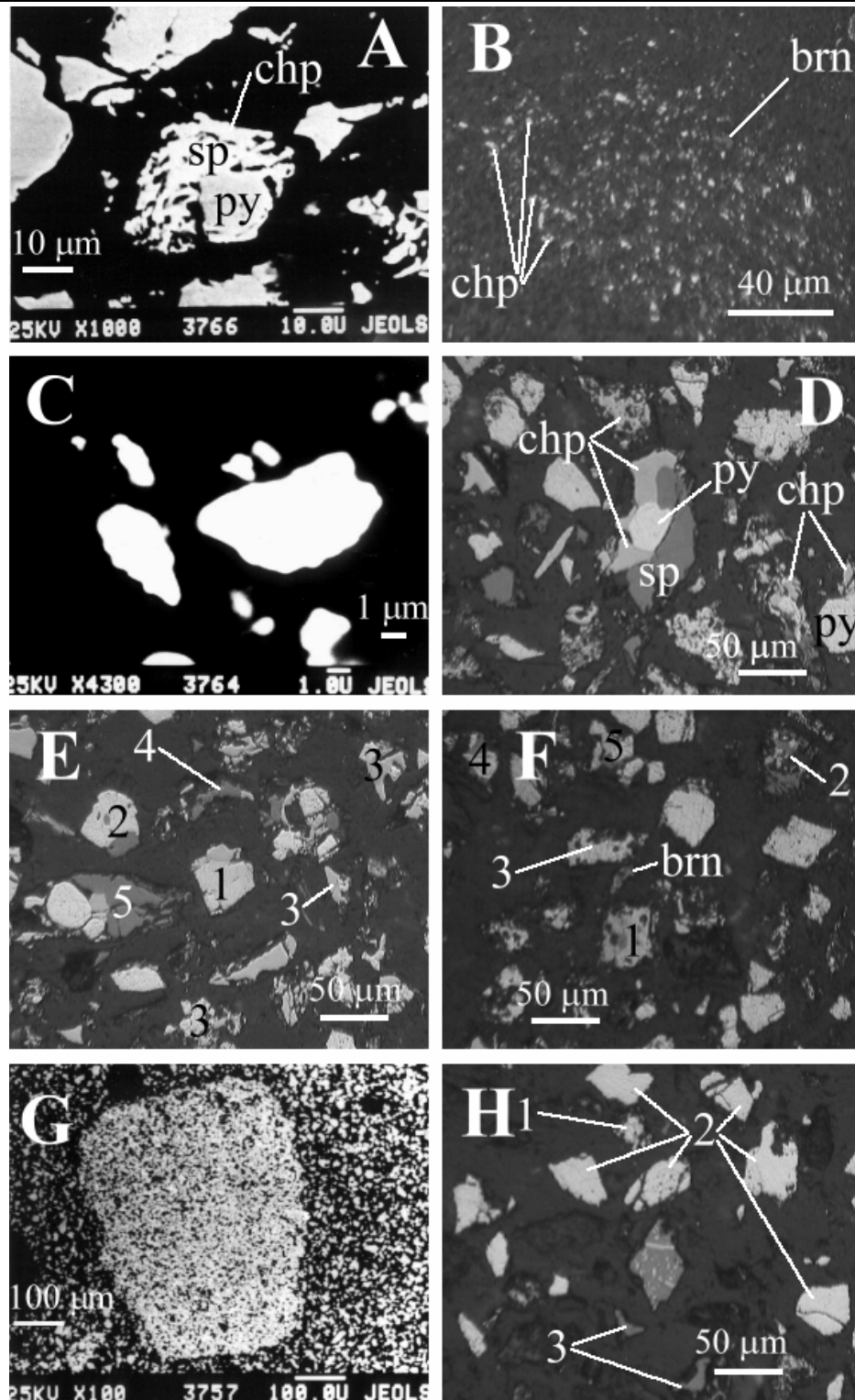
Fig. 2. Microphotographs (SEM and polarised reflected light).
