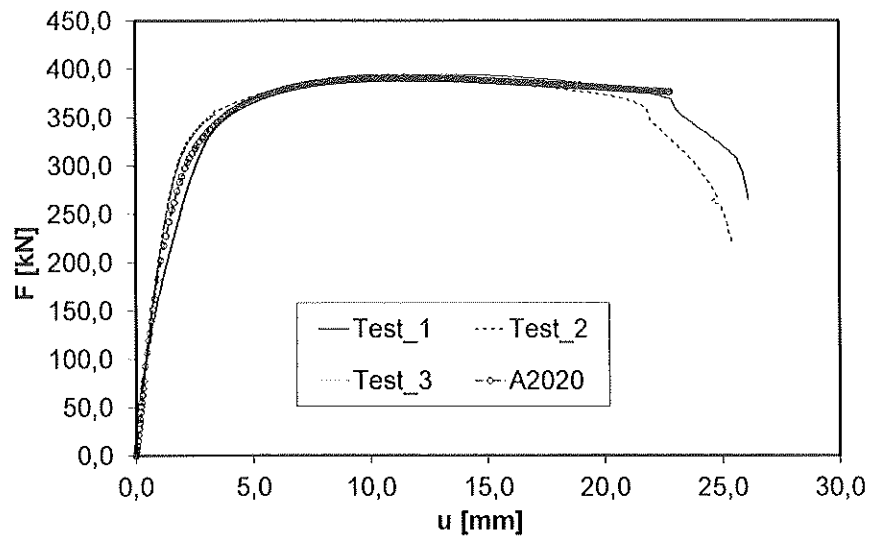
Figure 8 – Simulation of A2020 specimen [4] and comparison with tests.
