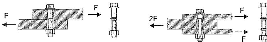
Figure 1 –Single and double overlap connections.
