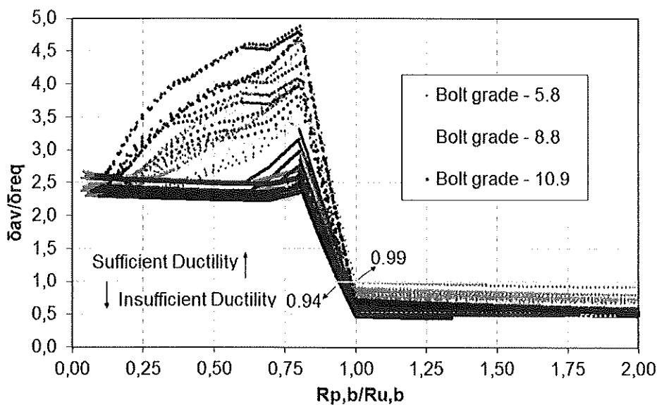
Figure 14 – Parametric analysis results.
