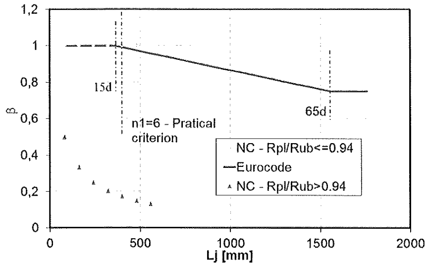
Figure 15 – Comparison with the Eurocode 3 criterion.
