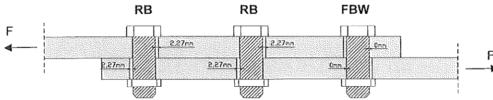
Figure 4 – Connection layout considering the presence of imperfections.
