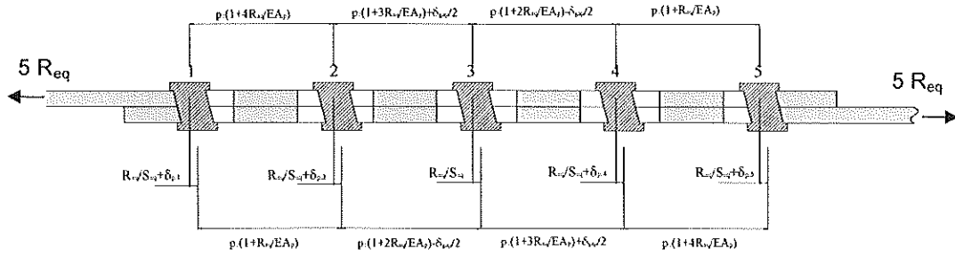
Figure 10 – Connection with 5 bolt rows.
