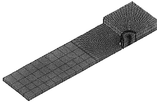
Figure 7 – Model with cover plate.
