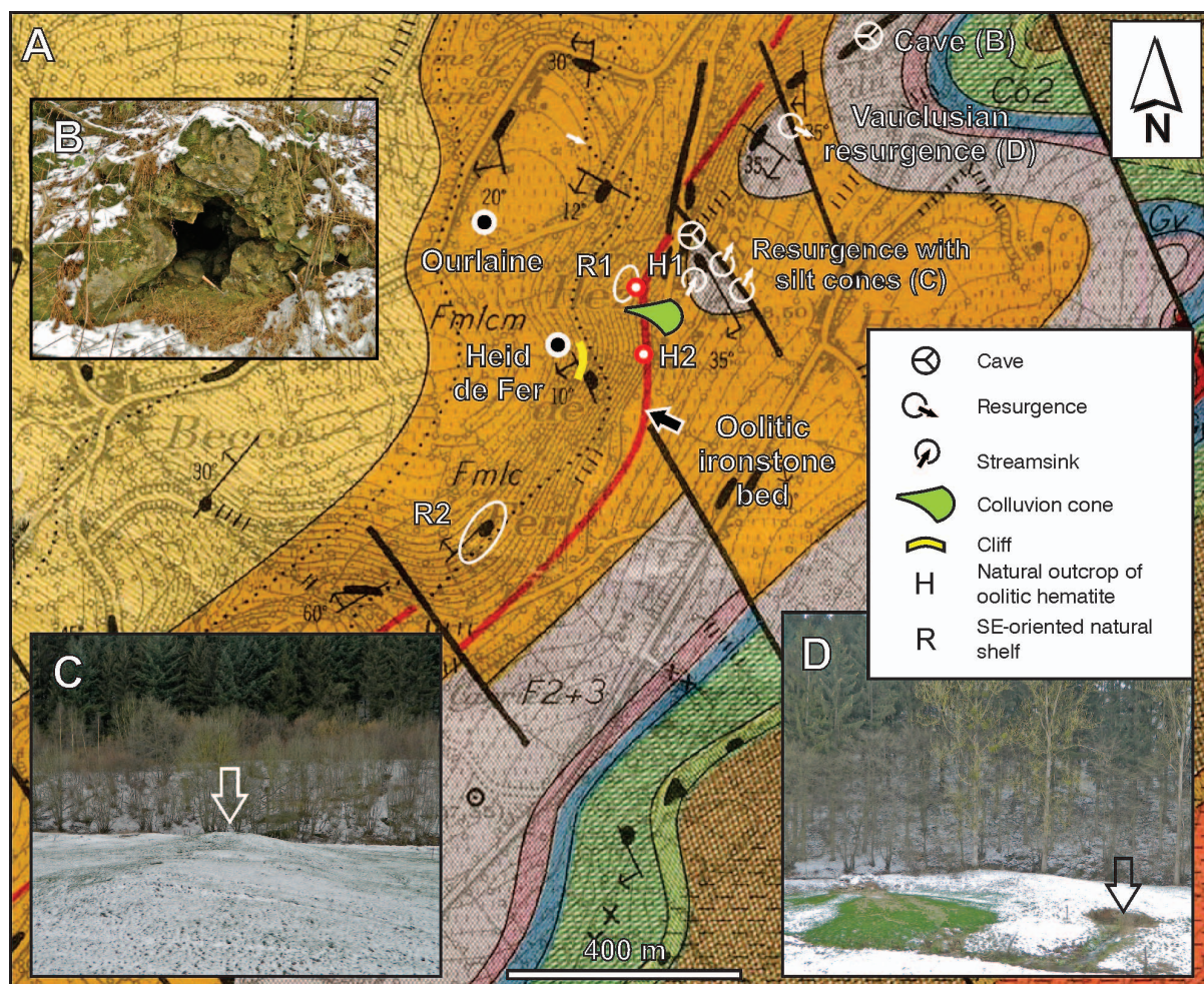
Fig 2 – Excerpt of the Louveigné-Spa geological map (Fourmarier, 1958) focused on the Heid de Fer and Ourlaine sites (Thûron valley). The shoulders R1 and R2 are located halfway up the steep shaly slope of the Heid de Fer. R1 is developed in contact with the horizon of oolitic ironstone H1 (base of Hodimont Formation). B: collapsed SE-oriented cave (limestone of the Lustin Formation), Thûron valley (hammer size: 0.5 m); C: cone of soft sediments (silts); D: Vaucclusian resurgence. Abbreviations : Fm2a: Montfort Formation (sandstones); Fm1cm: Souverain-Pré Formation (nodular limestones); Fm1c: Esneux Formation (sandstones and siltstones); Fm1ba: Lambermont and Hodimont formations (shales, siltstones); F3: Aisemont Formation (shales and limestones); F2: Lustin Formation (limestones); F1: Le Roux Formation (limestones, dolostones); Gv: Névremont Formation (limestones); Co1 & Co2: Pepinster Formation (shales, sandstones and conglomerates); E3 + E2: Wépion and Acoz formations (sandstones and quartzites).
