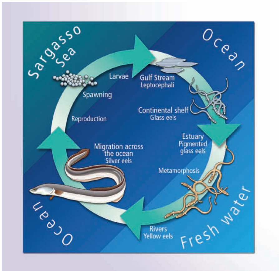
Migratory cycle of a catadromous, amphibiotic migratory species (European eel).
