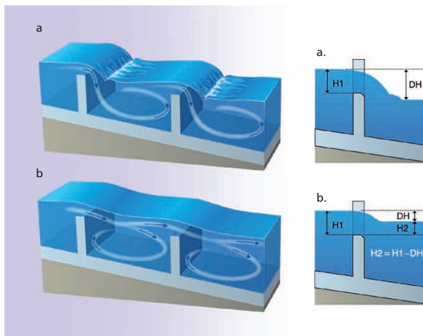
Types of flow over partitions in pool-type fish passes. (a) Plunging jet, (b) skimming flow.
