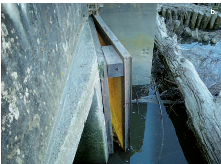
Examples of tidal structures left partially open or chocked open to enable passage upstream. (a) Gates held open at the Saubusse structure on the Adour River, (b) tide gates chocked open in the Arcins marshes.
