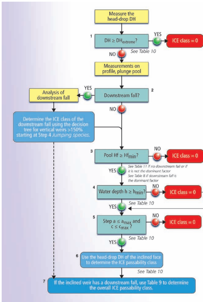
Decision tree to determine ICE passability classes for inclined weirs (slope ≤150% (56°)).
