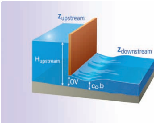
Parameters used to calculate a free gate flow.
