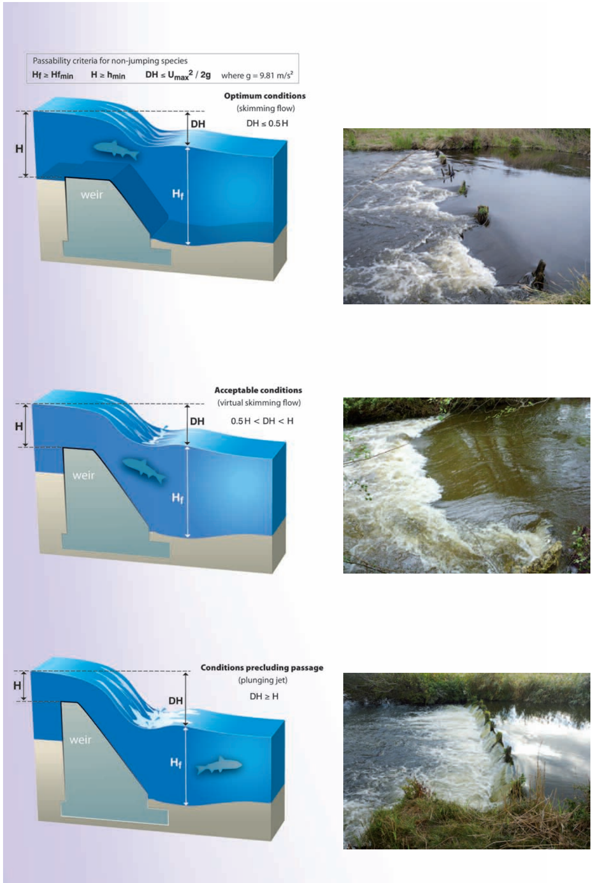
Types of jets and passage conditions for non-jumping species confronting a vertical or subvertical obstacle (slope >150% (56°)). (a) Skimming flow, (b) virtual skimming flow, (c) plunging jet (waterfall).
