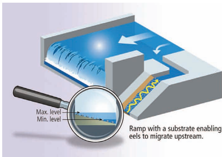
Diagram of a fish pass for eels supplied directly with upstream water.
