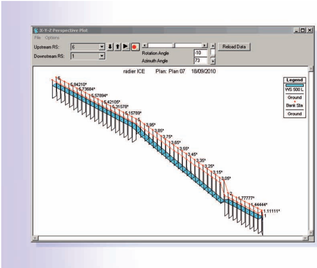
Graphic presentation of hydraulic modelling using the HEC RAS software.
