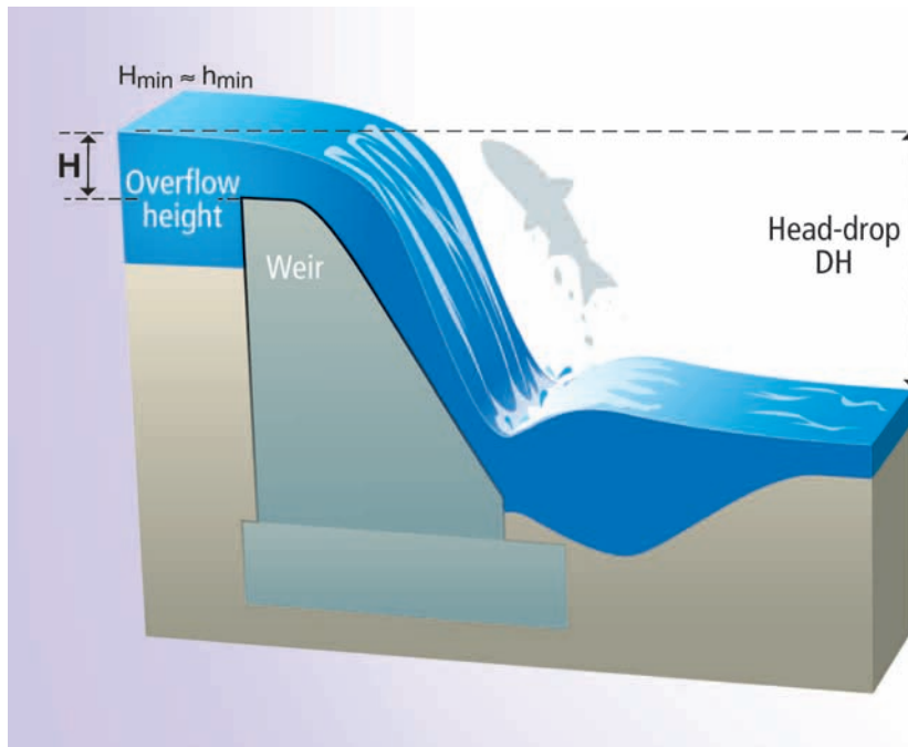
Minimum overflow height H_{\min} over an obstacle required by jumping species to ensure sufficient depth on arrival and effective passage upstream.
