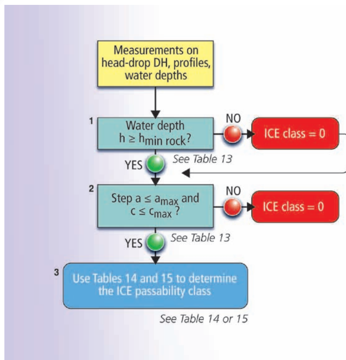
Decision tree to determine ICE passability classes for rock weirs.
