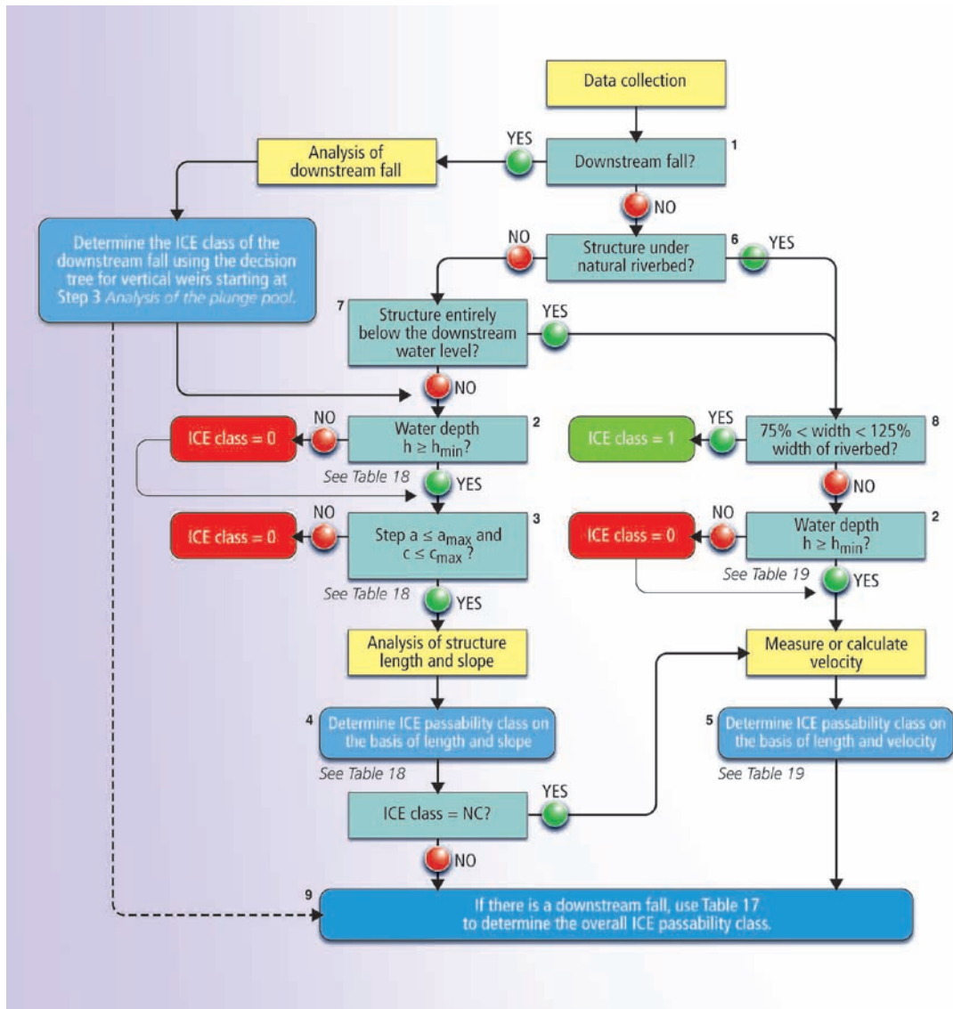
Decision tree to determine ICE passability classes for road structures or culverts.
