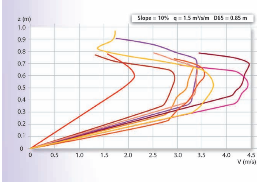
Example of velocity profiles on a rock chute made up of joined rocks ( D_{65} = 0.85 \text{ m} ) with a slope of 10%.
