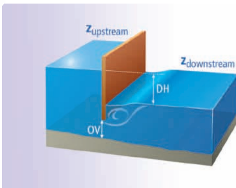
Parameters used to calculate a drowned gate flow.
