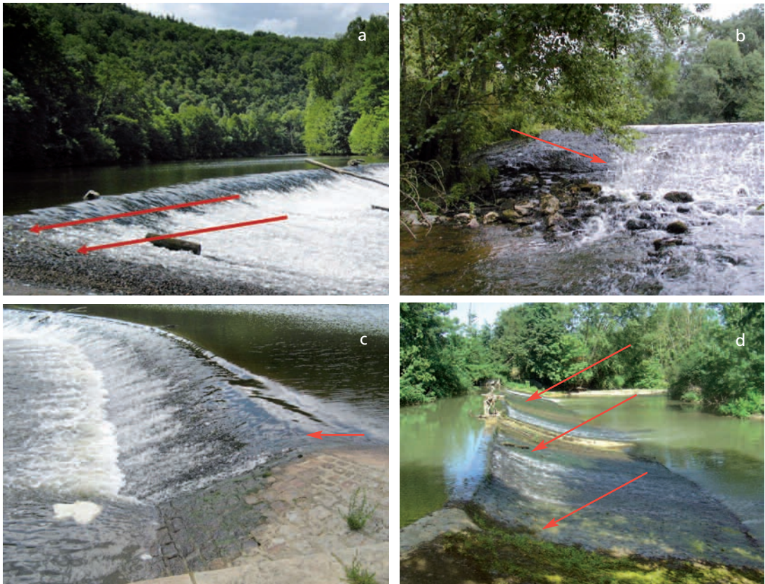
Examples of crawl ways.
