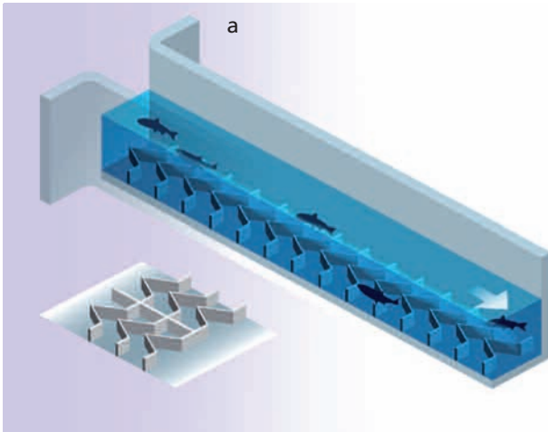
Diagram and example of fish passes with floor baffles. (a) Diagram, (b) fish pass with floor baffles at the Soustons dam.
