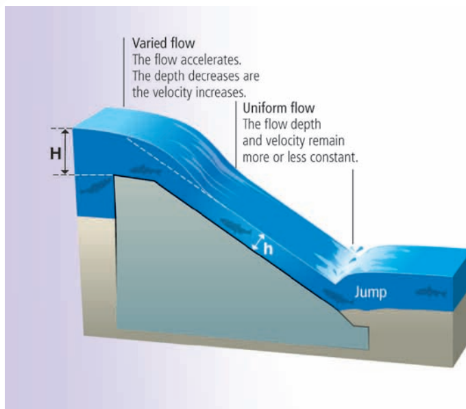
Changes in flow conditions along an inclined glacis.
