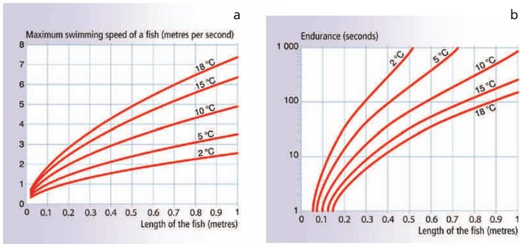
(a) Maximum swimming speed as a function of the size of the fish and the water temperature for salmonids, (b) endurance at maximum speed as a function of the size of the fish and the water temperature for salmonids. Adapted from Beach, 1984.
