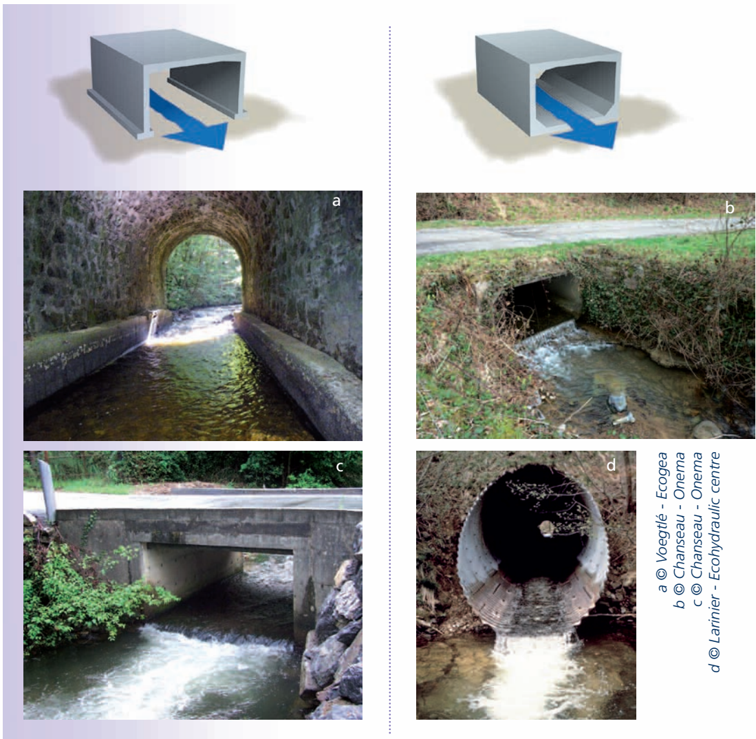
Diagrams and photos of open-bottom and closed-bottom structures. (a, c) Open-bottom passages, (b, d) closed-bottom passages.
