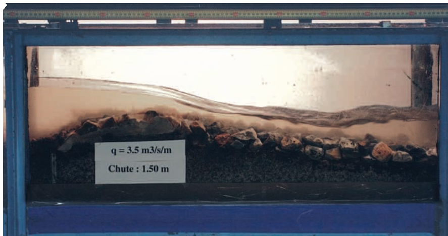
Flow over joined rocks with a slope of 10% (model to 1:22 scale).
