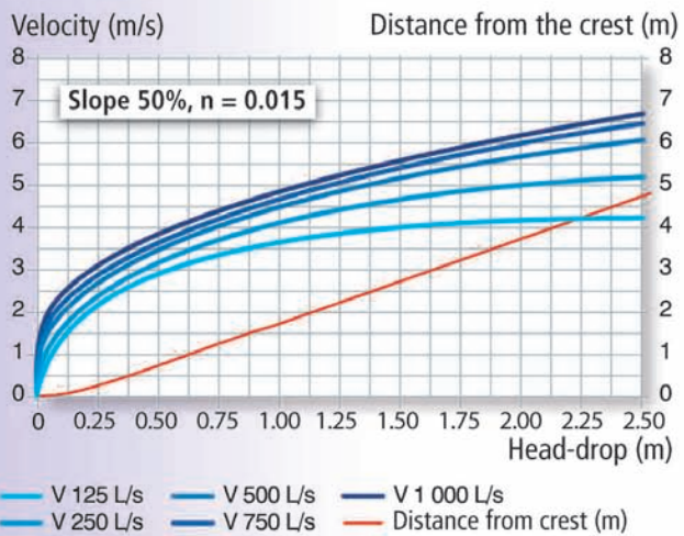
Graphs showing the relation between flow velocity, head-drop and distance from the weir crest as a function of the unit discharge (125 L/s/m to 1000 L/s/m), the slope (12%, 25% and 50%) and the roughness of the glacis surface (Manning n = 0.015 ).
