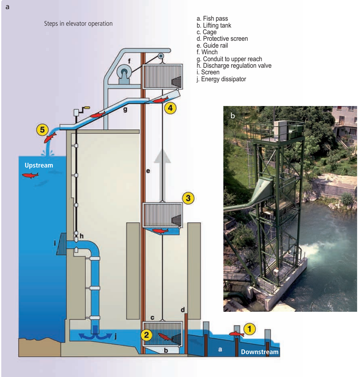
Diagram and example of a fish elevator. (a) Diagram of a fish elevator with a built-in lifting tank, (b) Castet elevator on the Ossau River.
