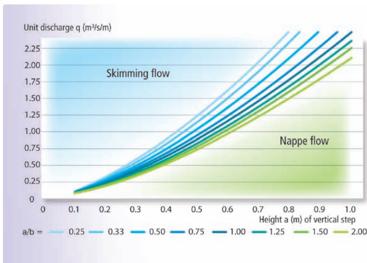
Transition between a nappe flow (with hydraulic jump) to a skimming flow as a function of the unit discharge and step characteristics.
