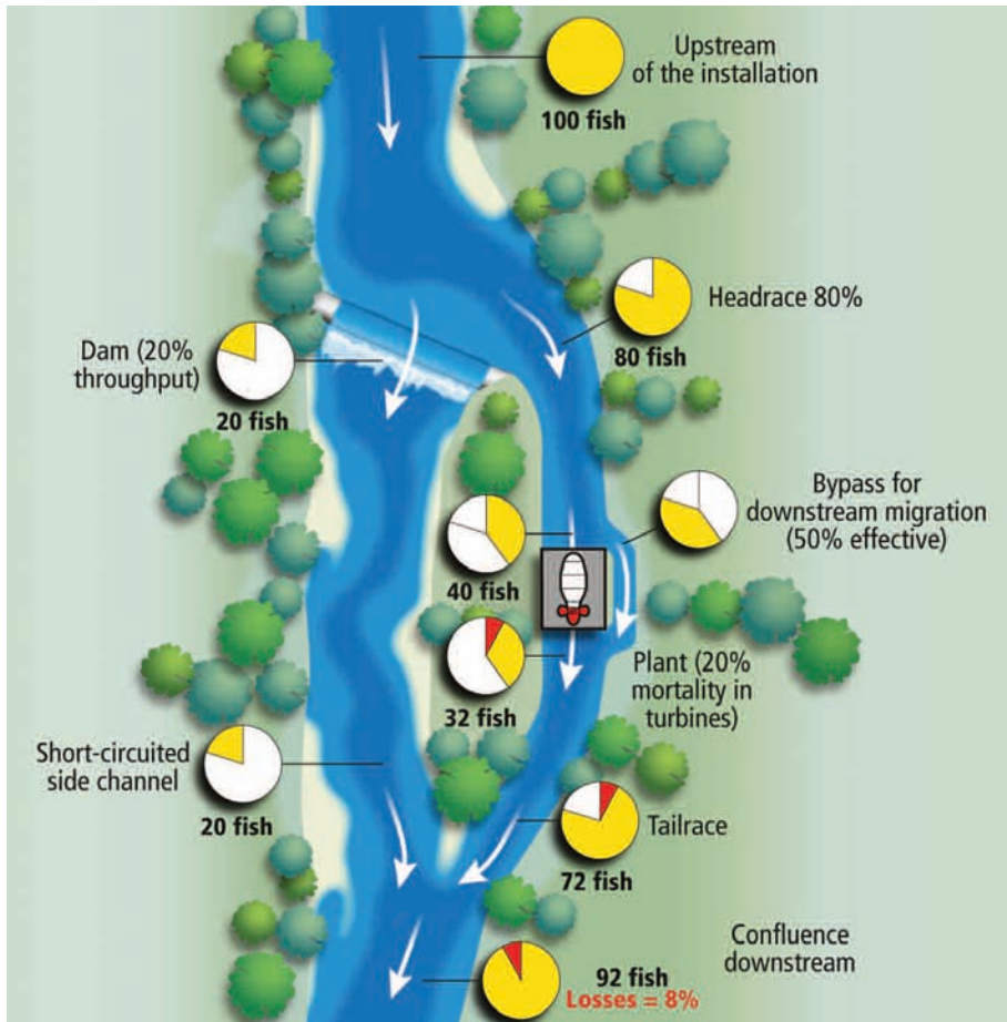
Diagram of a typical installation and basis for modelling the downstream migration. According to Voetgle and Larinier, 2004.
