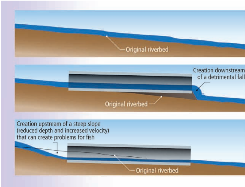
Examples of the problems created by poor longitudinal positioning of a structure.
