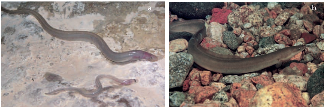
Examples of fish in Group eleven. (a) Glass eel and elver, (b) yellow eel.
