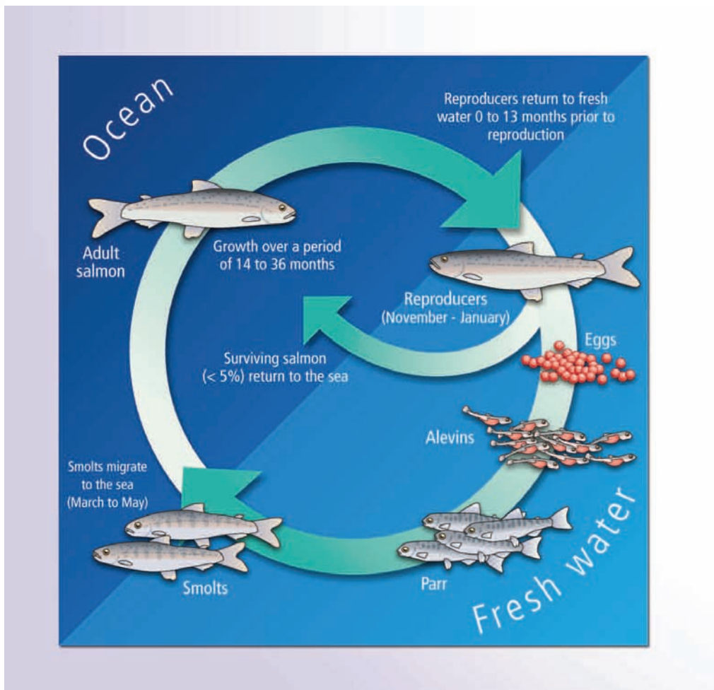
Migratory cycle of an anadromous, amphibiotic migratory species (Atlantic salmon).
