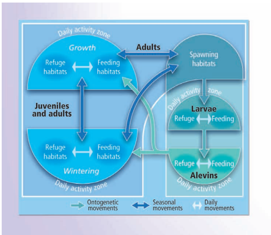
Diagram showing some of the many different movements undertaken by fish during their biological cycle. Drawn from Baras (1992).
