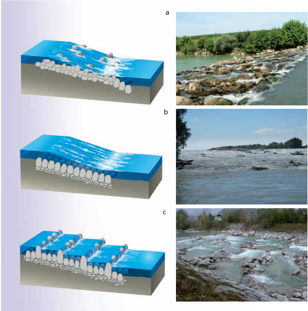
Examples of various rock-weir layouts.
