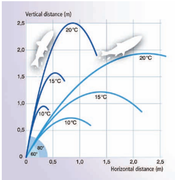
The theoretical trajectories of a salmon 0.8 metres long as a function of the water temperature and the angle of incidence of the jump. According to Larinier et al., 1998.
