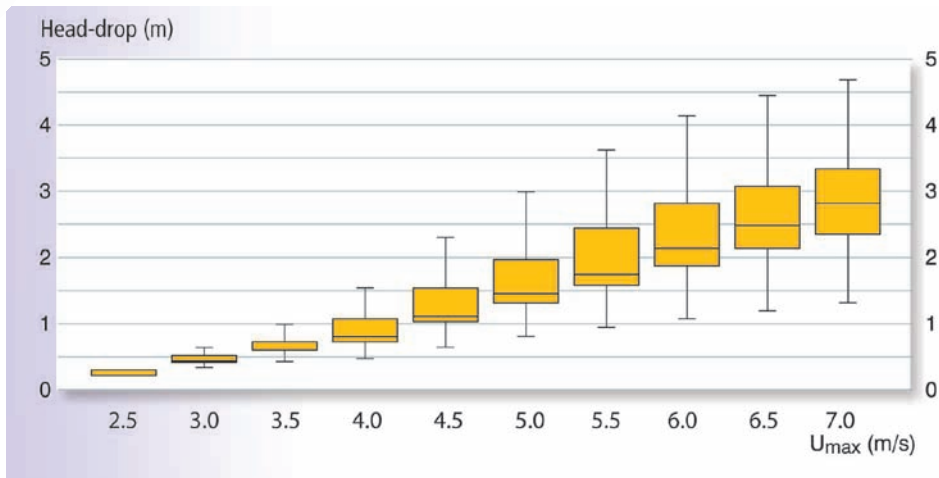
Passable head-drops as a function of the maximum swimming speed U_{max} (where the endurance is between 10 and 20 seconds), whatever the values of the other tested parameters (slope, unit discharge, roughness).
