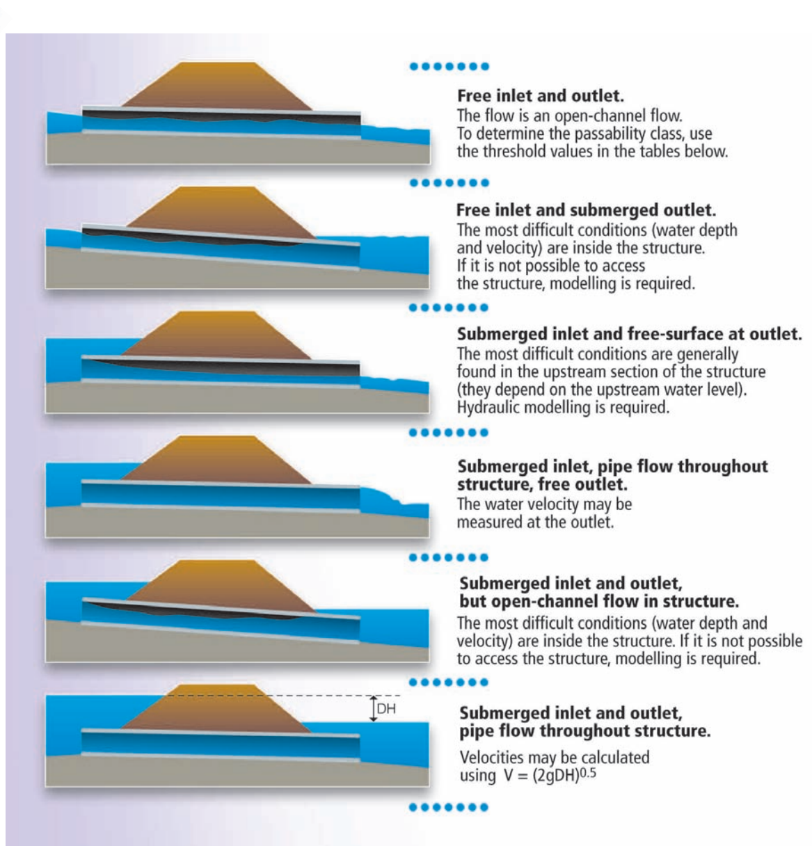
Various flow configurations in culverts.
