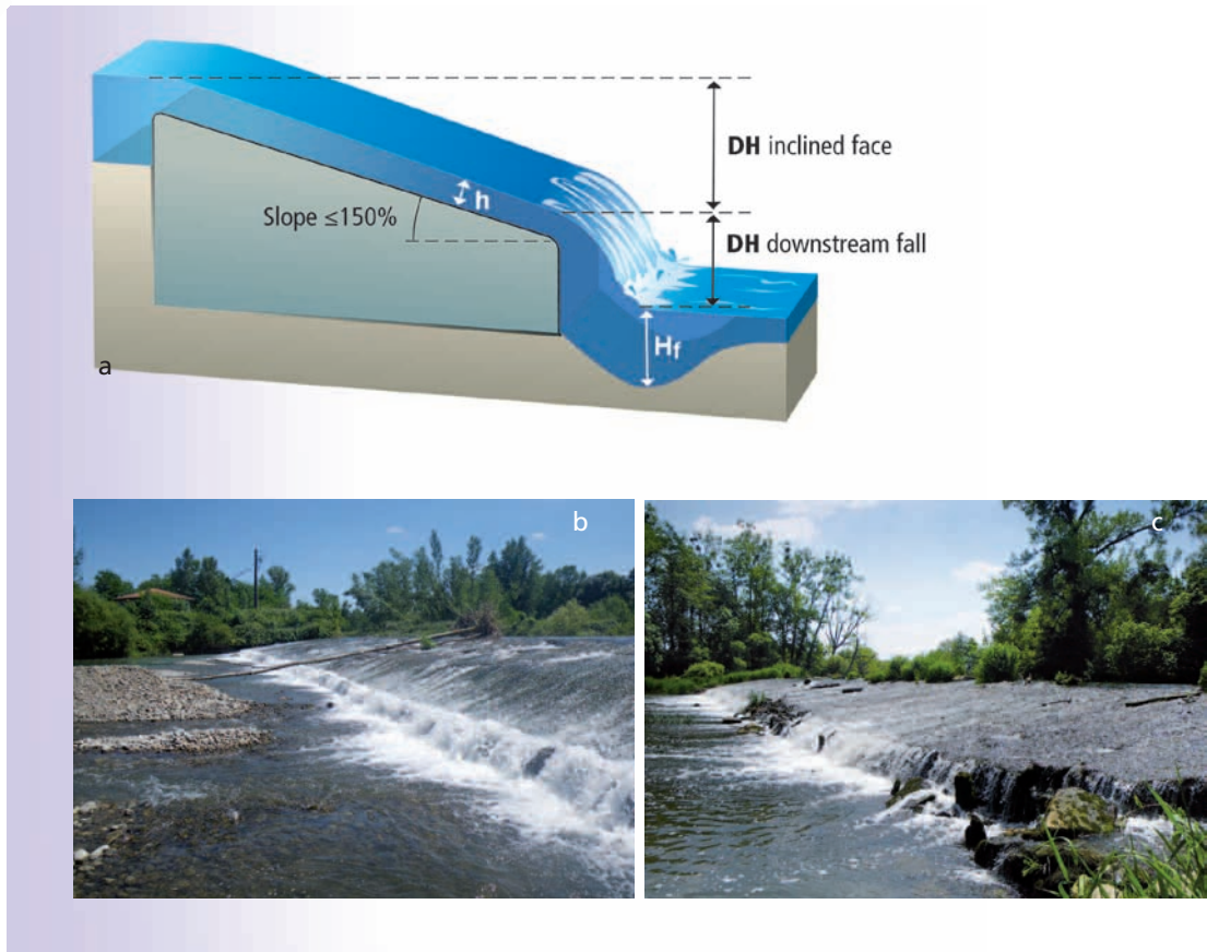
Examples of flows. (a) Diagram showing an inclined weir with a downstream fall, (b, c) flows over an inclined downstream face with a downstream fall.
