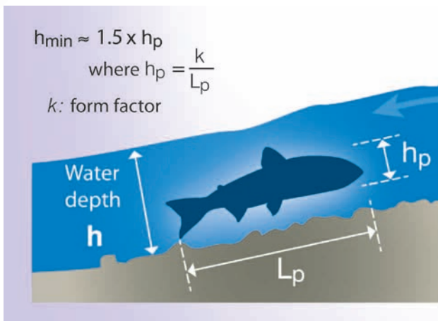
Diagram showing the water depth seen as the minimum required for fish to swim adequately.
