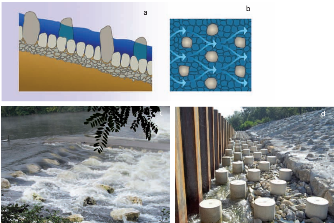
Diagrams and examples of rock chutes with staggered arrays of elements. (a) and (b) Diagrams of rock chutes with staggered arrays of elements, (c) rock chute at the Carennac weir on the Dordogne River, (d) fish pass at the weir for the ASF A7 highway over the Rubion River.
