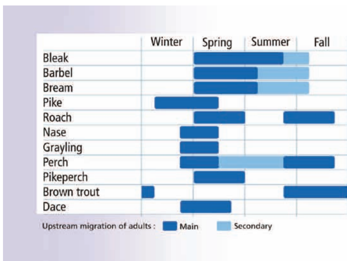
Main migratory periods of amphibiotic species and of adults in holobiotic species.
