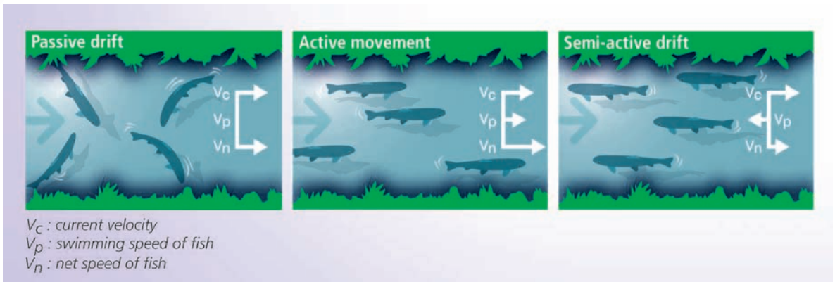
Types of downstream migration. Drawn from Sonny (2006), modified diagram drawn from Pavlov (1994).
