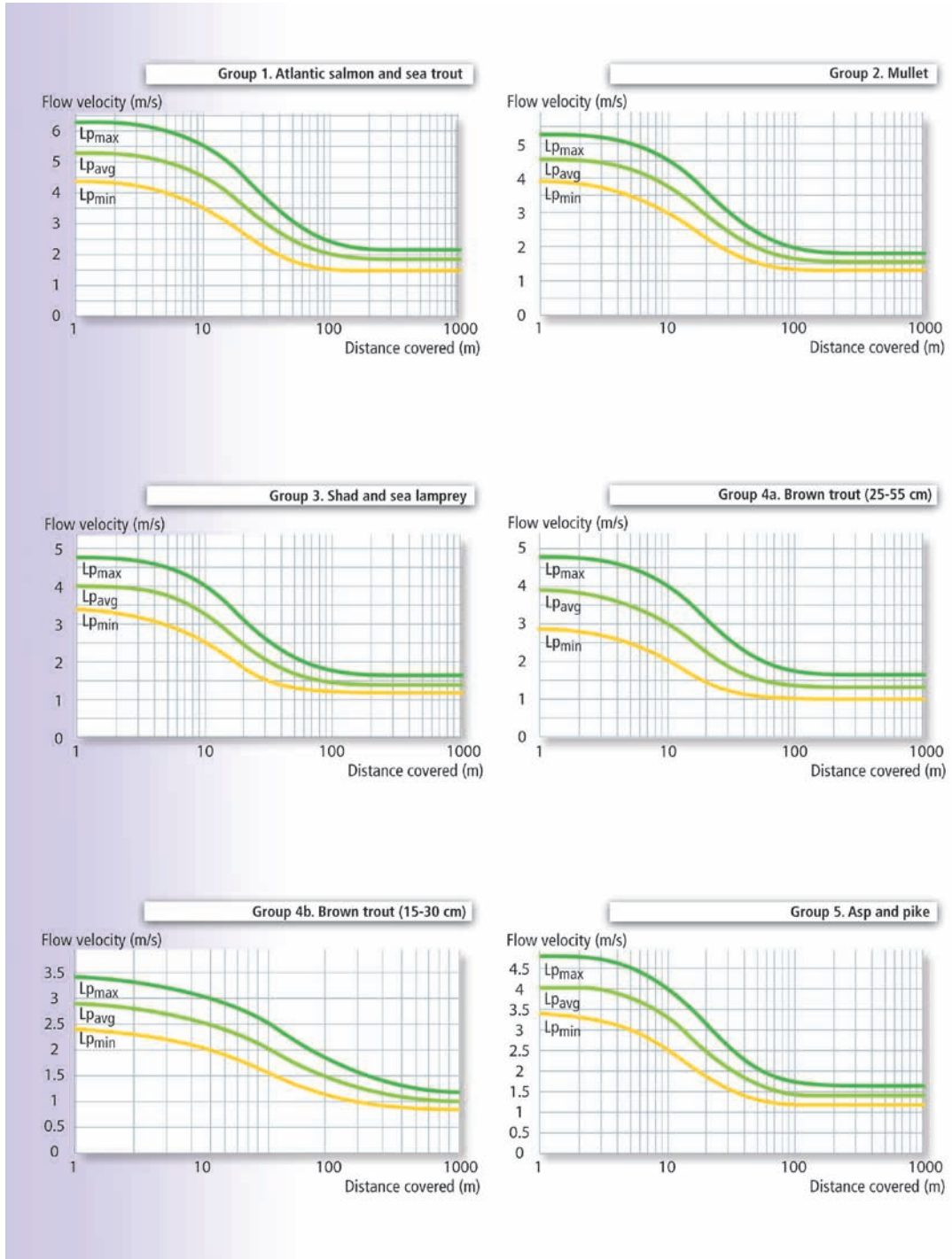
Distance covered as a function of the flow velocity for the species or groups of species number 1 to 5.
