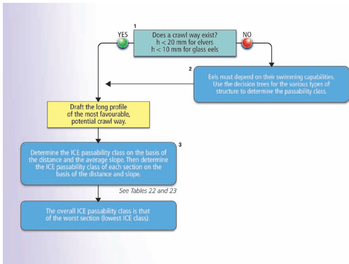
Decision tree to determine ICE passability classes for eels.
