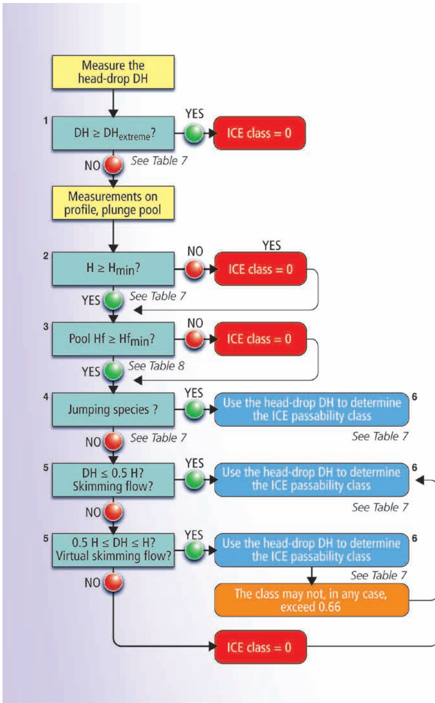
Decision tree to determine ICE passability classes for vertical and subvertical obstacles (slope >150% (56°)).
