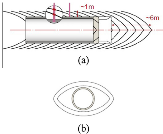
Fig. 9. Schematic representation of the fracturing pattern observed along a (a) vertical cross-section parallel to the gallery axis and (b) a cross-section perpendicular to the gallery axis [2].
