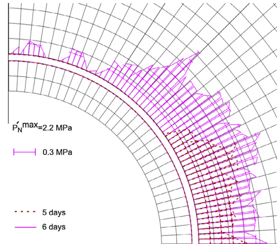
Fig. 14. Diagram of the normal contact pressure on the interface.
