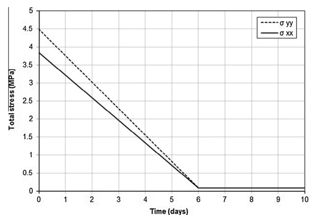
Fig. 5. Imposed total stresses on the gallery wall.
