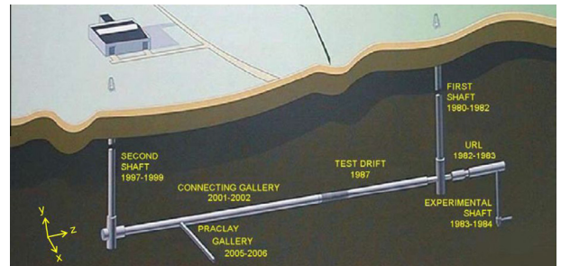
Fig. 3. Sketch of different galleries in HADES for studying the high-level nuclear waste disposal in Boom clay [31].
