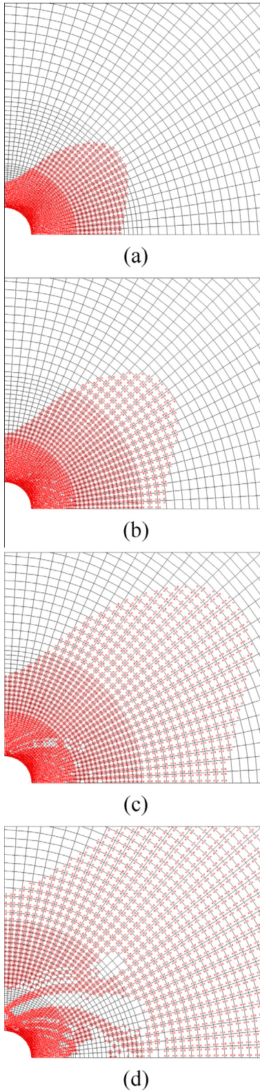
Fig. 13. Plastic loading index around the gallery without the concrete lining after (a) 4 days, (b) 5 days, (c) 6 days, and (d) 3.5 years.
