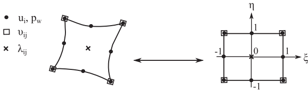
Fig. 1. 2D second gradient finite element: quadrilateral element (left), corresponding parent element (right).
