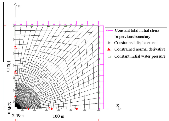
Fig. 4. Geometry of the model.
