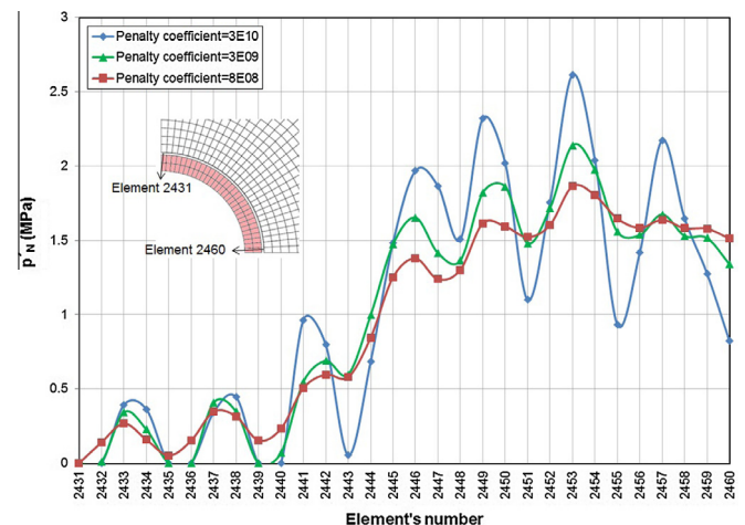
Fig. 17. The influence of penalty coefficient on development of the normal contact pressure on the interface.
