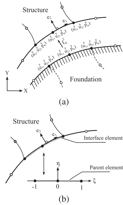
Fig. 2. 2D parabolic interface element (a) discretization description; ($e_1, e_2$) are the local current basis and (b) interface element and corresponding parent element.
