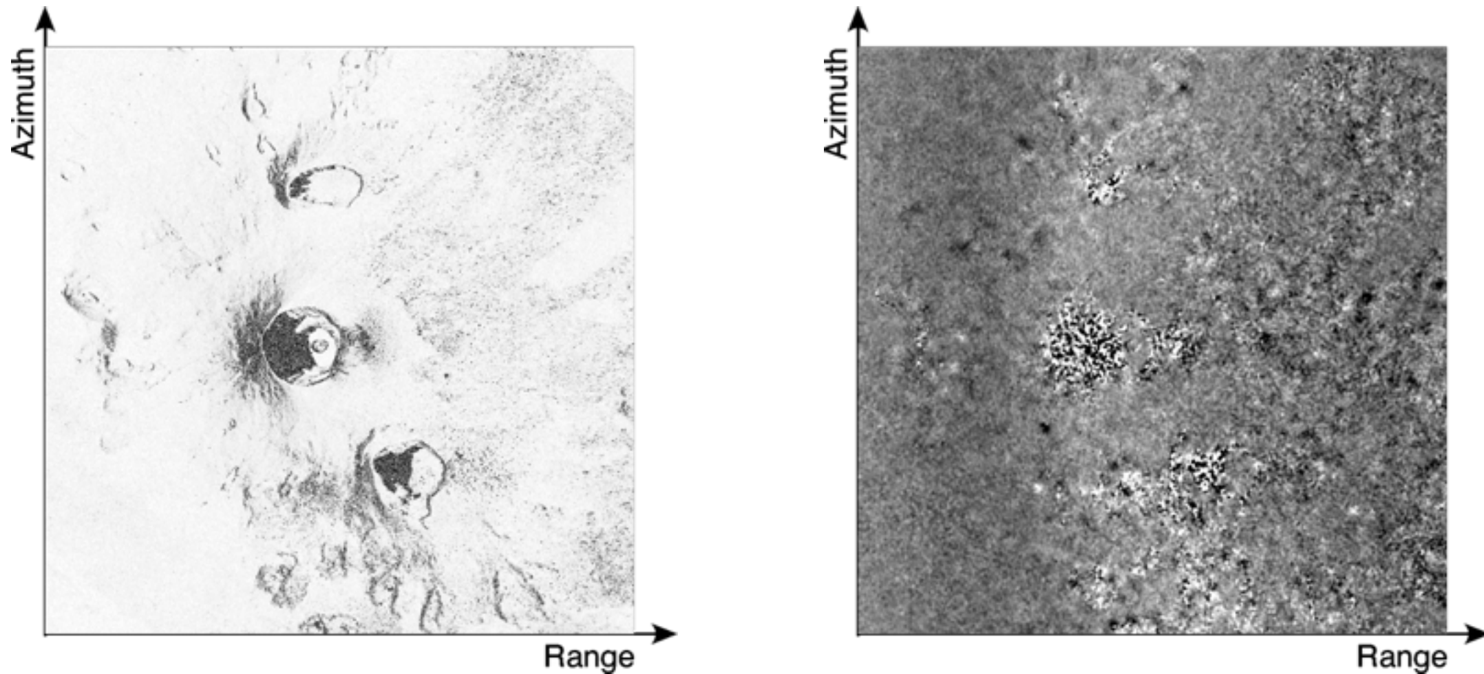
Left: Spectral coherence – Right: Correcting phase term
